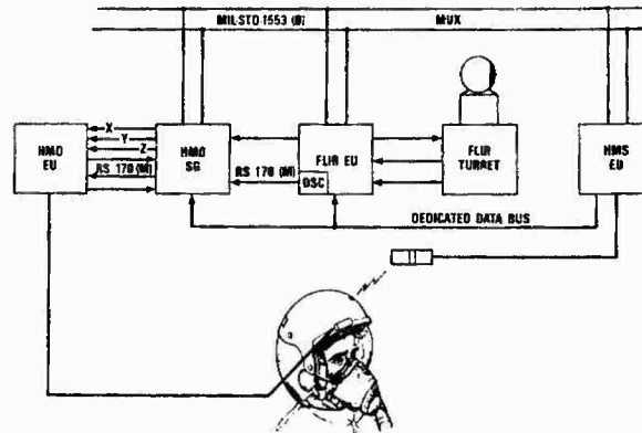
Figure 8. Electronic System Architecture
