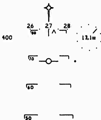
Fig 5. The Basic Fast-Jet HUD Format (FJF) showing a high nose-up CDA.
