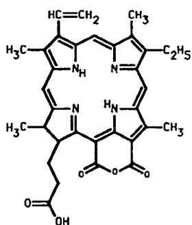
11 purpurin 18
