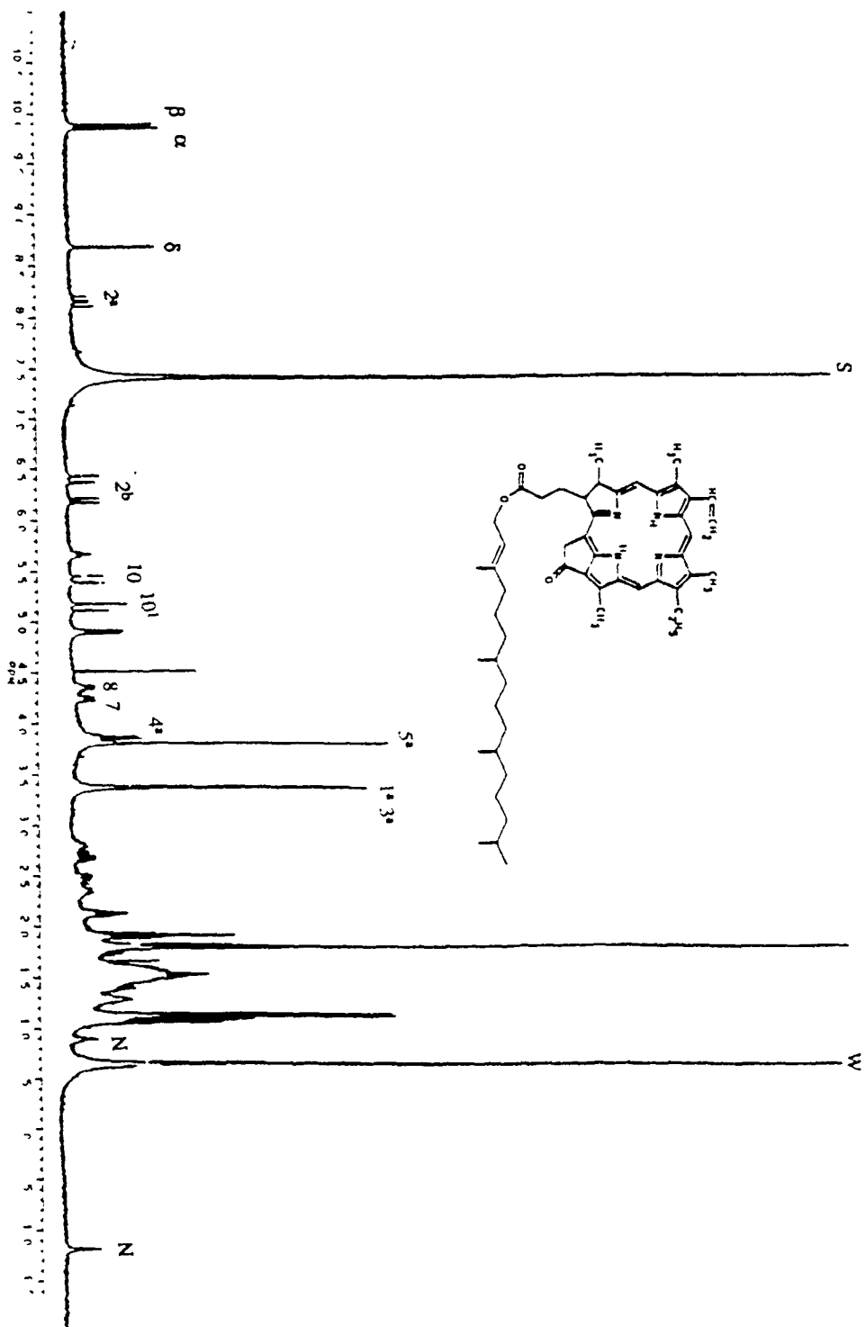
Fig. 2-4 300 MHz proton NMR spectrum of pyropheophytin- a in d 6 -benzene.
