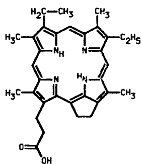
7 acid of deoxophylloerythroetioporphyrin
