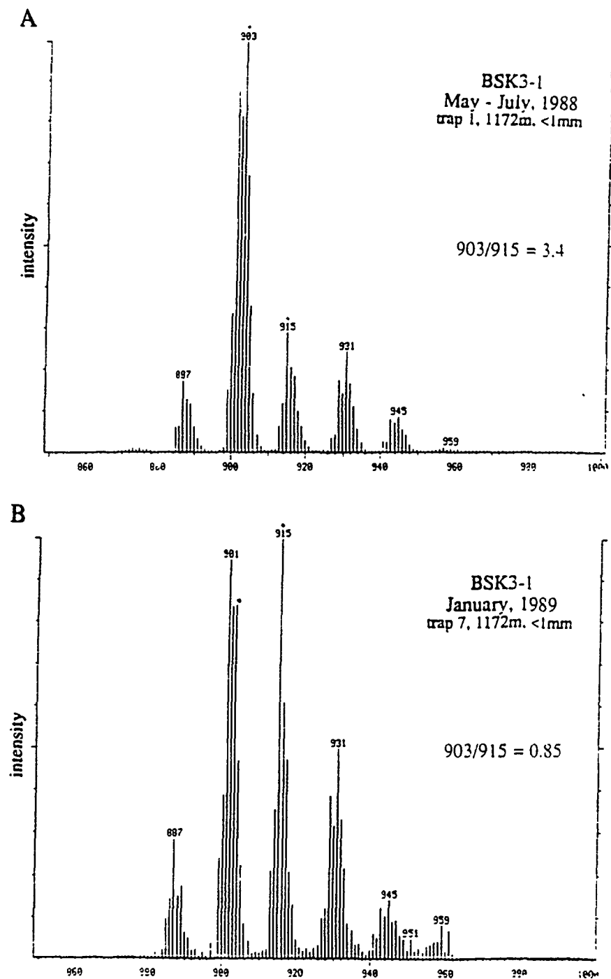
Fig. 5-5 Chemical ionization-MS of total PSE isolates from the May - July, 1988, and January, 1989 sediment trap samples from station BSK3-1.
