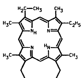
10 10-oxypeophorbide
