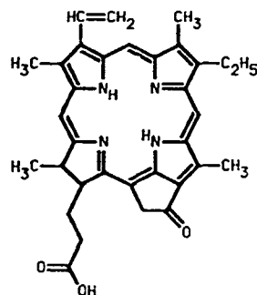
4 pyropheophorbide-a
