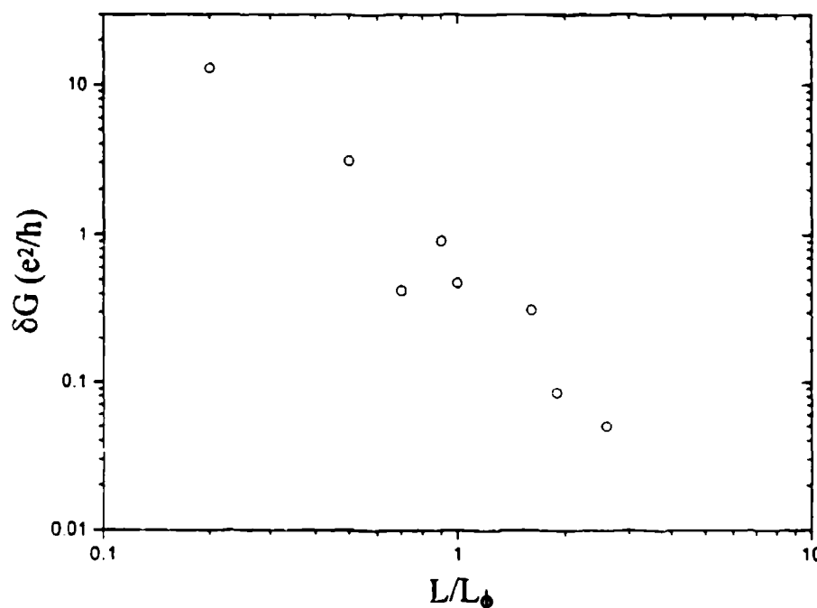
FIGURE 7. RMS magnitude of the conductance fluctuations as a function of normalized line length (where L_\phi is the phase breaking length taken as 1 \mu m ).
