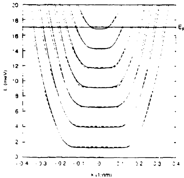
Fig. 2: The energy-dispersion relations for the hybrid magnetoelectric subbands in a 2000 Å wide structure at a magnetic flux density of 1.5 Tesla. The solid curves are the result of an exact numerical calculation and the broken curves are those obtained from the application of Bohr-Sommerfeld quantization rule.
