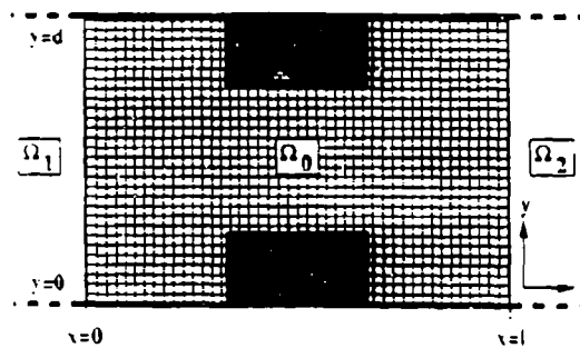
FIGURE 1. Schematic of the channel geometry showing the finite element domain, \Omega , and the leads, \Omega_1 and \Omega_2 . The shaded regions represent the confining gate potentials.
