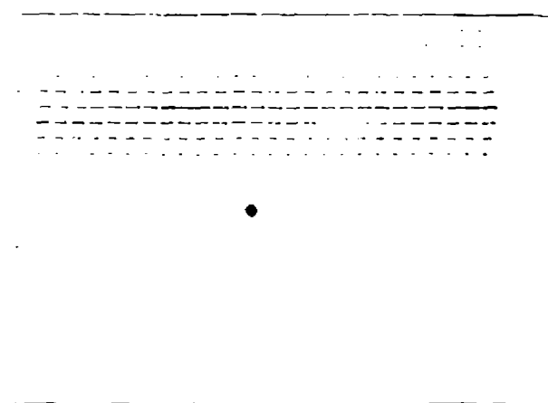
• Fig. 4: The spatial distribution of the current density J_{\text{tot}}(x, y) in the structure of Fig. 3(a) when a magnetic flux density of 2.18 Tesla is applied. The current flows along the top edge indicative of the formation of "edge states". This situation corresponds to the onset of the integer quantum Hall effect.
