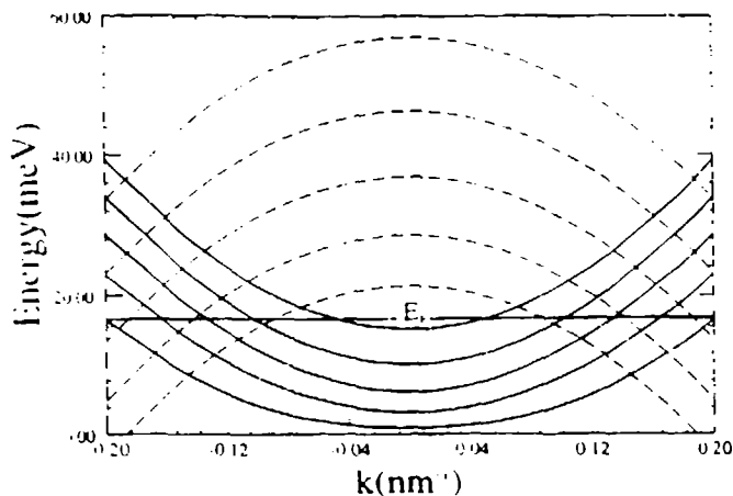
FIG. 2. Energy dispersion E vs k_x of magneto-electric subbands in a waveguide subjected to a magnetic field. The waveguide transverse width is 100 Å and the magnetic field is 1 T. The Fermi energy is taken to be 17 meV. If the subband bottoms are below the Fermi energy, the states are propagating states and have real wave vectors; otherwise they are evanescent states and have imaginary or complex wave vectors. For the parameters (well width and magnetic field) chosen, the lowest evanescent states have purely imaginary wave vectors. The evanescent states are shown with negative curvatures. The energy separation between the subband bottoms depends on the magnetic field as well as the width of the waveguide.
