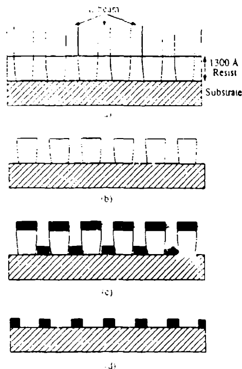
Fig. 1. Explanation of the lift-off process. (a) Exposure of resist by electron beam before development, resulting in slight undercutting. (b) Resist wall profile after development. (c) Resist walls after metalization from small, perpendicular source. (d) Metal pattern after dissolution of remaining resist in suitable solvent.
