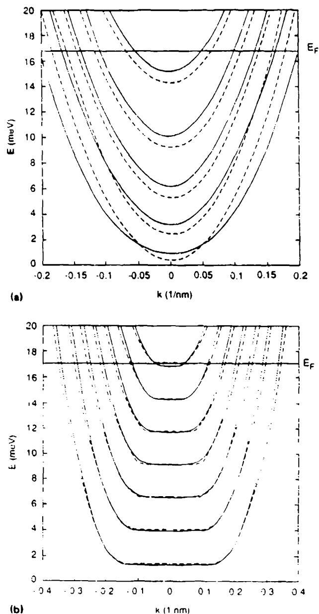
FIG. 3. Energy dispersion relations (for the propagating states only) obtained from our results (solid curves) and the Bohr-Sommerfeld quantization rule (broken curves). (a) The waveguide width is 1000 Å and the magnetic field is 1 T; (b) the waveguide width is 2000 Å and the magnetic field is 1.5 T.
