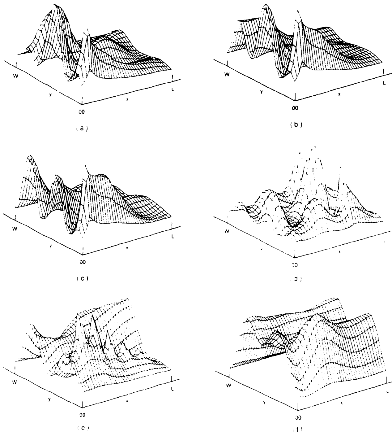
FIG. 6. Two-dimensional profile of the concentration of Fermi carriers. (a)-(f) correspond to the parameters and conditions of Figs. 5(a)-5(f).
