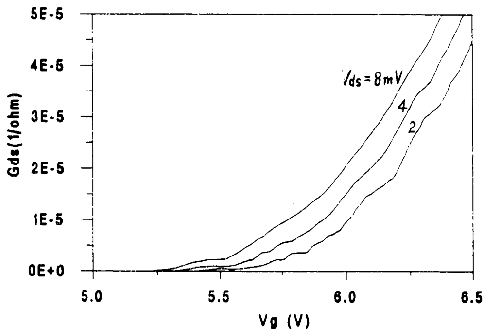
FIGURE 13. Structure in the drain conductance, g_d , between source and drain of an 8 \mu\text{m} long MOSFET at 1.83 K as a function of gate voltage, V_g . The 1-D channel was created by EBL exposure and resulting positive oxide charge creating a potential well at the interface.
