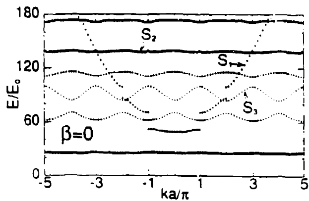
FIGURE 2. Shown is the bandstructure when \beta = 0 in extended zone scheme.
