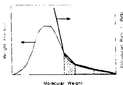
FIG. 9. Solubility curve for a conceptualized "ideal" developer superimposed on the distribution of fragment molecular weights for PMMA. The shape of the solubility curve ensures that dissolution rates for each molecular weight are no higher than necessary to dissolve all molecular weight fractions completely, thereby minimizing erosion of areas adjoining those of primary exposure.
