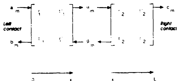
FIG. 3. A structure is decomposed into two sections with a common boundary at the coordinate x . The wave amplitudes at x are related to the wave amplitudes at the left and right contacts through the two scattering matrices describing the two sections.
