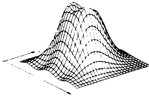
• Fig. 8. The spatial distribution of \delta n(x, y) at a magnetic flux density of 3.5 Tesla when a magnetic bound state forms.
