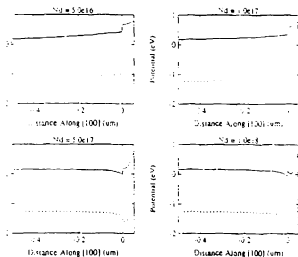
FIG. 2. Band diagrams on the n side of the lateral p - n junction for several doping concentrations. The solid line represents the conduction band, the dashed line the valence band, and the dotted line the Fermi level.
