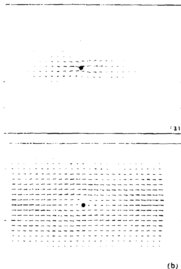
• Fig. 3: The spatial distribution of the current density J_{\text{tot}}(x, y) in a 800 Å long and 1000 Å wide structure in the absence of any magnetic field. The Fermi energy is 2.054 meV. (a), Current crowding around an attractive impurity, (b), current detour around a repulsive impurity.
