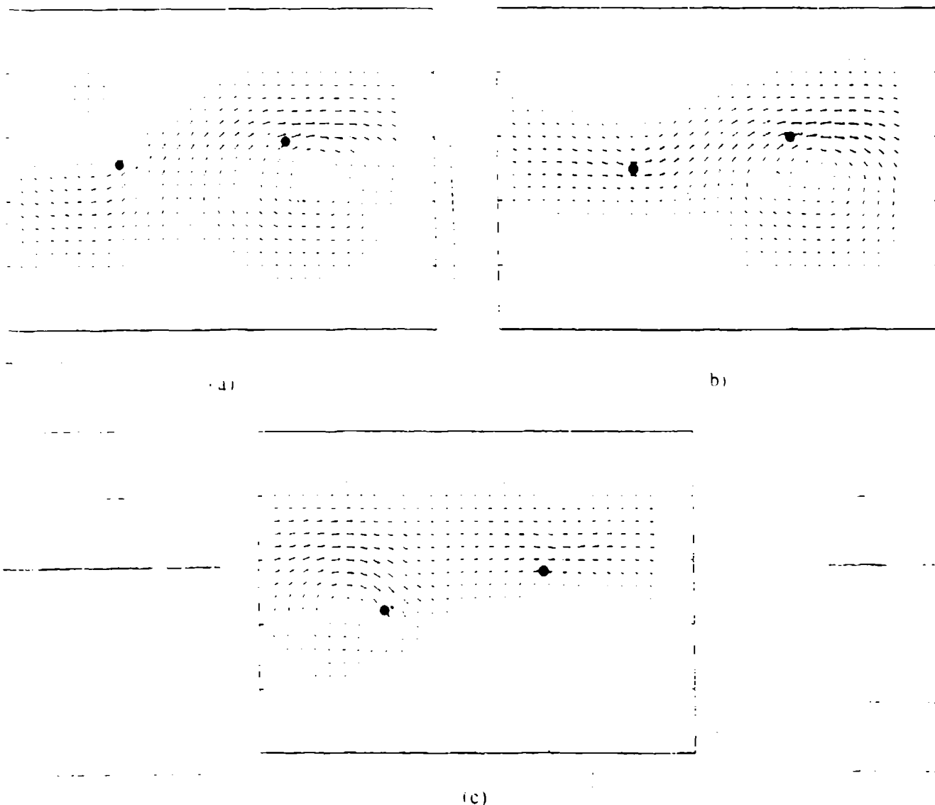
FIG. 9. The spatial distributions for a 900-Å-long and 1000-Å-wide structure containing multiple impurities. (a) The current profile in zero magnetic field showing the formation of two strong vortices due to quantum interference between the scatterers and (b) the current profile in a magnetic field of 0.08 T. (c) Complete change
