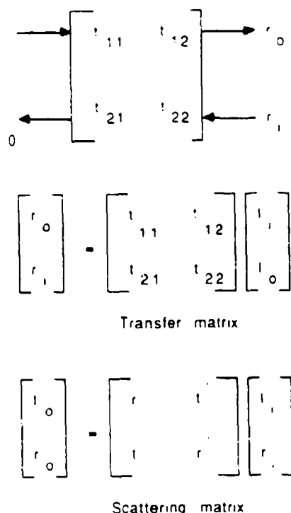
FIG. 2. Incident and reflected waves at any arbitrary section of the structure. The relationships between the waves are expressed through the transfer matrix [Eq. (10)] and the scattering matrix [Eq. (12)].
