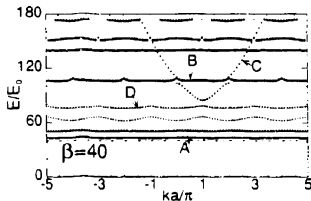
FIGURE 4. Shown is the bandstructure when \beta = 40 in extended zone scheme.
