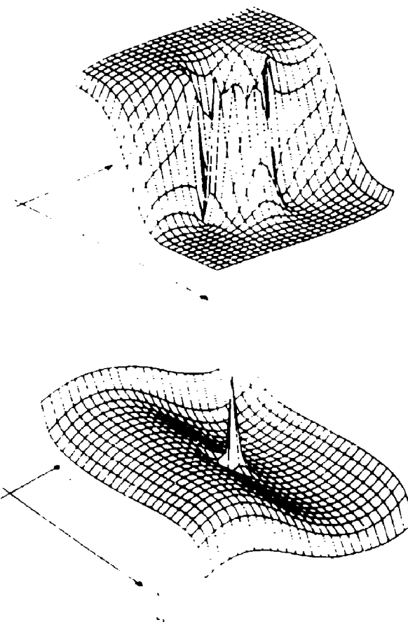
• Fig. 9. The spatial distribution of the chemical potential in the absence of any magnetic field. (a), the scatterer is attractive (corresponding in the case of Fig. 3(a)), (b), the scatterer is repulsive (corresponding to the case of Fig. 3(b)). Note that in the first case, most of the potential drop occurs around the impurity which is the dominant cause of resistance. In the second case, the potential is dropped more at the contacts showing that the contact resistances are dominant over the residual resistance of the impurity. This is a major difference between attractive and repulsive scatterers.
