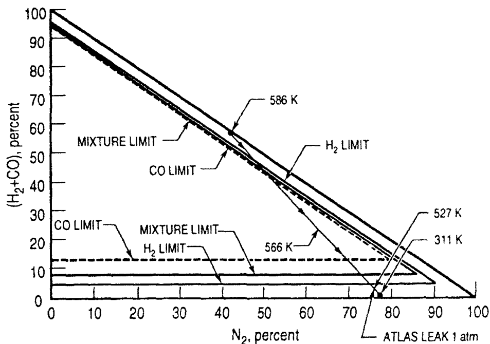
Figure 15. Flammability limits of \text{H}_2 -CO mixture-- \text{H}_2\text{CO} = 25:32 , 298 K, 1 atm. Trajectory shows Atlas leak at 1 atm.
