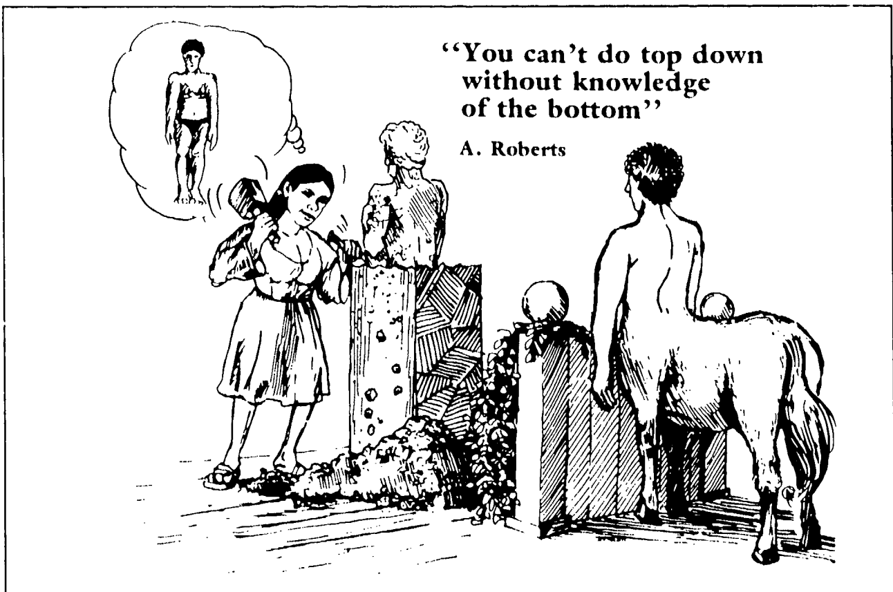
Fig. 13-6 Top-Down Design
