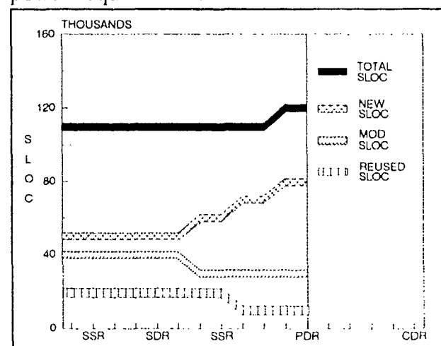
Fig. 12-1 Software Size
