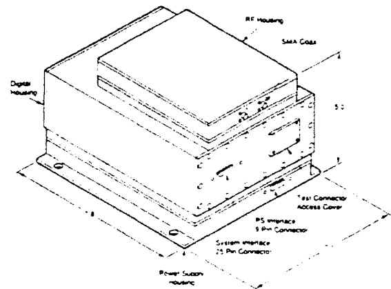
Figure 1. Miniature GPS Receiver
