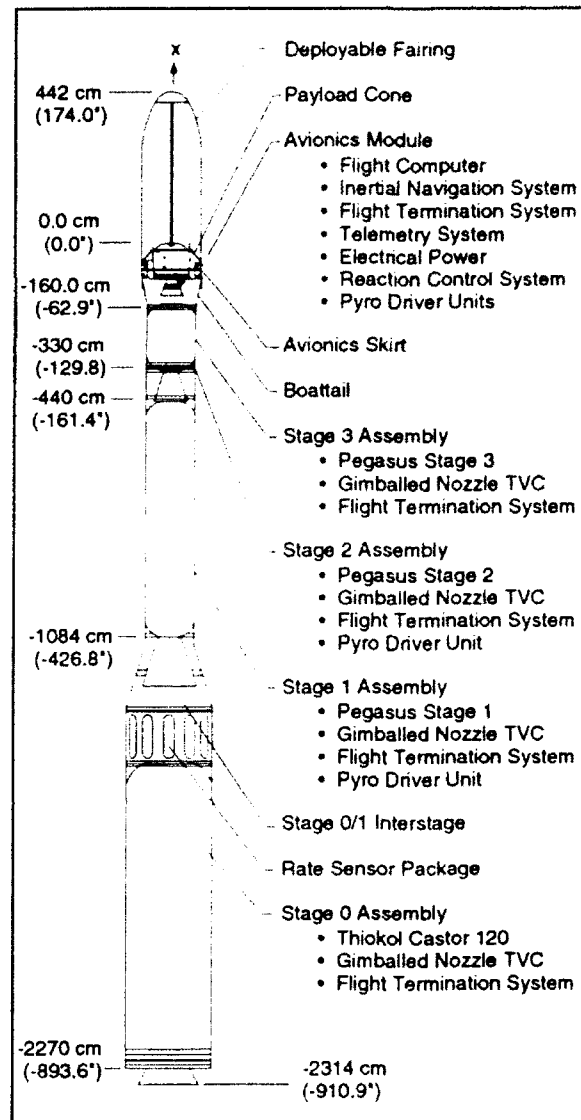
Figure 8. Taurus subsystems.
