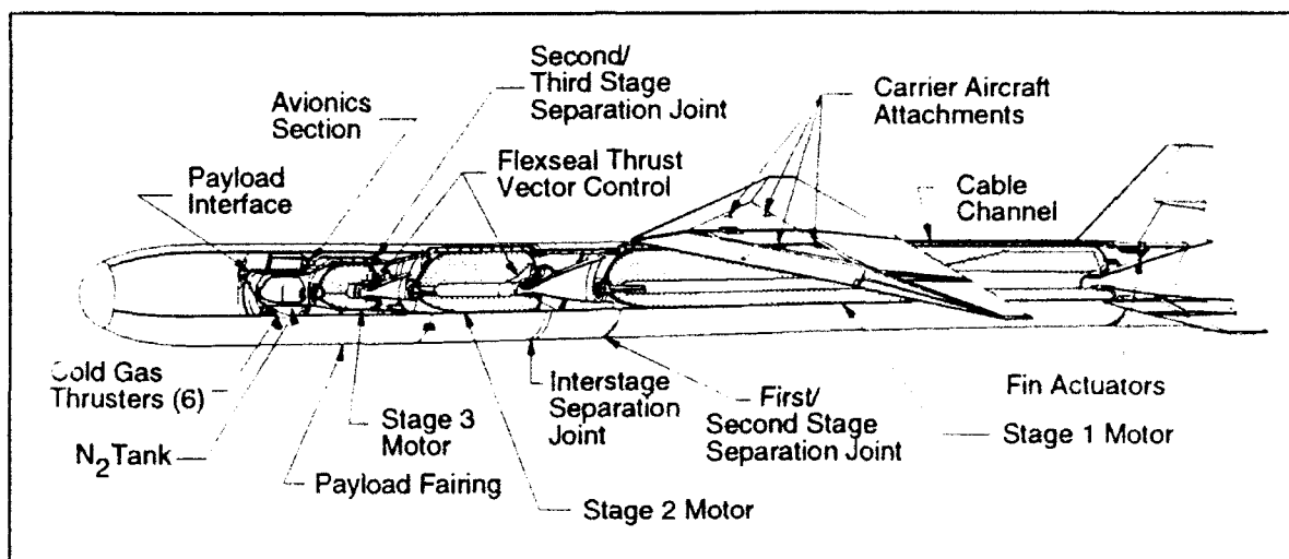
Figure 3. Pegasus cutaway.
