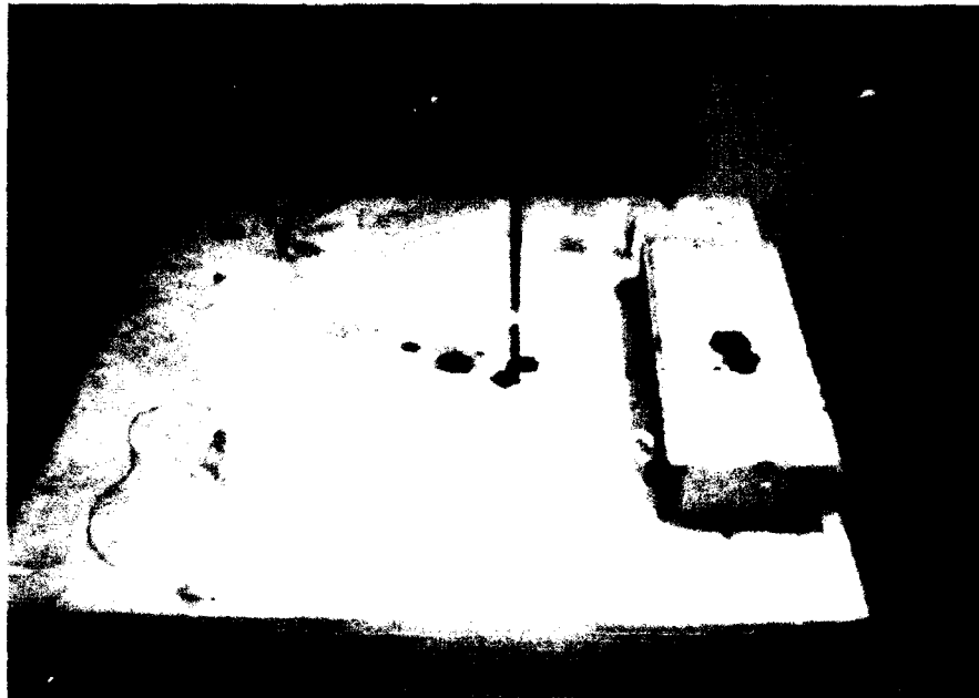
Figure 37. PZT piezoelectric element bonded to end of 7-ft steel rod used to make pulse-echo measurements on concrete slab. Analogous to function of a Hopkinson Bar
