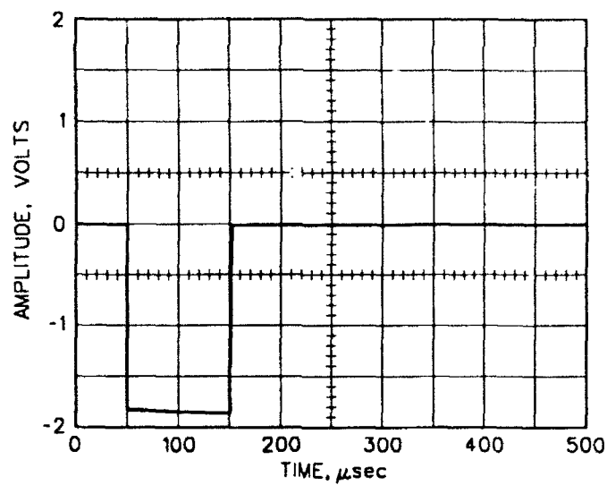
Figure 20. Rectangular shaped electrical pulse from a pulse generator (similar to shape of mechanical load-pulse from Schmidt hammer)
