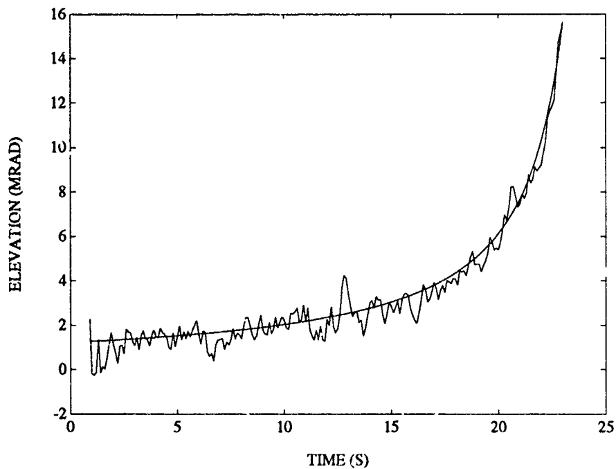
FIGURE D-31. SAMPLE ELEVATION ESTIMATE FOR 3 STATE FILTER ON S-TURN TARGET
