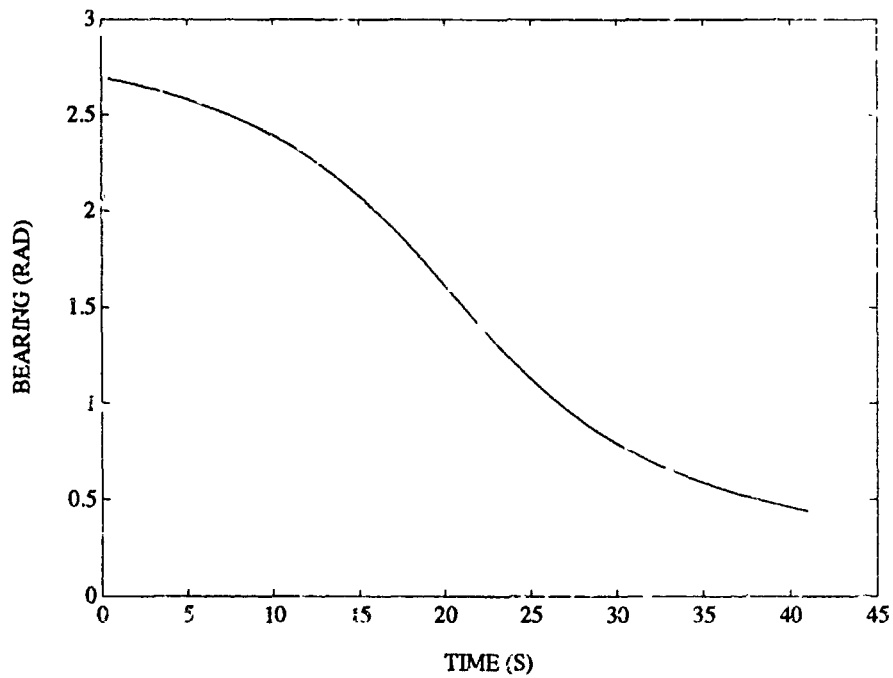
FIGURE C-15. SAMPLE BEARING ESTIMATE FOR 2 STATE FILTER ON CROSSING TARGET
