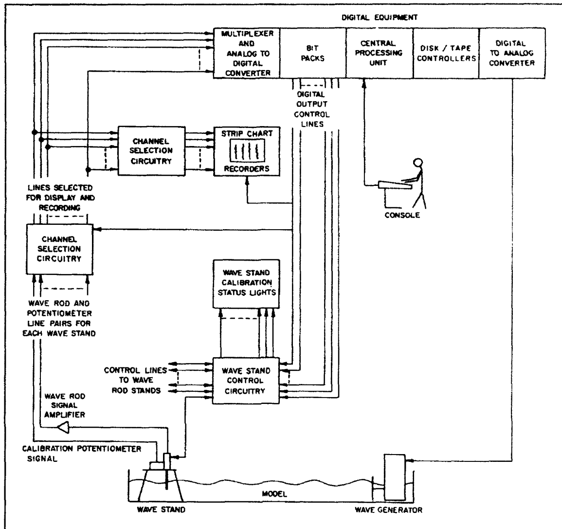
Figure 6. Automated Data Acquisition and Control System
