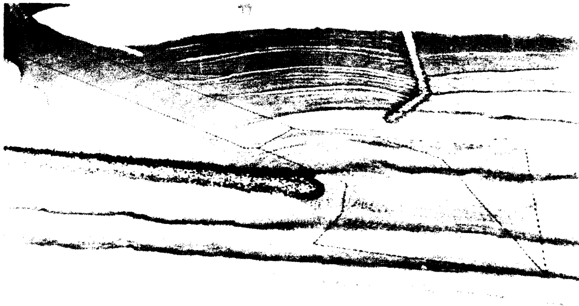
Photo 11. Typical wave patterns for Plan 1: 17-sec. 16-ft monochromatic waves from 275 deg; swl = 0.0 ft
