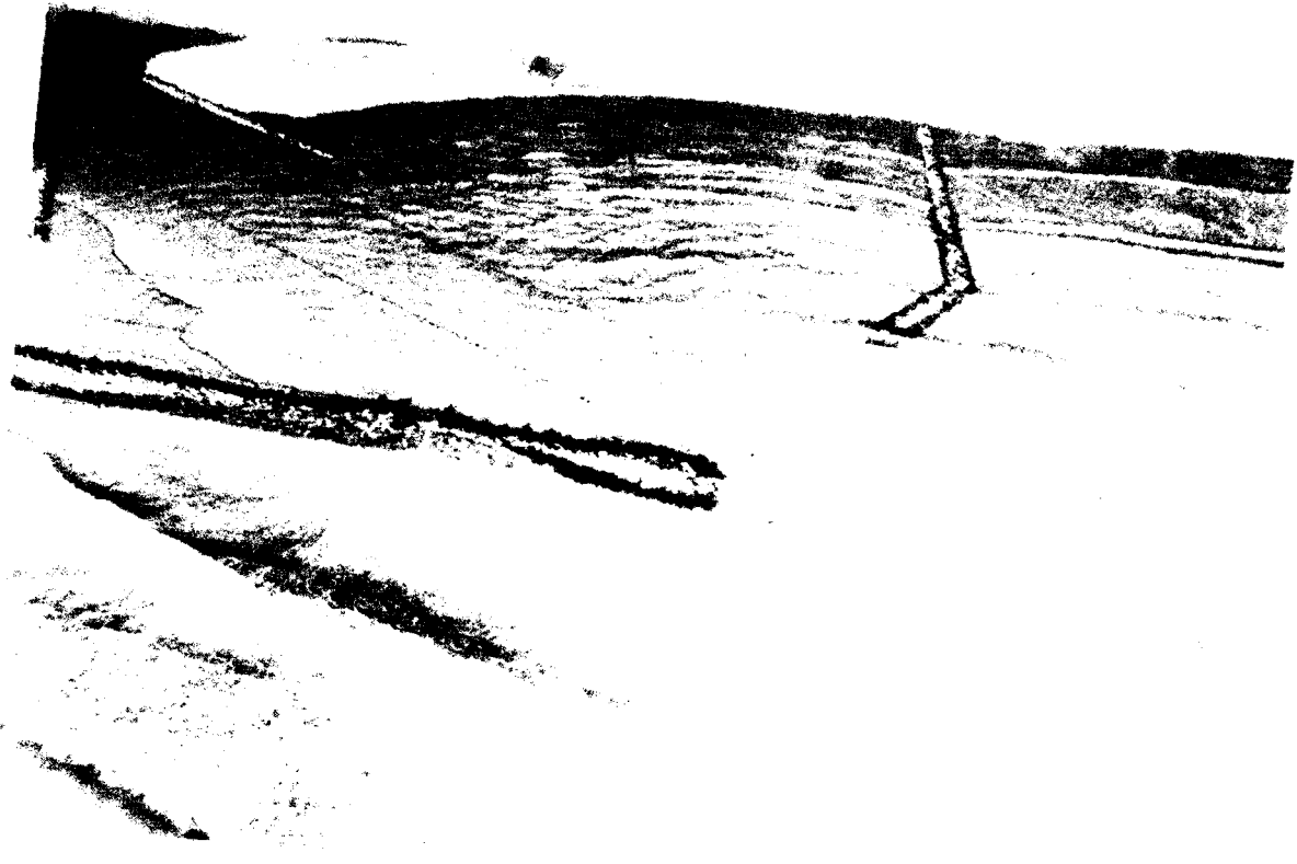
Photo 45. Typical wave patterns for Plan 15; 15-sec. 21-ft spectral waves from 300 deg; swl = +7.0 ft
