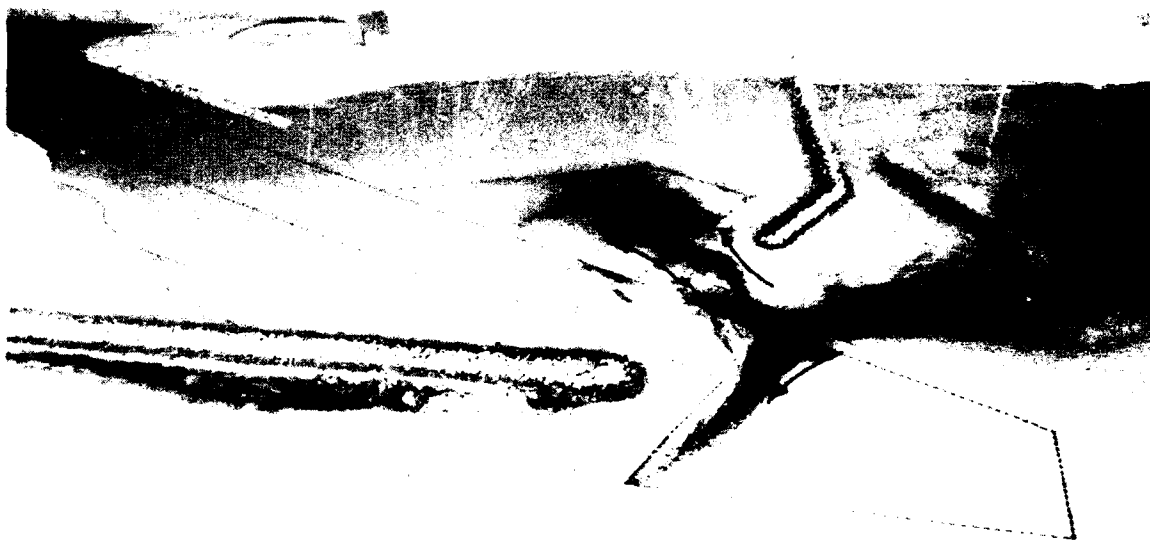
Photo 61. General movement of tracer material and subsequent deposits for Plan 14 for 15-sec, 12-ft monochromatic waves from 250 deg; swl = 0.0 ft
