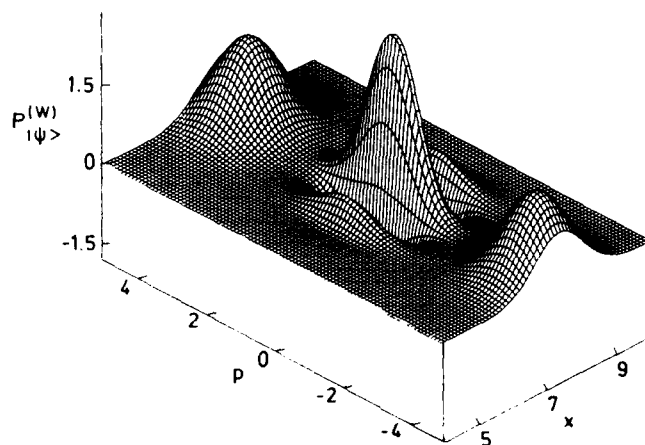
Figure 6: The Wigner function, P_{|\psi\rangle}^{(W)} , of the quantum mechanical superposition of two coherent states does not consist of only two Gaussian bells located in x - p oscillator phase space at x = \sqrt{2} \alpha \cos \varphi/2 and p = \pm \sqrt{2} \alpha \sin \varphi/2 corresponding to two individual coherent states |\alpha e^{i\varphi/2}\rangle and |\alpha e^{-i\varphi/2}\rangle but involves an interference term located on the x -axis. This contribution originates from the quantum mechanical superposition of the two coherent states and the bilinearity of the Wigner distribution, Eq. (2), in the wave function. This interference hill can be narrower in the x -direction than the individual Gaussian bells giving rise to squeezing in the x -variable (Fig. 5a); or it can even take on negative values to create an oscillatory photon count probability, W_m , Fig. 4d. (Here we have chosen \alpha^2 = 36 and \varphi = \pi/3 .)
