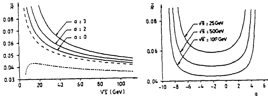
Fig. 3.1 The energy dependence of \tilde{R} for a = 0.2 and 3 in AMOM scheme. The dashed line represents \tilde{R} in \overline{\text{MS}} scheme.
