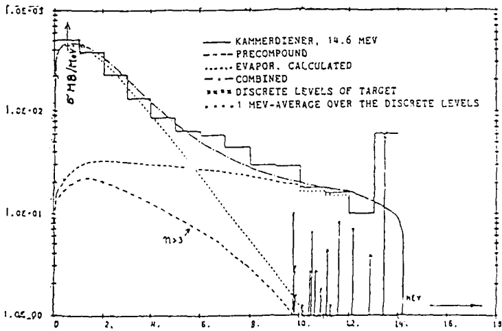
Fig. 3: Neutron emission cross-section of ^{56}\text{Fe} ; \epsilon_i = 14,6 \text{ MeV}
