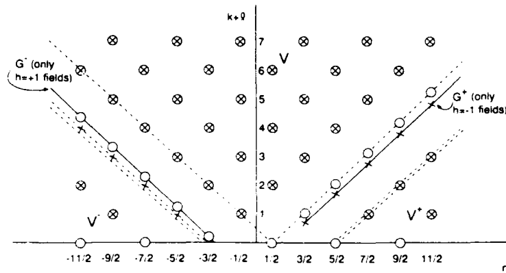
FIGURE 1. WEIGHT DIAGRAM FOR FRONT-HALF SPANNORS. Each circle or cross represents two K types, namely b(n, k + \ell, h)^+ and b(n, k + \ell, h)^- . Circles denote h = +1 fields and crosses denote h = -1 fields. Points to the right of and along the dashed half-line in the first quadrant represent V^-[V^+] . Points above and along the dashed half-lines represent V^-[V^+] . Points to the left of and along the dashed double half-line in the second quadrant represent V^+[V^-] . Points along the solid half-lines represent G^-[G^+] and G^+[G^-] . They have been slightly displaced in order to make clear their disjointness from V^-[V^+] and V^+[V^-] .
