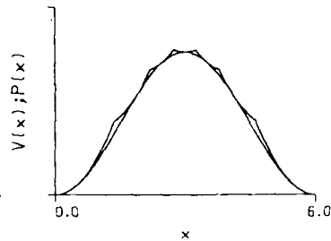
Fig.2: Parabolic contact transformation: A potential V(x) and the corresponding approximating 6-parabola potential P(x) .
