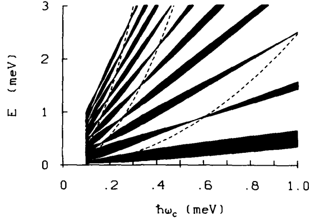
Figure 2: Sketch of the modulation-broadened Landau fan diagram, calculated from Eq. (5) with V_x = 0.2\text{meV} and 2\pi/K = 200\text{nm} . Allowed energy regions in the Landau bands with n = 0, 1, \dots, 9 are shown black. The flat band energies, \varepsilon_\lambda for \lambda = 1, 2, 3 , are indicated by dashed lines.
