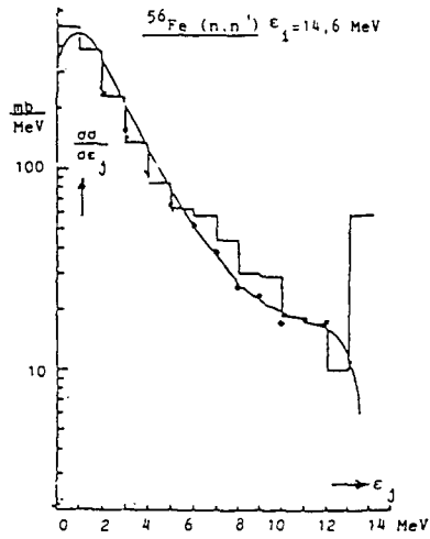
Fig. 1: Stepcurve and GDH-curve of the secondary energy dependent total inelastic scattering cross section of 14,6 MeV neutrons on ^{56}\text{Fe} . Points: Dresden Measurements, /2/
