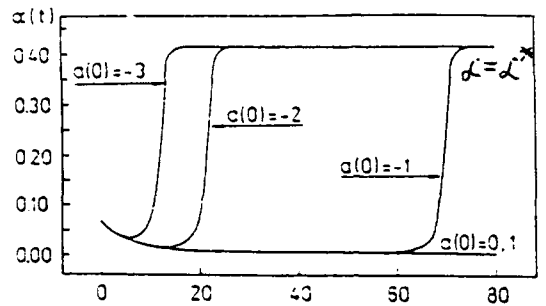
Fig. 2.2 The rcc \alpha(t) for different gauges a = 1, 0, -1, -2, -3 and \alpha(0) = 0.06 .
