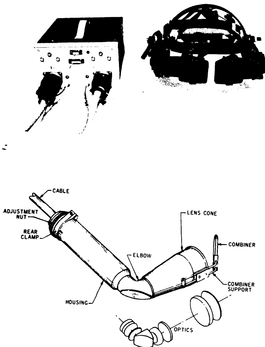
Figure 4. The VR Group HMD with Side-Mounted CRTs. The Image is Projected in Front of the Eyes by Means of Relay Optics and Mirrors
