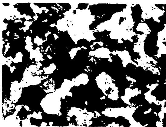
1A Extruded to 20.3 mm diameter bar Equiaxed \alpha phase
