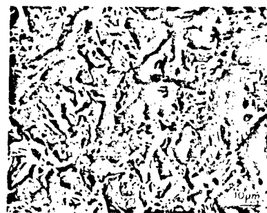
Figure 7. The fracture surface of Nb-10 at.% Si in the region of the rising resistance curve. Ductile stretching of the niobium is observed.
