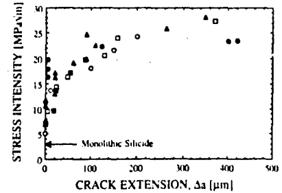
Figure 5. (a) Typical load-load point displacement traces from the three-point bend mechanical tests. (b) The corresponding stress intensity ( K ) vs. crack extension ( \Delta a ) plots for Nb-10 at.% Si.
