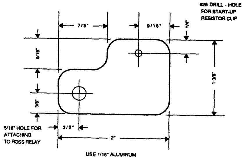
A. RELAY TERMINAL BRACKET
