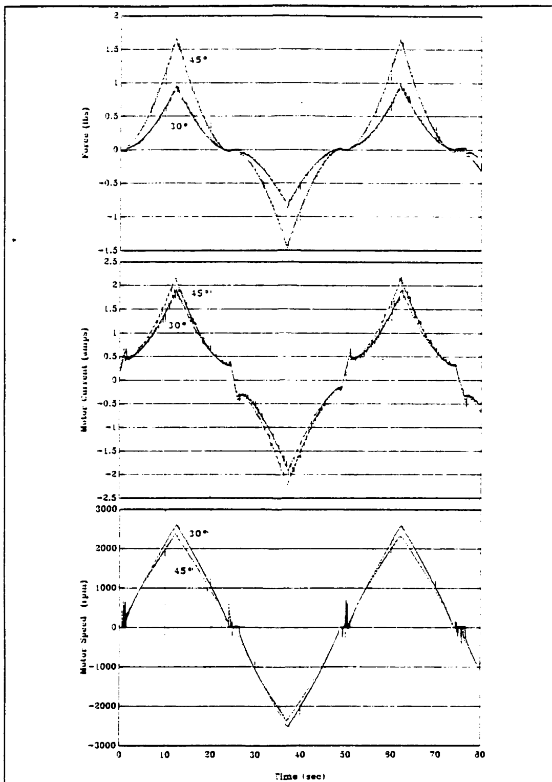
Figure 16 50 second period triangular wave, +/- 20.4 volts, 30° and 45° pitch propellers, 10.0 inch tunnel length
