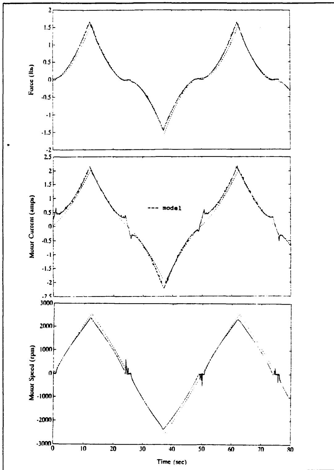
Figure 37 50 second period triangular wave, \pm 20.4 volts, 45^\circ pitch propeller, 10.0 inch tunnel length with model
