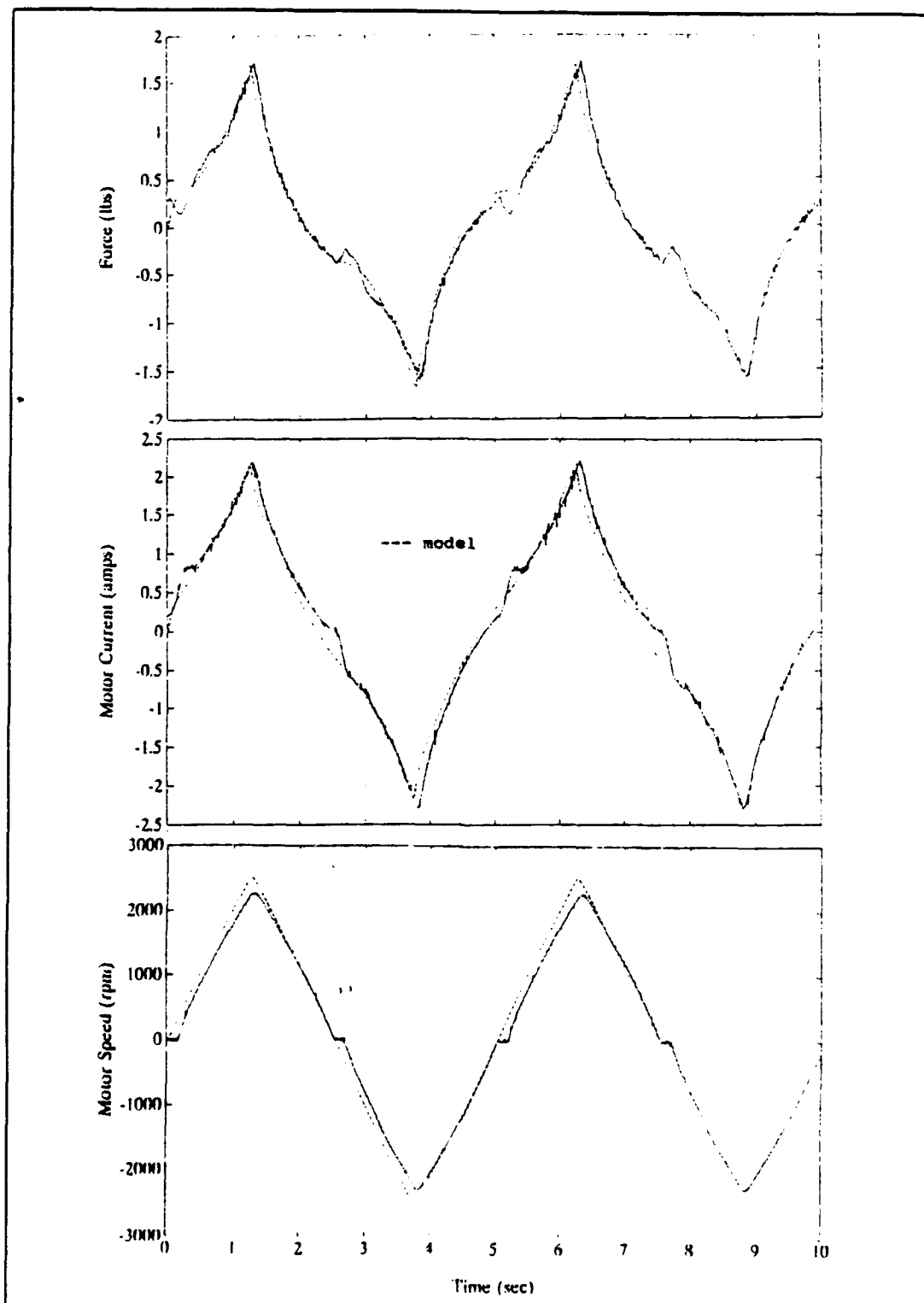
Figure 40 5 second period triangular wave, \pm 20.4 volts, 45^\circ pitch propeller, 16.5 inch tunnel length with model
