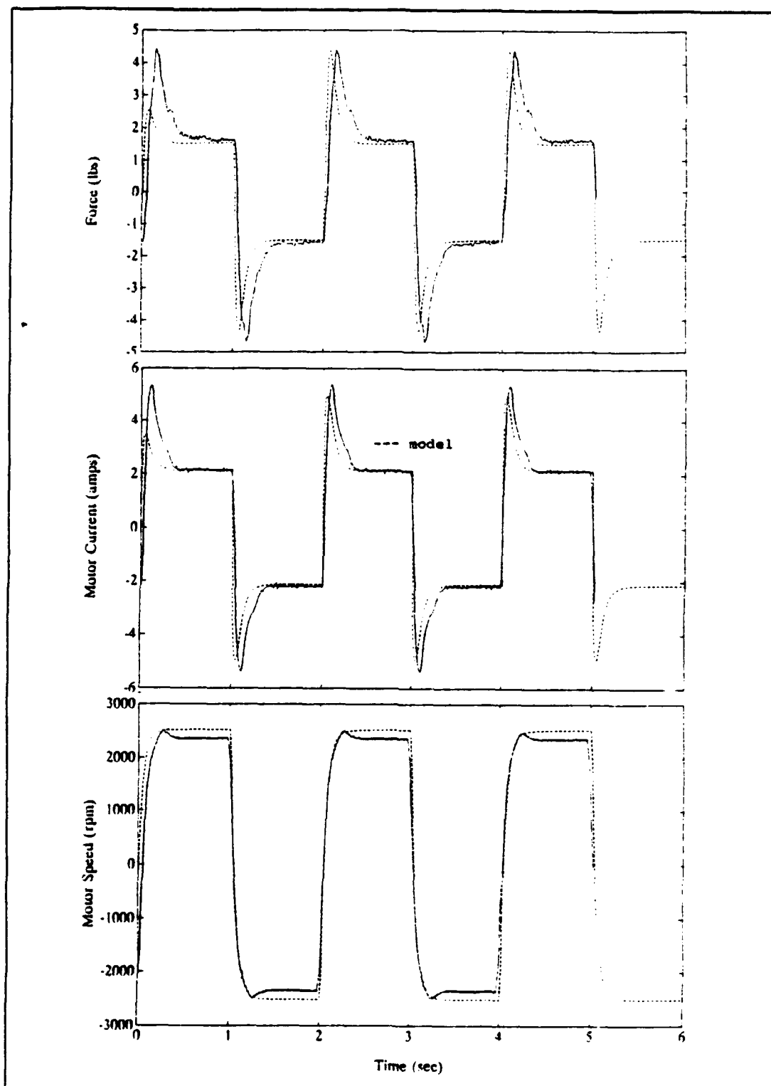
Figure 46 2 second period square wave, \pm 20.4 volts, 45^\circ pitch propeller, 10.0 inch tunnel length with model
