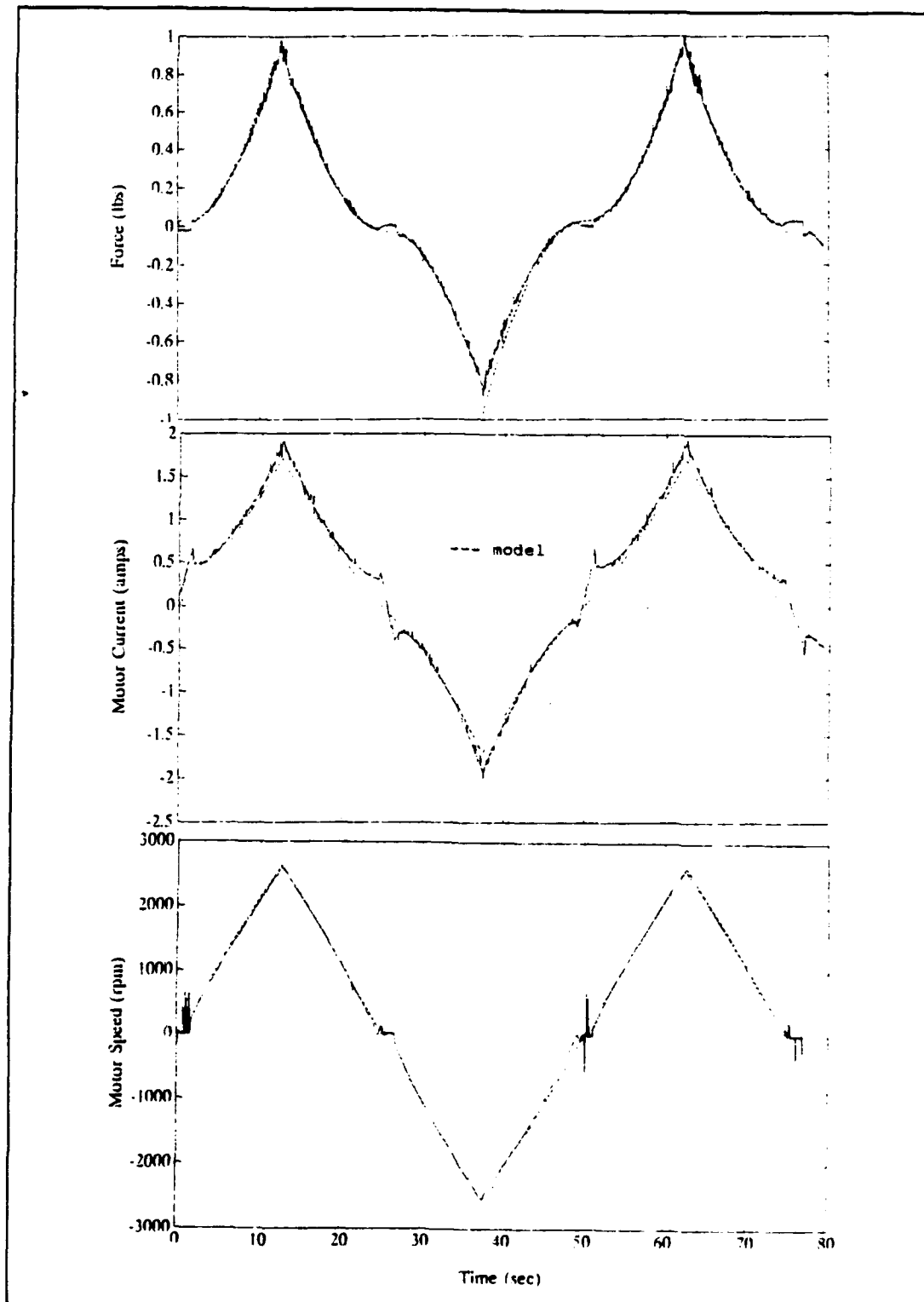
Figure 35 50 second period triangular wave, \pm 20.4 volts, 30^\circ pitch propeller, 10.0 inch tunnel length with model
