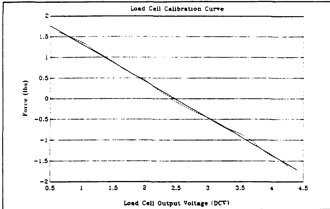
Figure 11 Load Cell Calibration Curve
