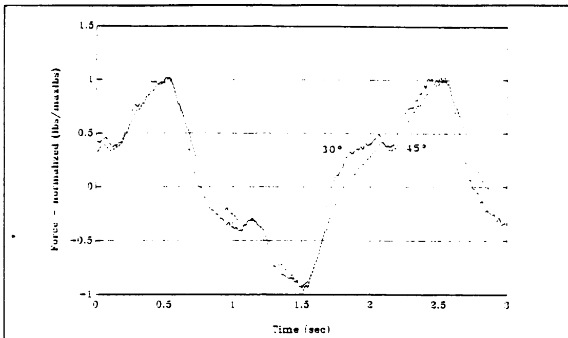
Figure 27 2 second period triangular wave, \pm 20.4 volts 30^\circ & 45^\circ pitch propellers, 16.5 inch tunnel length
