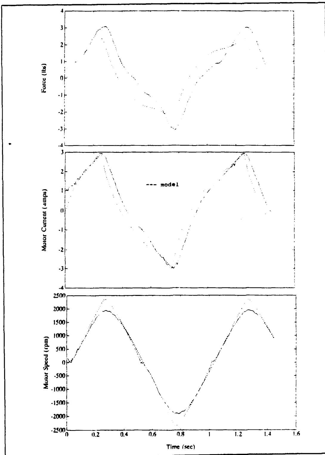
Figure 42 1 second period triangular wave, \pm 20.4 volts, 45^\circ pitch propeller, 16.5 inch tunnel length with model
