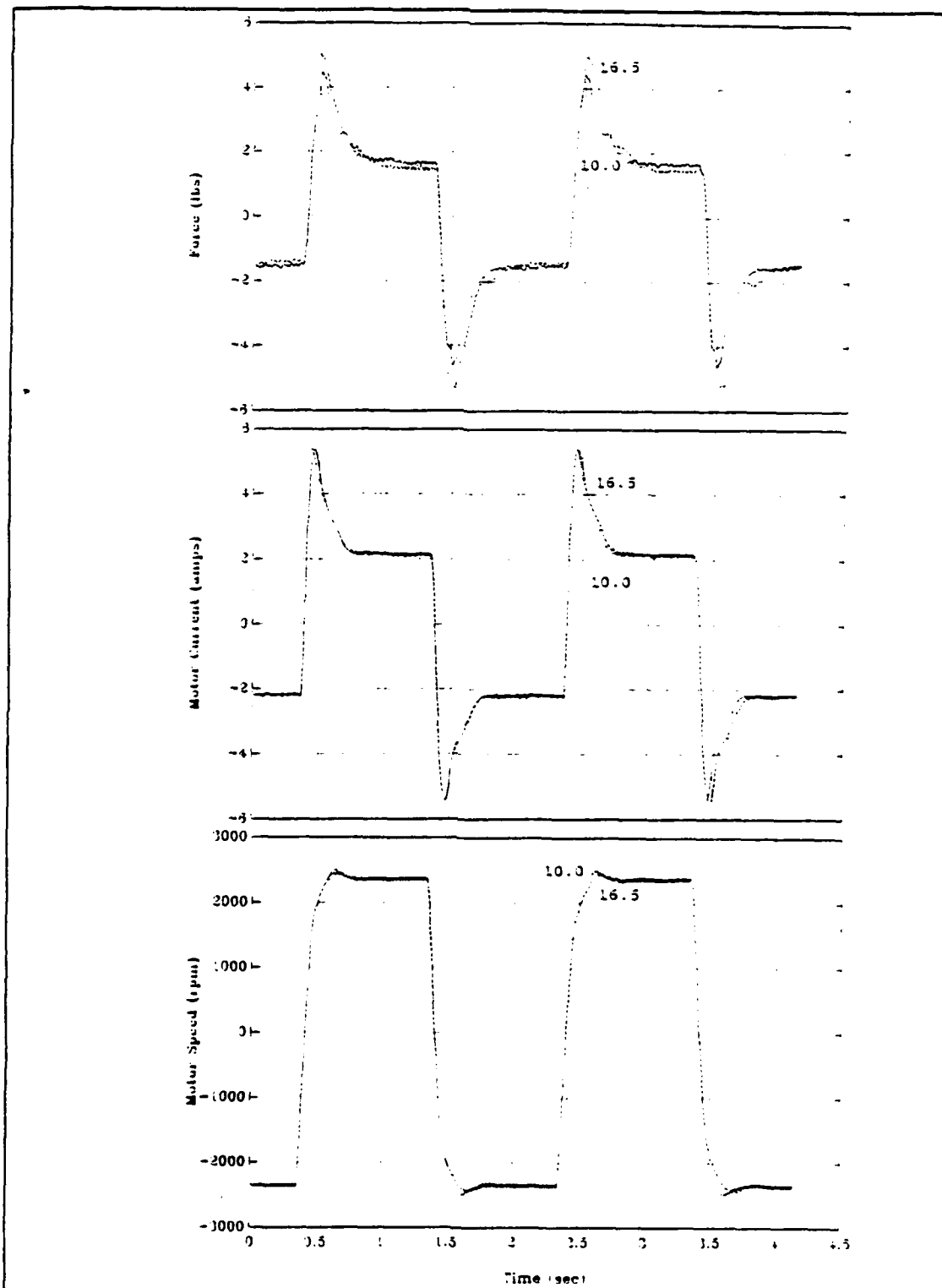
Figure 33 2 second period square wave, +/- 20.4 volts, 45° pitch propeller, 10.0 & 16.5 inch tunnel lengths
