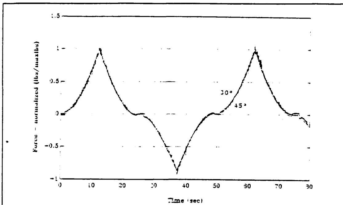
Figure 23 50 second period triangular wave, \pm 20.4 volts 30^\circ & 45^\circ pitch propellers, 10.0 inch tunnel length
