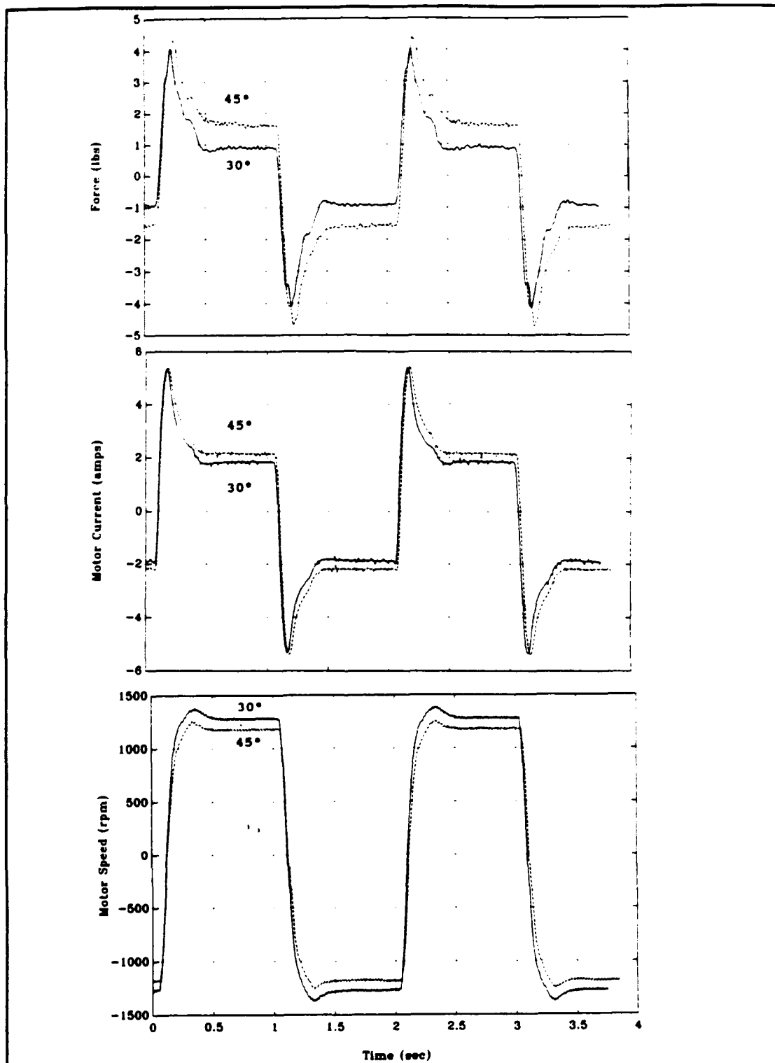
Figure 30 2 second period square wave, +/- 20.4 volts, 30° & 45° pitch propellers, 10.0 inch tunnel length
