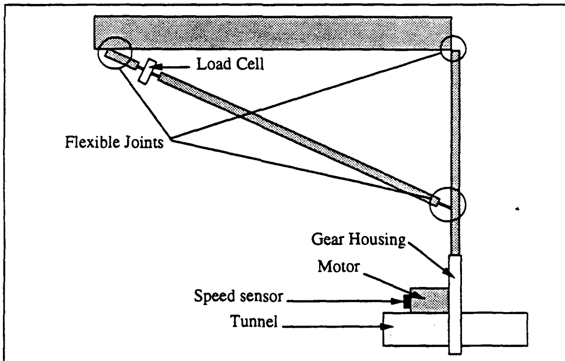
Figure 6 Test Frame Assembly
