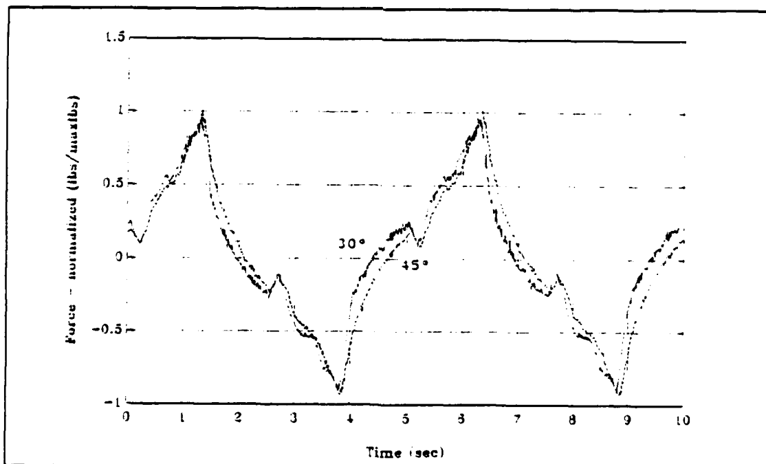
Figure 26 5 second period triangular wave, +/- 20.4 volts 30° & 45° pitch propellers, 16.5 inch tunnel length
