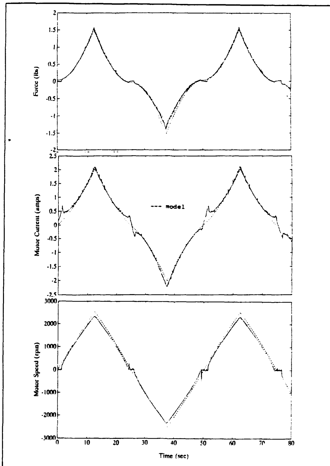
Figure 38 50 second period triangular wave, \pm 20.4 volts, 45^\circ pitch propeller, 16.5 inch tunnel length with model
