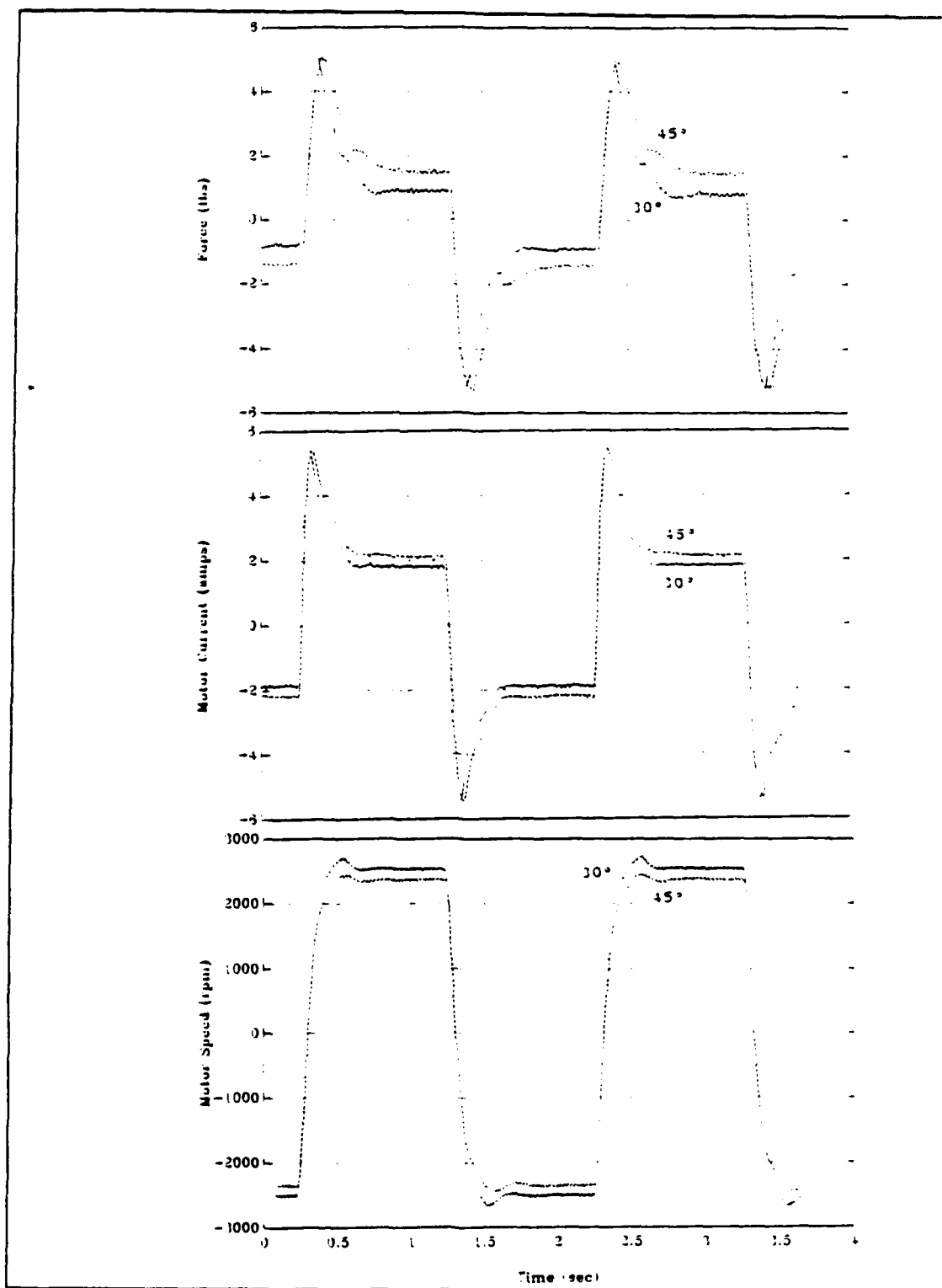
Figure 31 2 second period square wave, \pm 20.4 volts, 30^\circ & 45^\circ pitch propellers, 16.5 inch tunnel length
