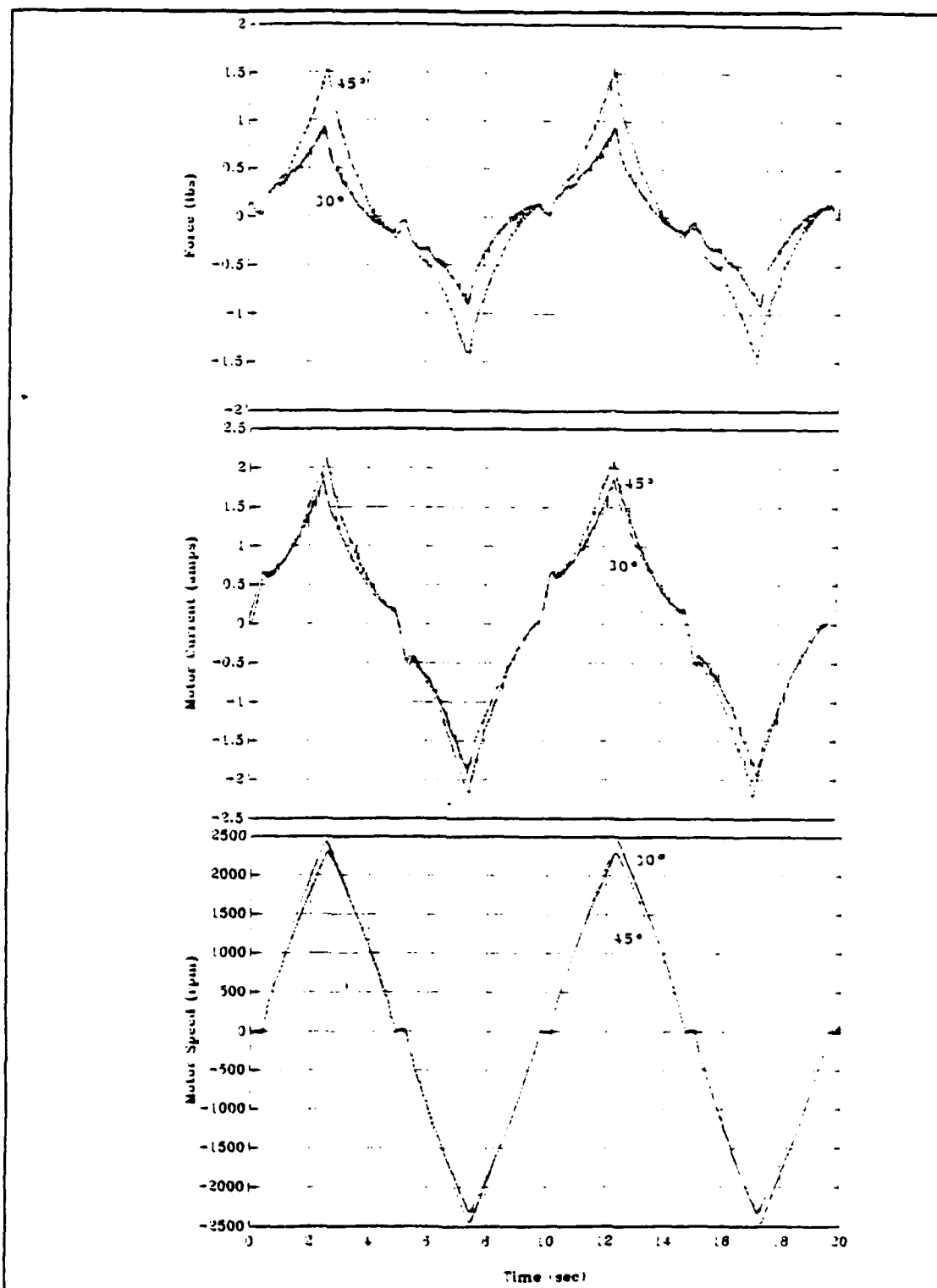
Figure 18 10 second period triangular wave, \pm 20.4 volts, 30^\circ & 45^\circ pitch propellers, 16.5 inch tunnel length
