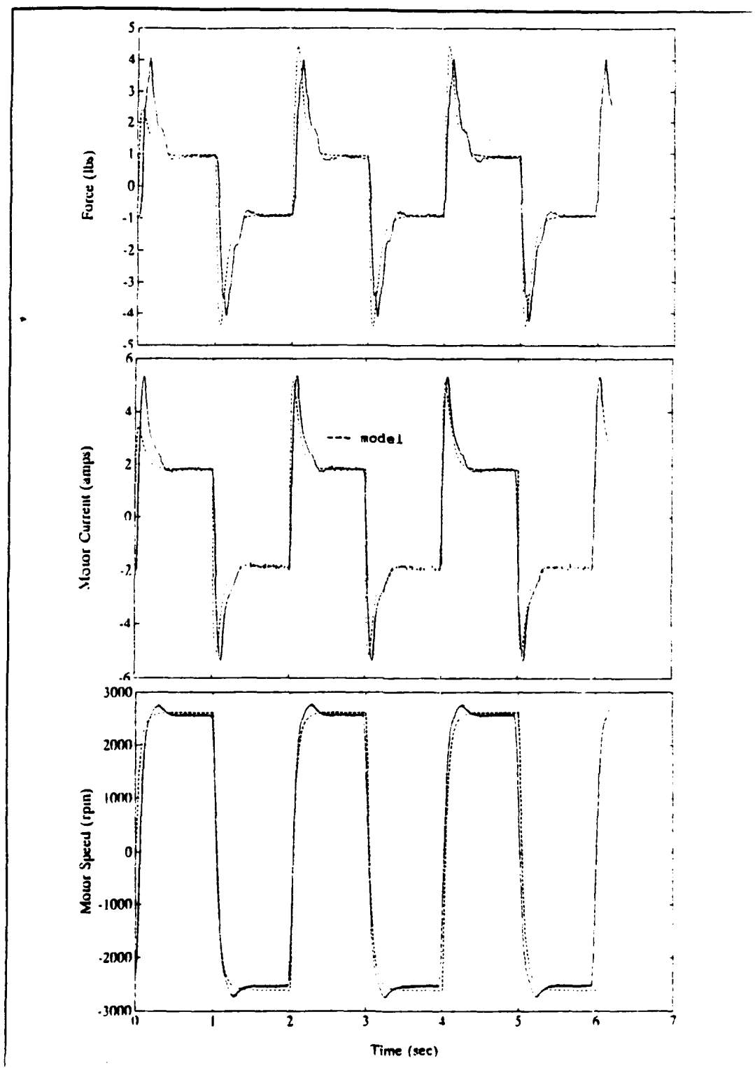
Figure 44 2 second period square wave, \pm 20.4 volts, 30^\circ pitch propeller, 10.0 inch tunnel length with model
