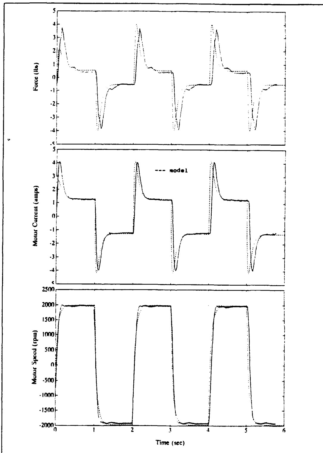
Figure 48 2 second period square wave, \pm 18.4 volts, 30^\circ pitch propeller, 16.5 inch tunnel length with model
