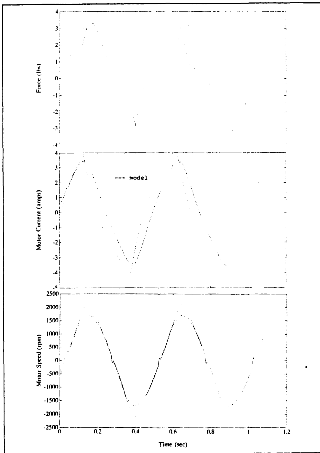
Figure 43 0.5 second period triangular wave, \pm 20.4 volts, 45^\circ pitch propeller, 16.5 inch tunnel length with model
