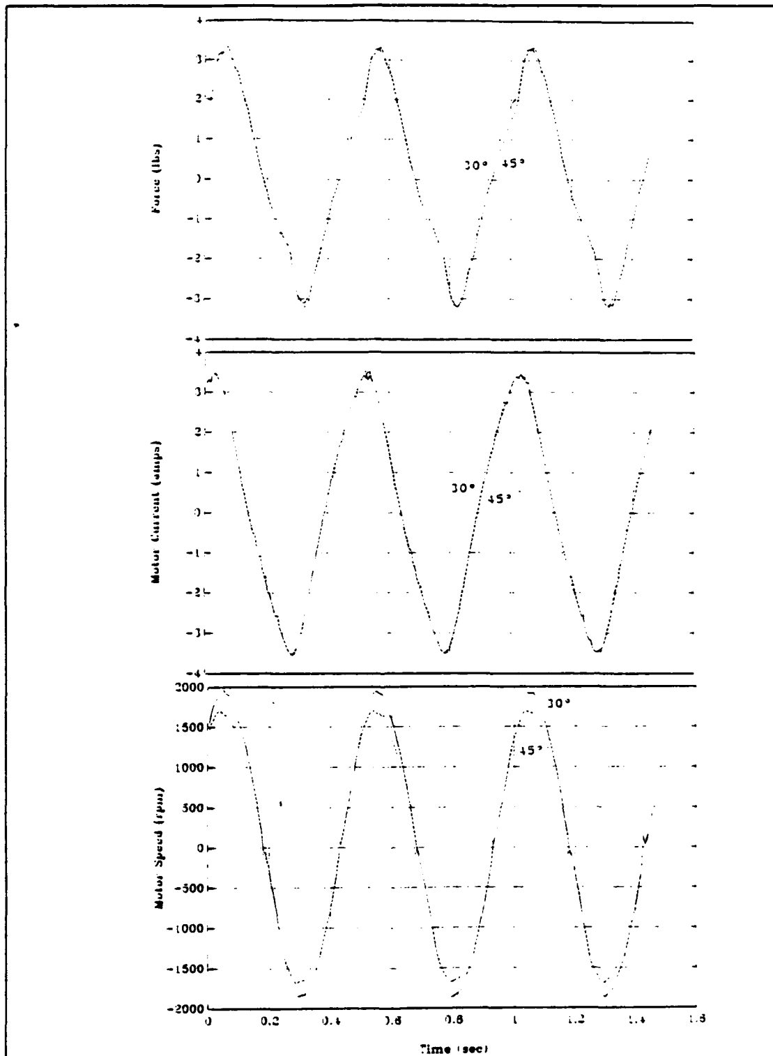
Figure 22 0.5 second period triangular wave, +/-20.4 volts, 30° & 45° pitch propellers, 16.5 inch tunnel length
