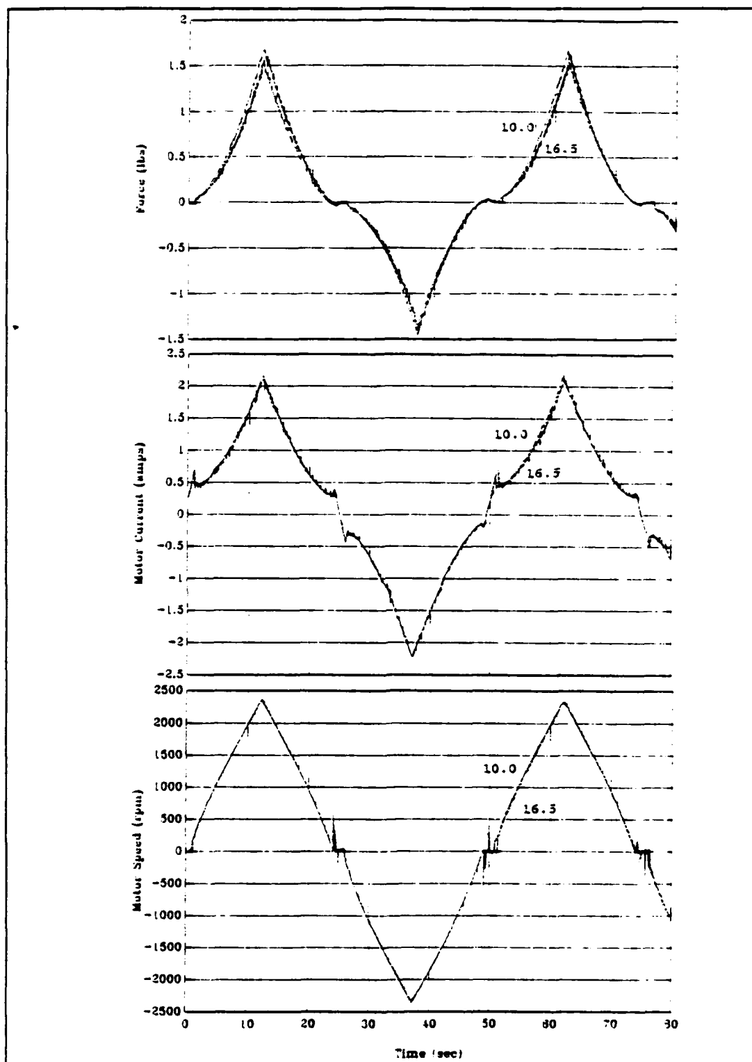
Figure 15 50 second period triangular wave, \pm 20.4 volts, 45^\circ pitch propeller, 10.0 and 16.5 in tunnel lengths
