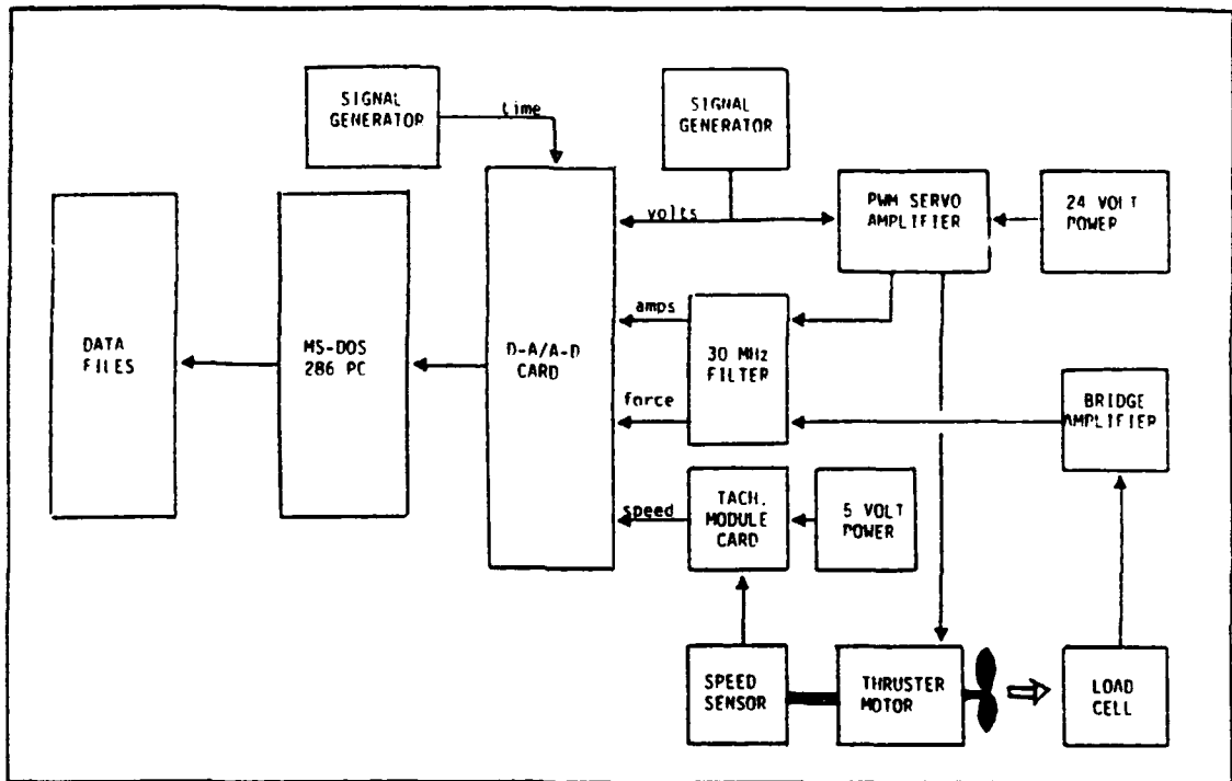
Figure 9 Block Diagram of Experimental Setup
