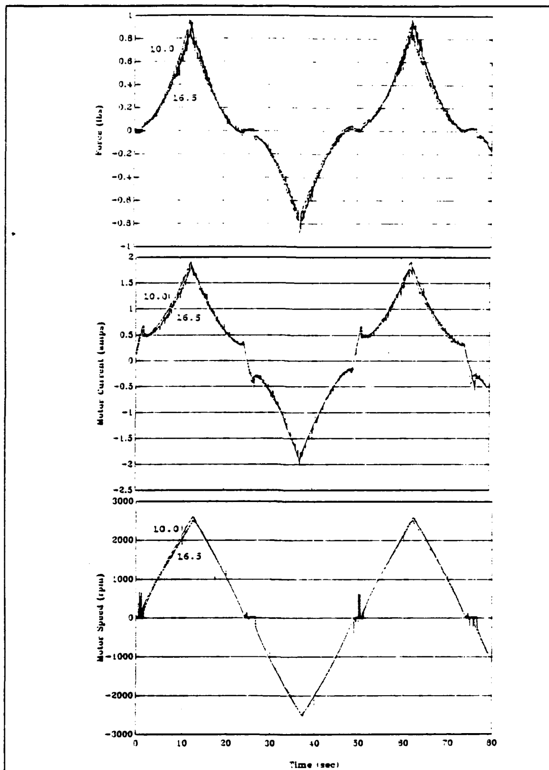
Figure 14 50 second period triangular wave, \pm 20.4 volts, 30^\circ pitch propeller, 10.0 and 16.5 inch tunnel lengths
