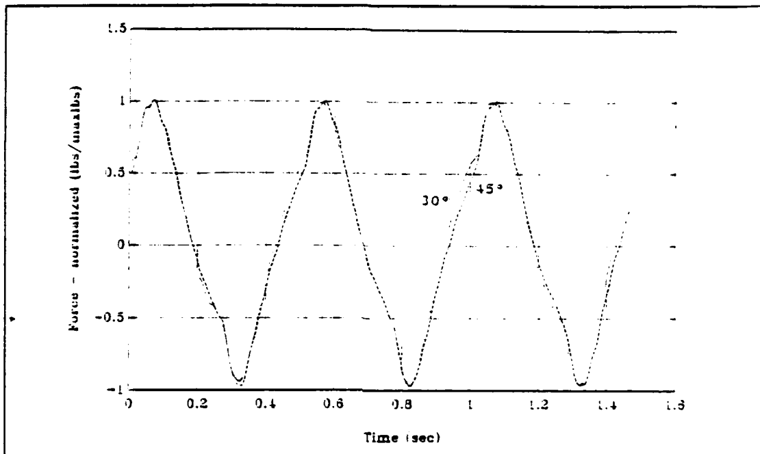
Figure 29 0.5 second period triangular wave, +/-20.4 volts 30° & 45° pitch propellers, 16.5 inch tunnel length
