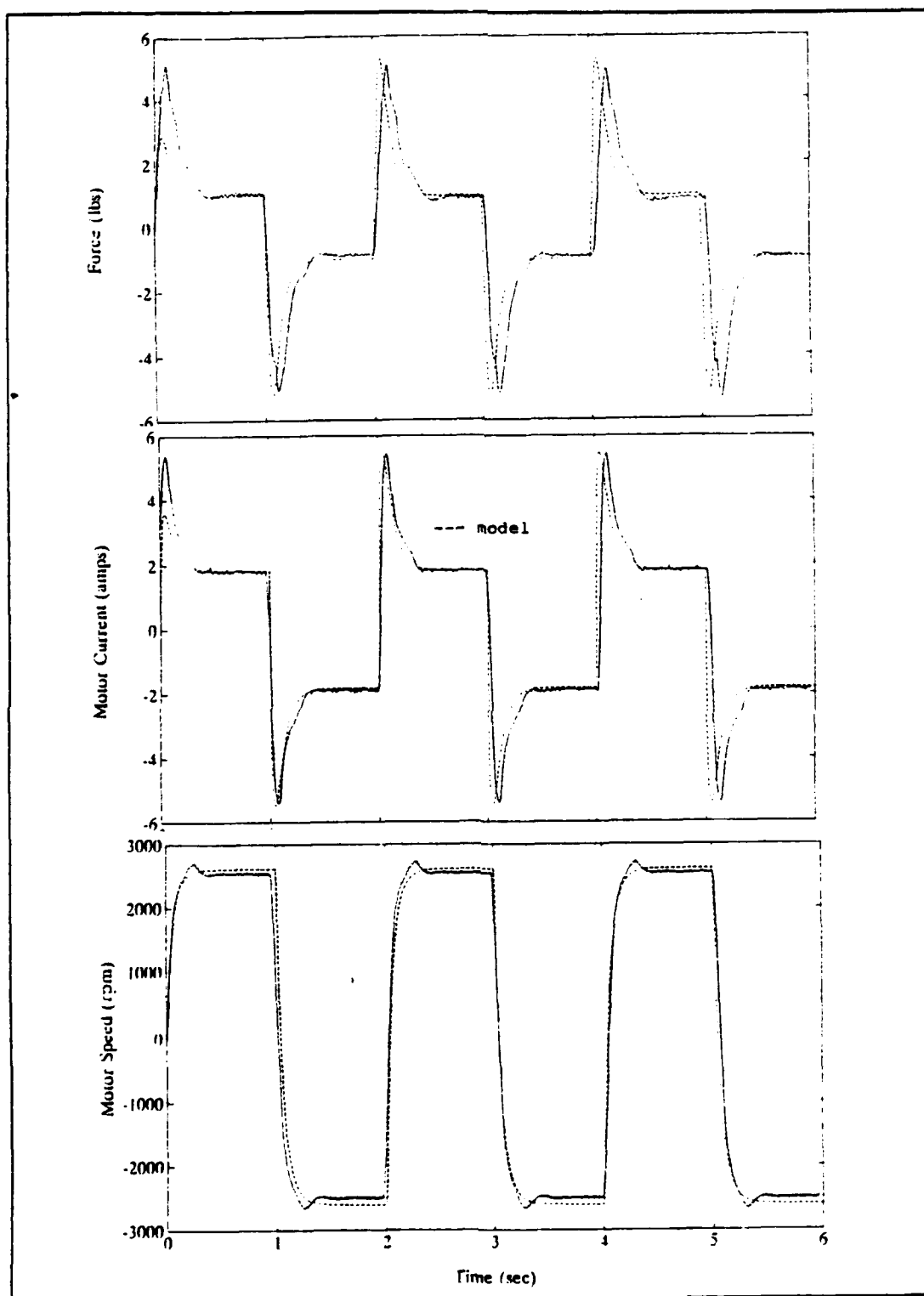
Figure 45 2 second period square wave, \pm 20.4 volts, 30^\circ pitch propeller, 16.5 inch tunnel length with model
