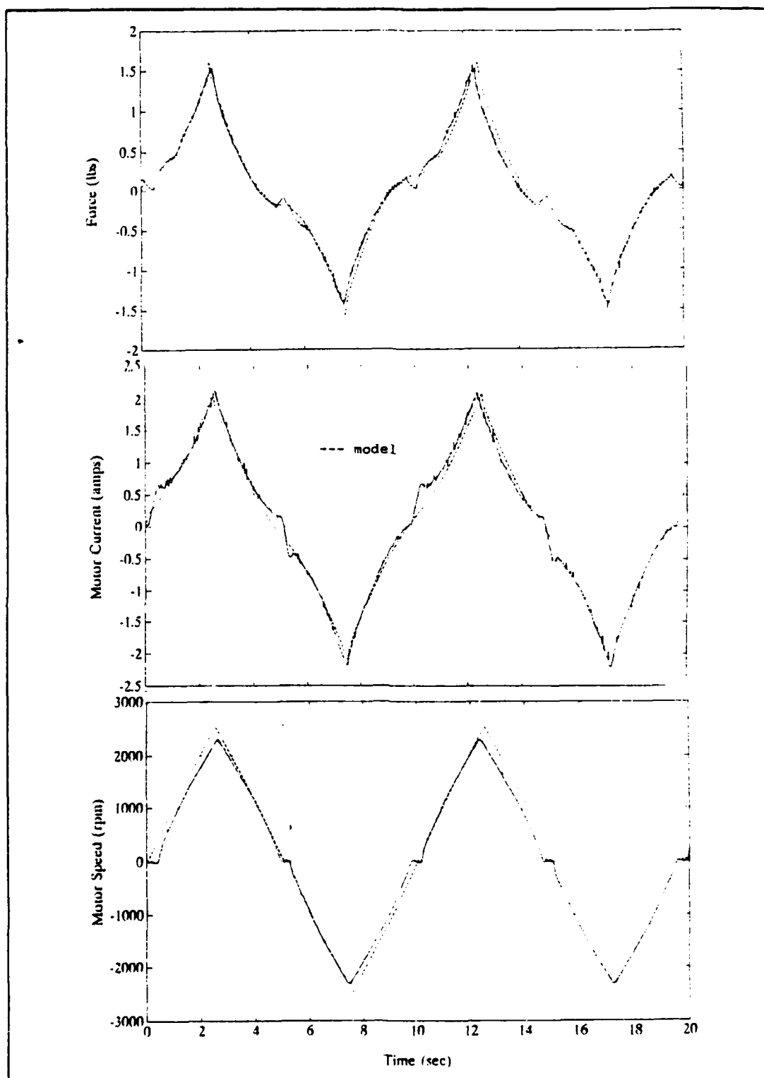
Figure 39 10 second period triangular wave, \pm 20.4 volts, 45^\circ pitch propeller, 16.5 inch tunnel length with model
