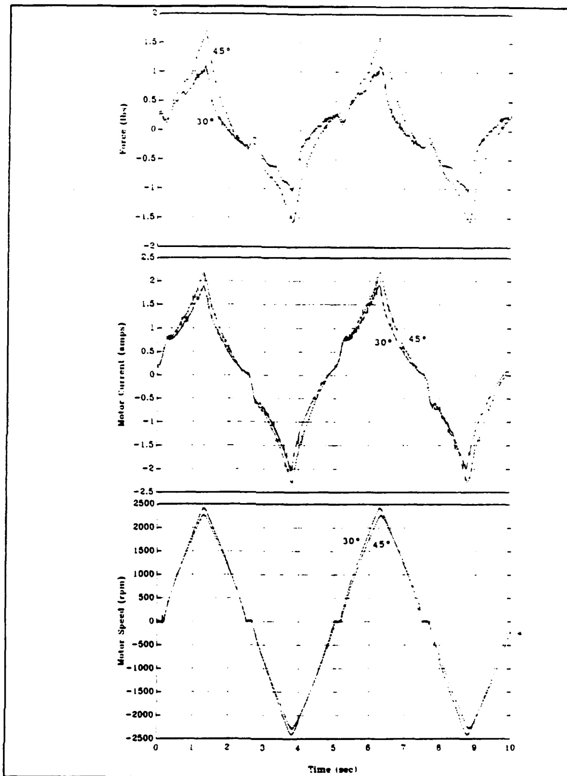
Figure 19 5 second period triangular wave, +/- 20.4 volts, 30° & 45° pitch propellers, 16.5 inch tunnel length
