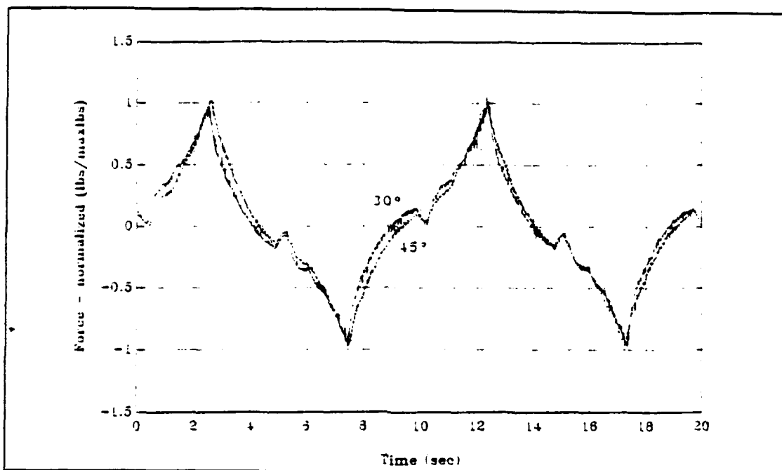
Figure 25 10 second period triangular wave, +/- 20.4 volts 30° & 45° pitch propellers, 16.5 inch tunnel length
