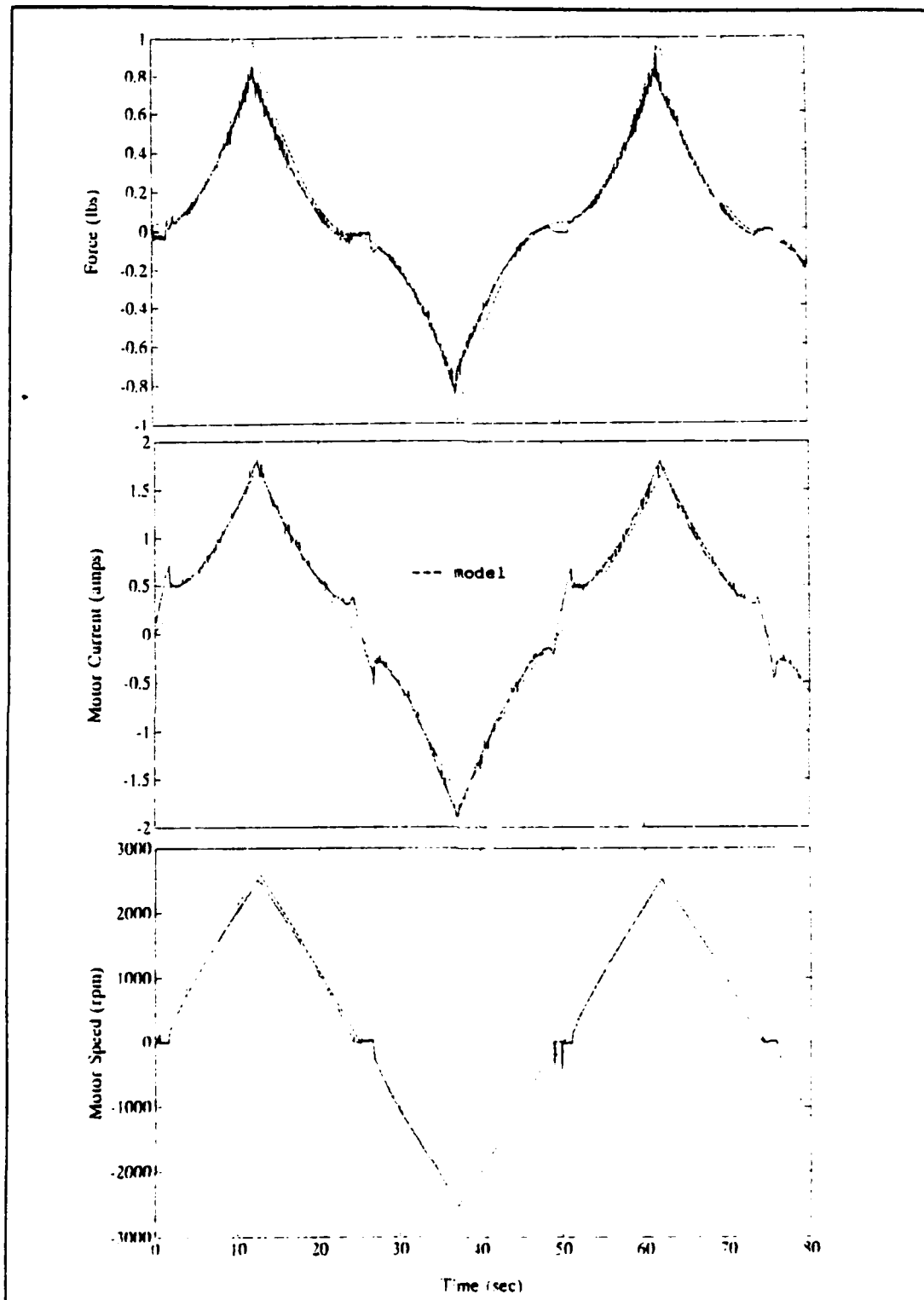
Figure 36 50 second period triangular wave, \pm 20.4 volts, 30^\circ pitch propeller, 16.5 inch tunnel length with model
