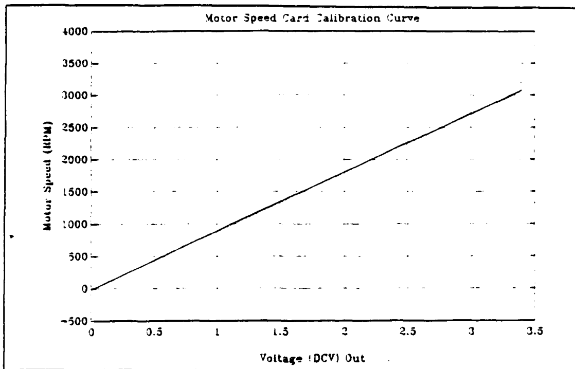
Figure 13 Motor Speed Calibration Curve
