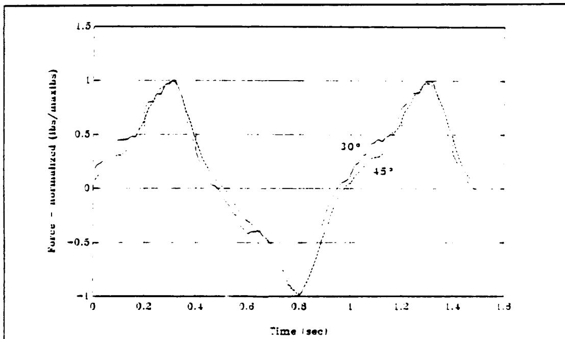
Figure 28 1 second period triangular wave, \pm 20.4 volts 30^\circ & 45^\circ pitch propellers, 16.5 inch tunnel length
