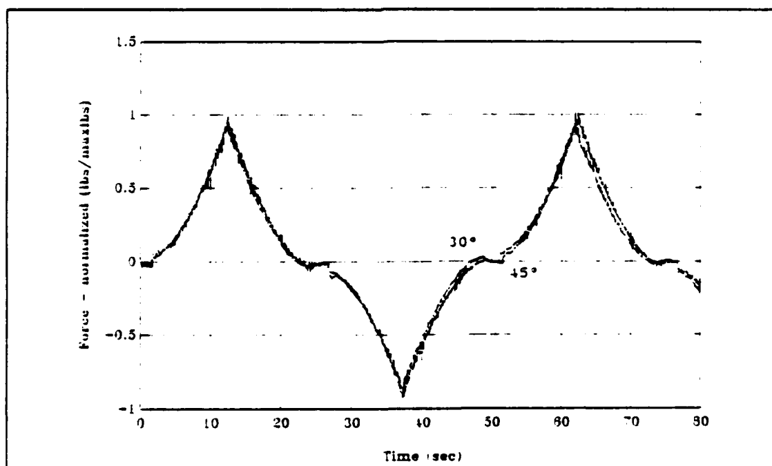
Figure 24 50 second period triangular wave, \pm 20.4 volts 30^\circ & 45^\circ pitch propellers, 16.5 inch tunnel length
