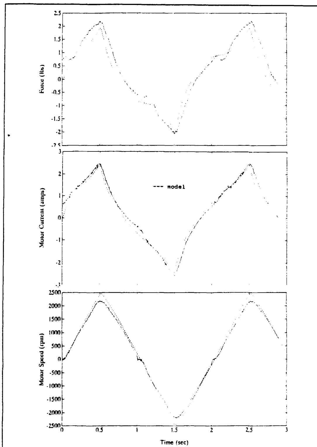
Figure 41 2 second period triangular wave, \pm 20.4 volts, 45^\circ pitch propeller, 16.5 inch tunnel length with model
