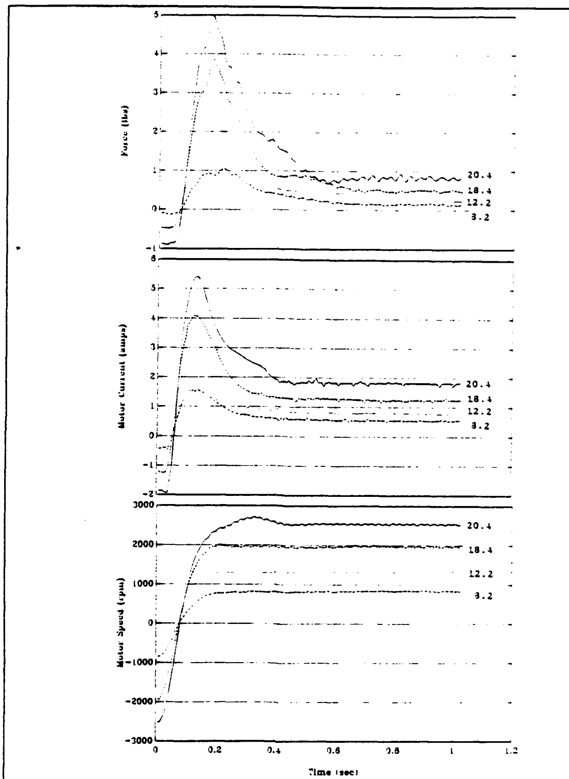
Figure 34 2 second period square wave, +/- 20.4, 18.4, 12.2, and 8.2 volts, 30° pitch propeller, 16.5 inch tunnel length
