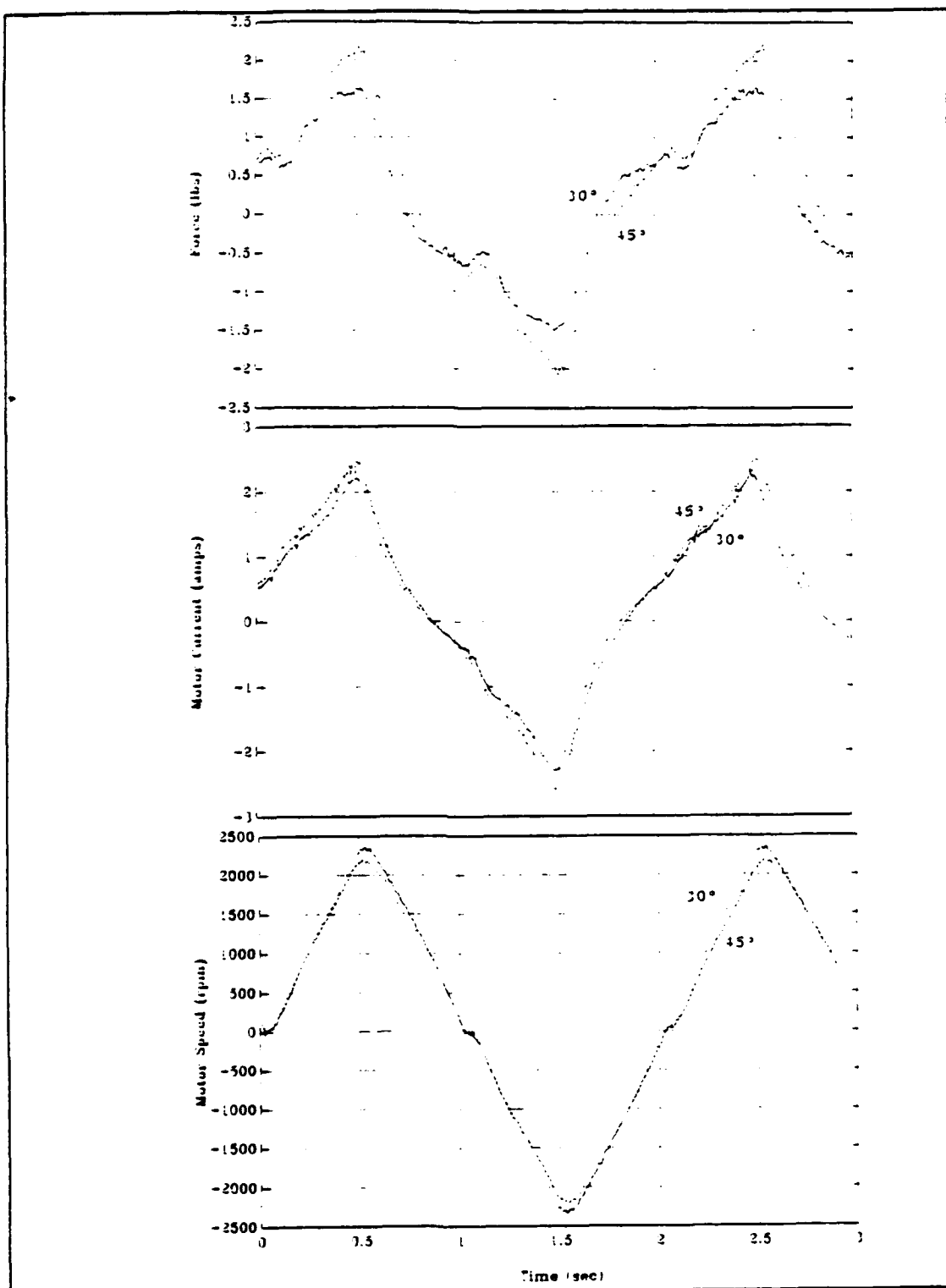
Figure 20 2 second period triangular wave, +/- 20.4 volts, 30° & 45° pitch propellers, 16.5 inch tunnel length
