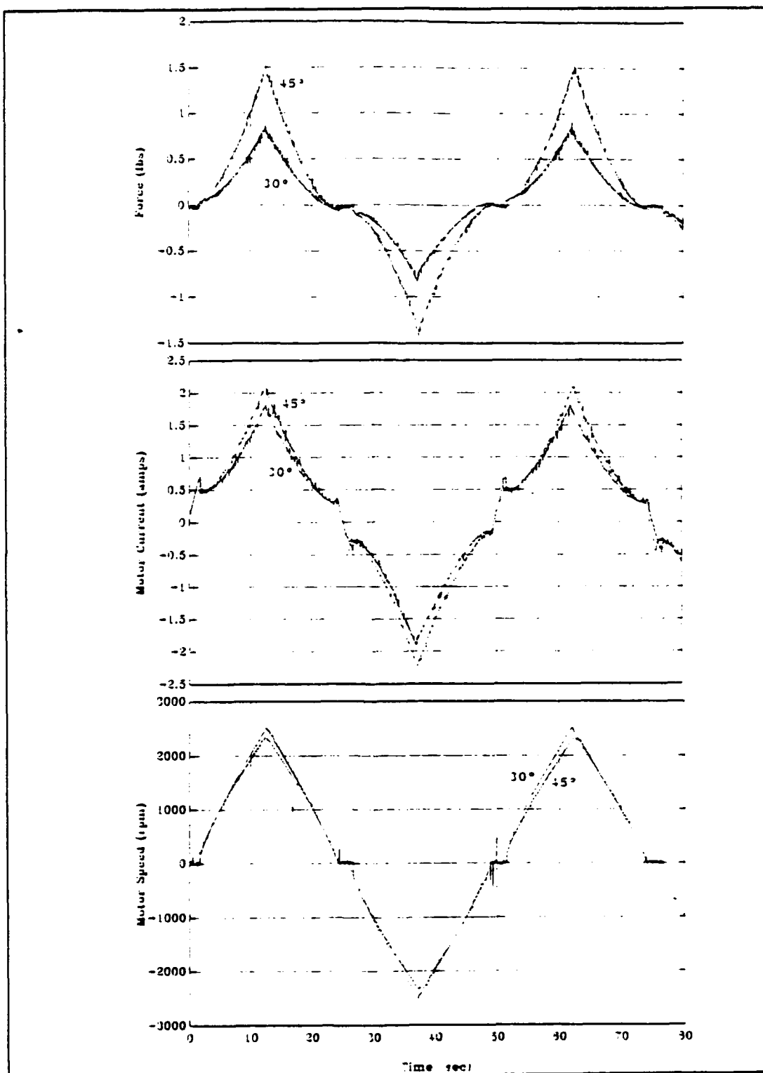
Figure 17 50 second period triangular wave, +/- 20.4 volts, 30° and 45° pitch propellers, 16.5 inch tunnel length
