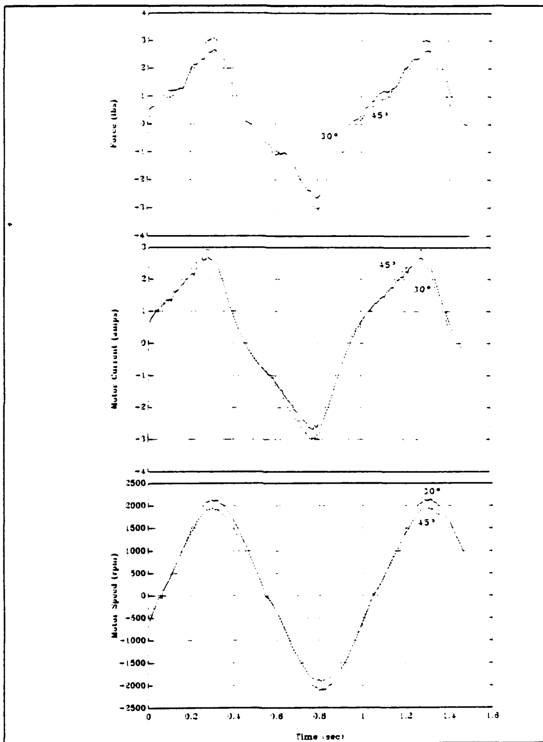
Figure 21 1 second period triangular wave, +/- 20.4 volts, 30° & 45° pitch propellers, 16.5 inch tunnel length
