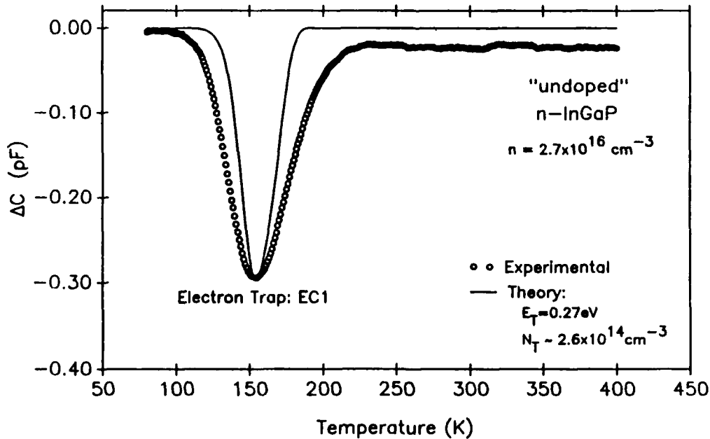
Figure 4. DLTS spectrum of "undoped" InGaP sample. Emission rate = 14\text{ s}^{-1} , bias = -2 to -1 V, and pulse width = 10 ms.
