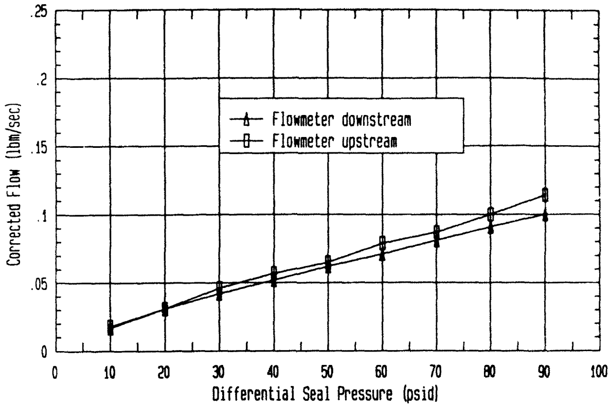
FIGURE 13. SIMPLE ORIFICES VERSUS PREDICTED FLOW
