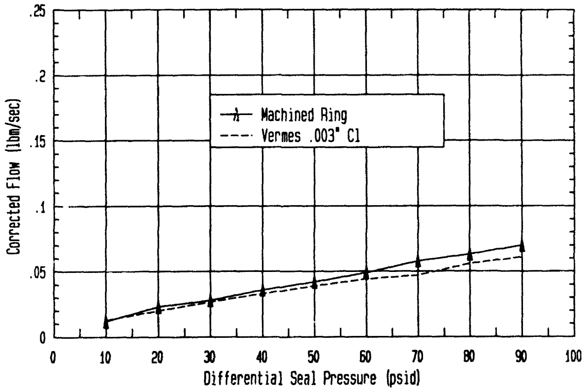
FIGURE 14. MACHINED RING VERSUS PREDICTED FLOW
