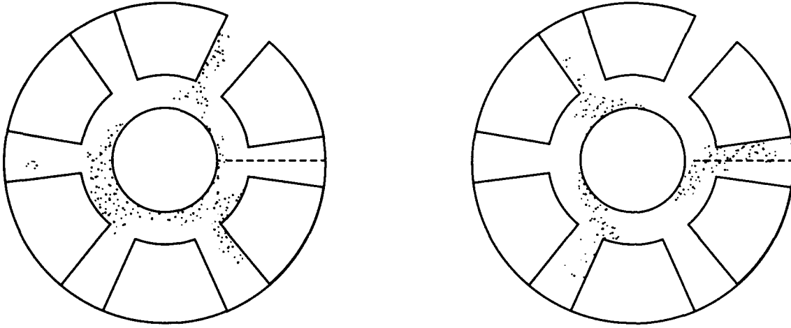
Figure 4. Magnetrons out of phase. Particle distribution at 12 nsec with transmission line length L = 0.5 wavelength and impedance Z_0 = 0.1 ohm.
