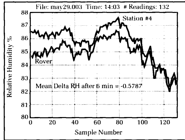
Figure 6. Relative humidity (rover vs. #4).
