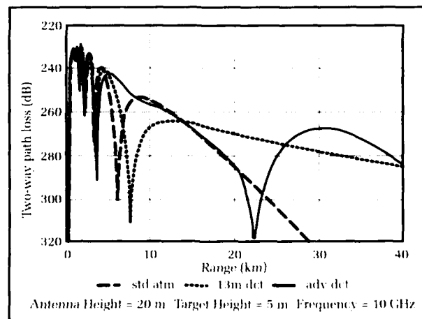
Figure 2. Two-way path loss versus range for three different refractive conditions.
