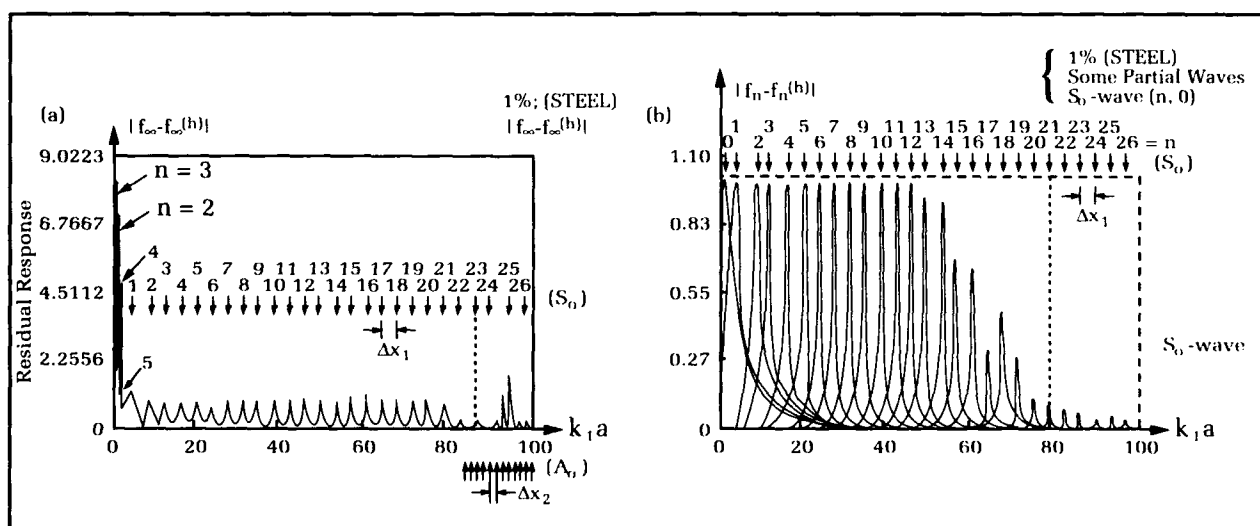
Figure 4. (a) Total residual response obtained by the novel hybrid background. (b) The leading portions of the first few modal residual responses, as obtained by the subtraction of the novel hybrid backgrounds.
