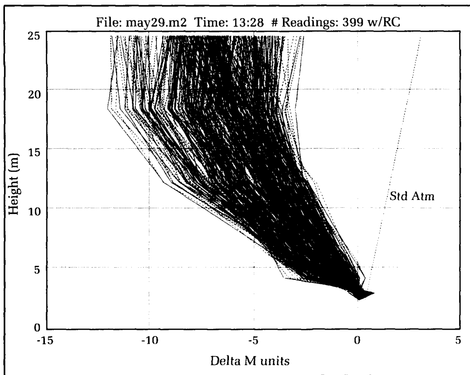
Figure 12. Delta M unit profiles spanning 33 min., May 29, 13:28 UTC.
