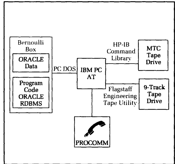
Figure 2. ALTSS software.
