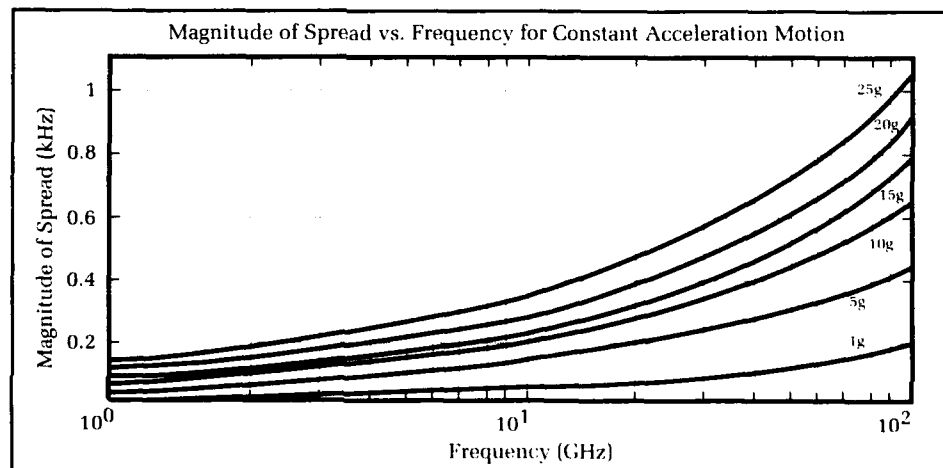
Figure 3. Spread in frequency due to varying accelerations.
