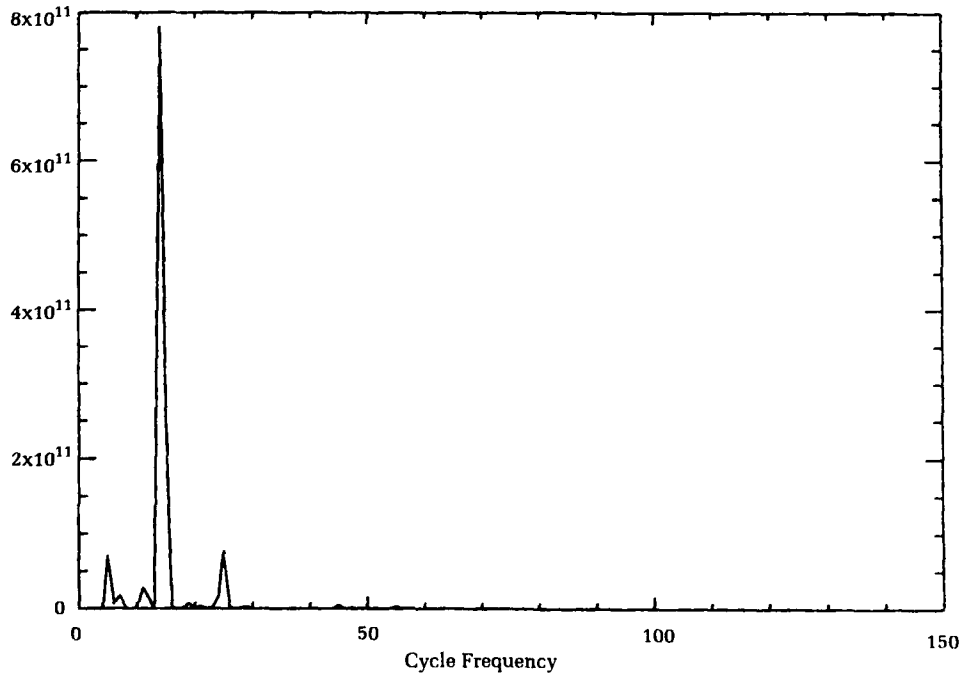
Figure 5. Direct-cycle frequency estimate of transmitted 8-ary frequency shift keyed data (dry end). The stationary part of the signal, which maps to the zero correlation axis, has been removed. ( N=64 , L=2 , I=4 , K_{dc}=1 .)
