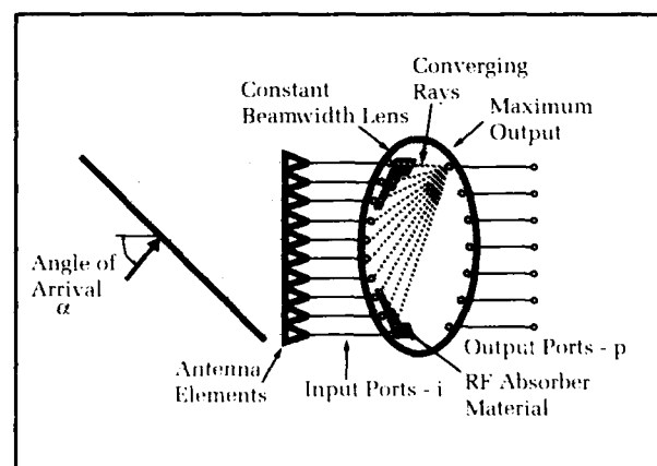
Figure 2. Bootlace lens antenna—direction-finding system.
