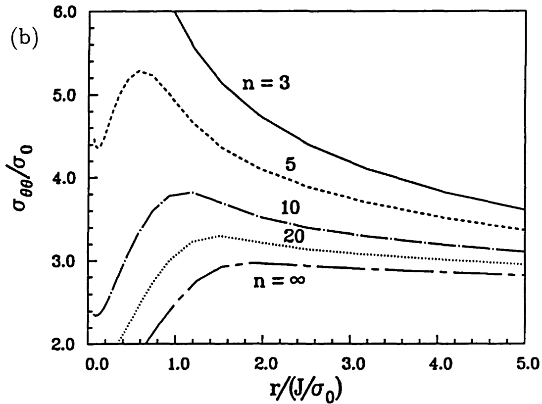
Figure 2. Plane strain reference fields for n = 3, 5, 10, 20 and \infty ( E/\sigma_0 = 500, \nu = 0.3 ). Hoop stress reference fields, (a) small strain (b) finite strain. Mean stress reference fields, (c) small strain (d) finite strain
