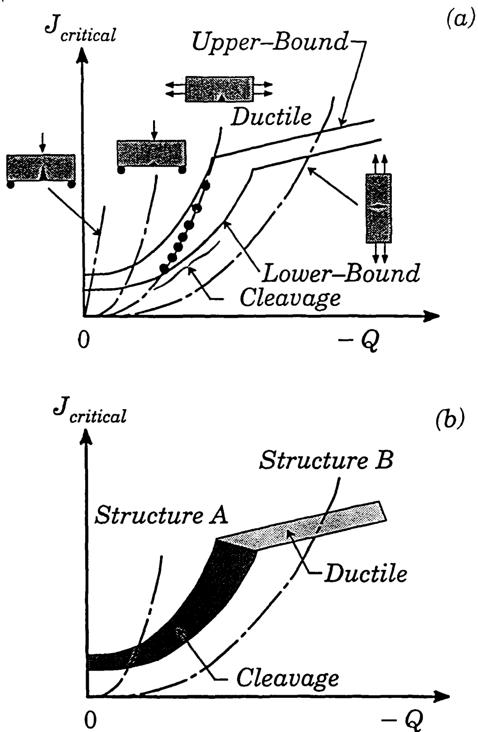
Figure 17. Illustration of J - Q methodology. (a) Laboratory testing of specimens of varying constraints to measure the material's fracture resistance. Circles indicate anticipated scatter in the measured cleavage toughness data which define the upper and lower bounds. (b) Evaluation of structures using measured toughness locus and predicted J - Q load path for two structural geometries.
