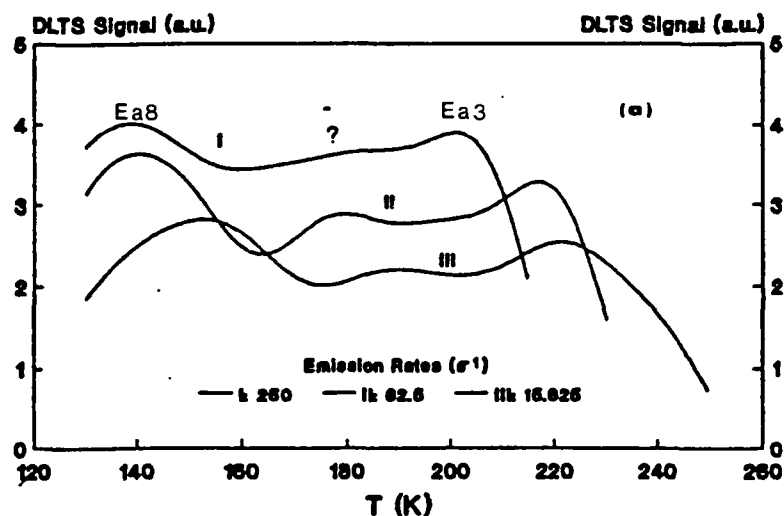
Fig.4 S4 samples IDS-DLTS spectra obtained after a radiation dose of 3.8 \times 10^{12}\text{cm}^{-2} He ions.
