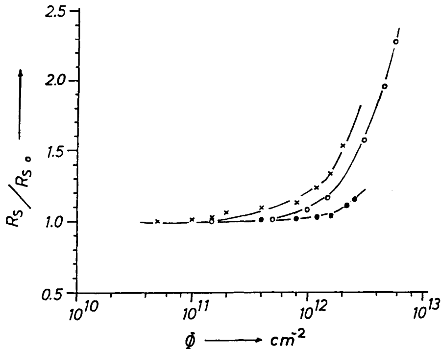
Fig.20 Variation of the normalized R_s / R_{s0} , to their values before radiation, parasitic resistances vs radiation dose for: (x) structure A, (o) structure B and (●) structure C.
