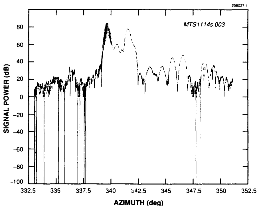
Figure 14. MTS PPI scan data [(gate 81) three-degree elevation, 1114 PRF, five degree per second scan rate)].
