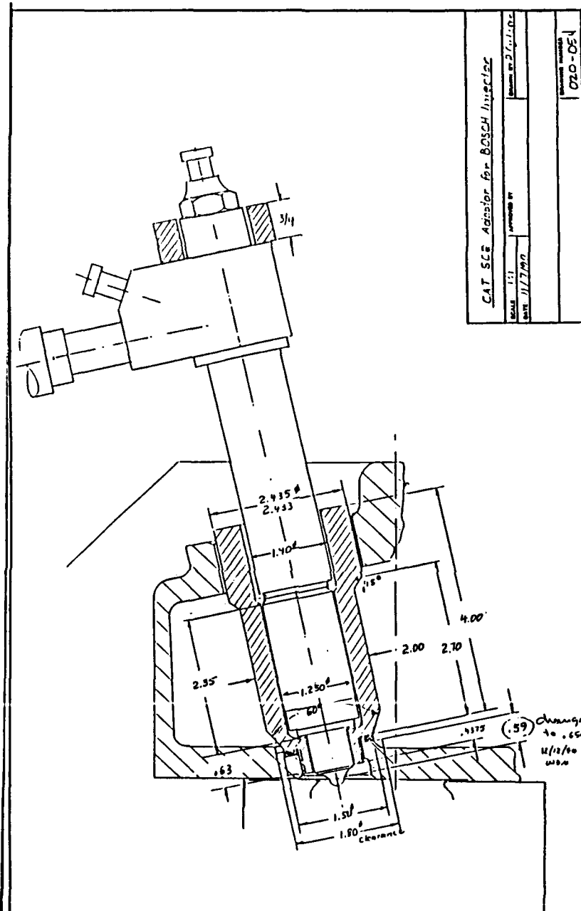
Figure 5.4-6. Bosch Type Injector in 1Y73 Cylinder Head
