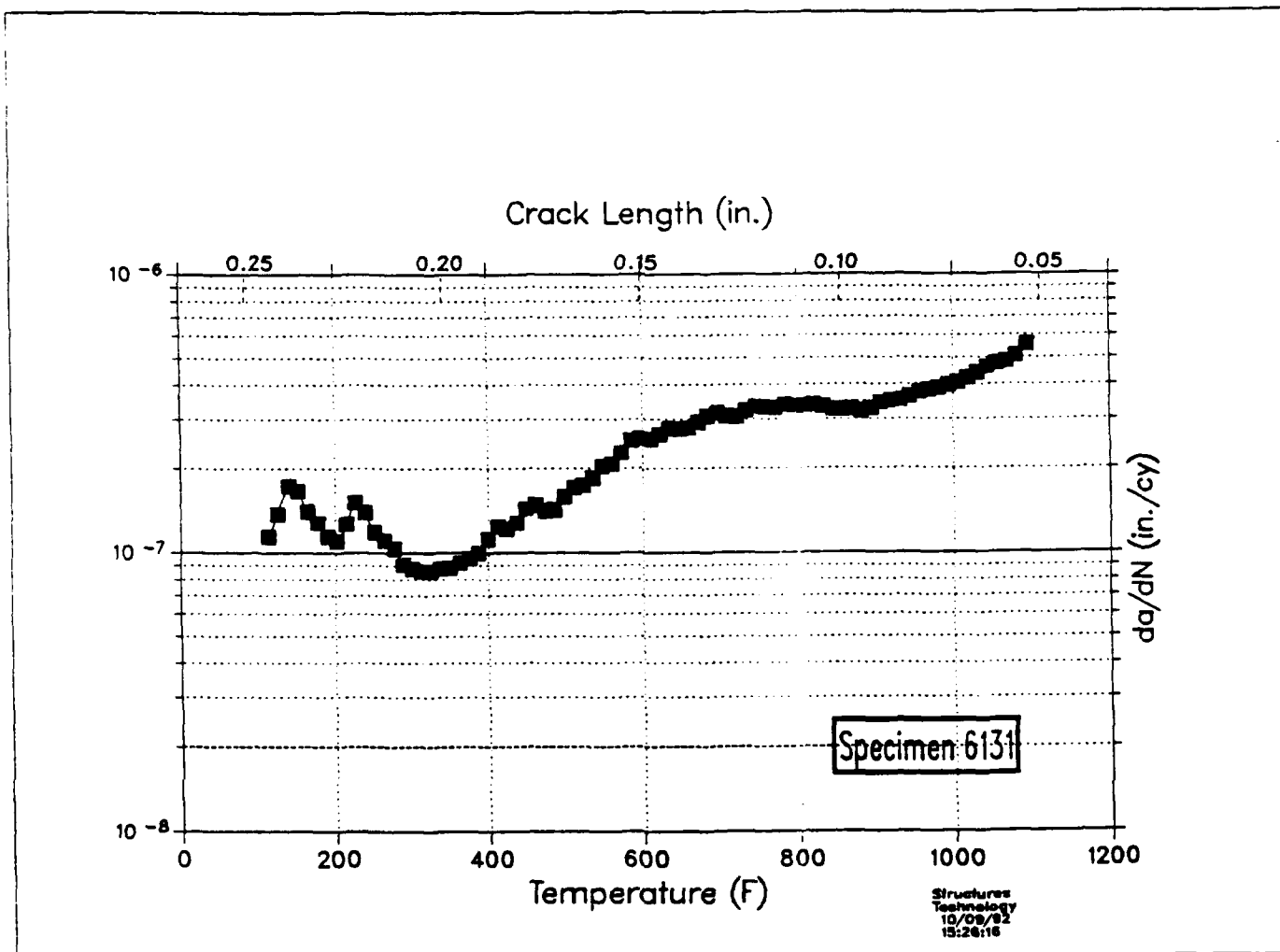
Figure 1: Crack Growth Rate vs. Temperature for PWA 1484, \Delta K = 6.5 \text{ ksi} \sqrt{\text{in.}} , Stress Ratio = 0.5, Frequency = 10 Hz from a Temperature Decreasing Test Between 1300F and 77F at Constant Stress Intensity.
