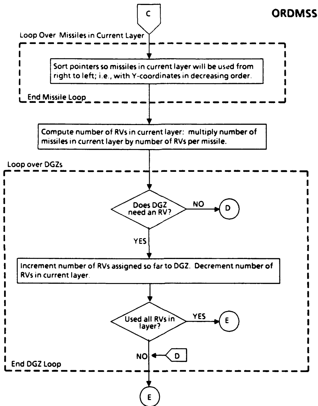
FIGURE 5-5 SUBROUTINE ORDMSS PROCESS FLOW (Continued)
