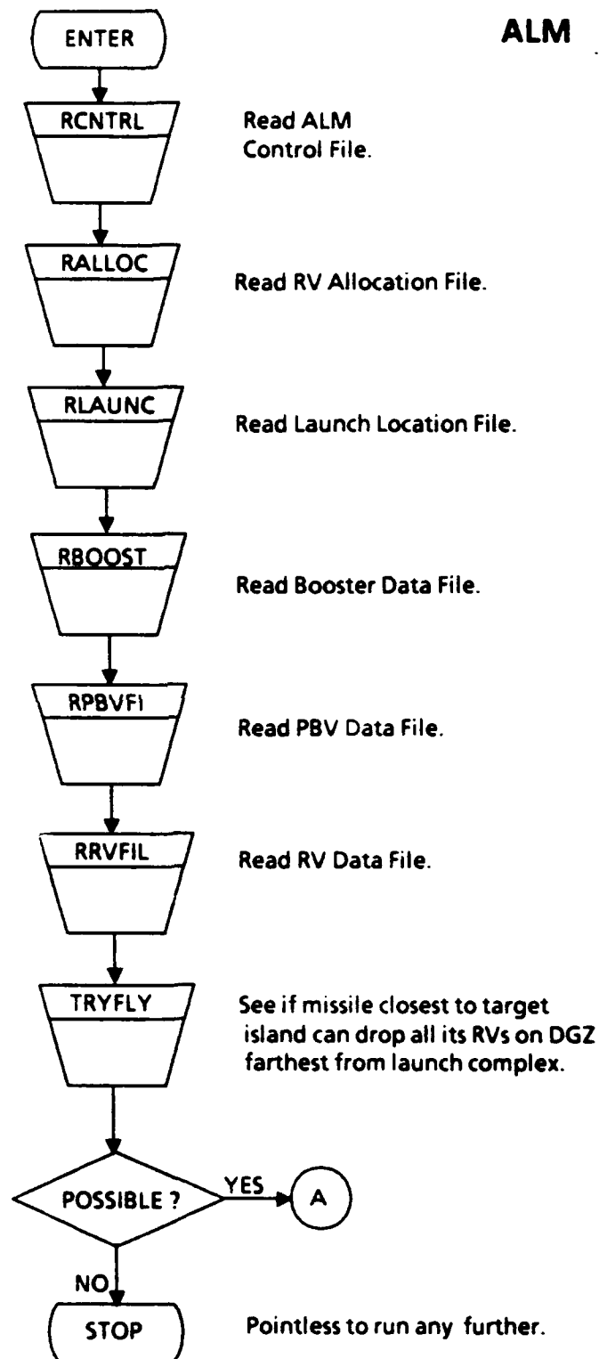
FIGURE 5-1 PROGRAM ALM PROCESS FLOW
