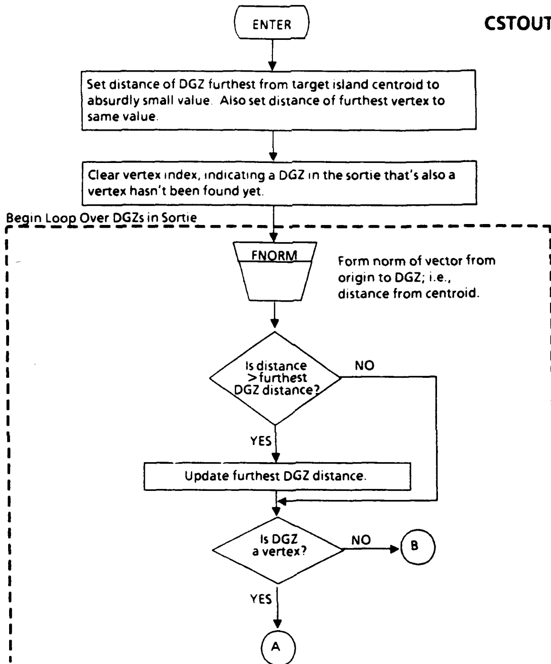
FIGURE 5-11 SUBROUTINE CSTOUT PROCESS FLOW
