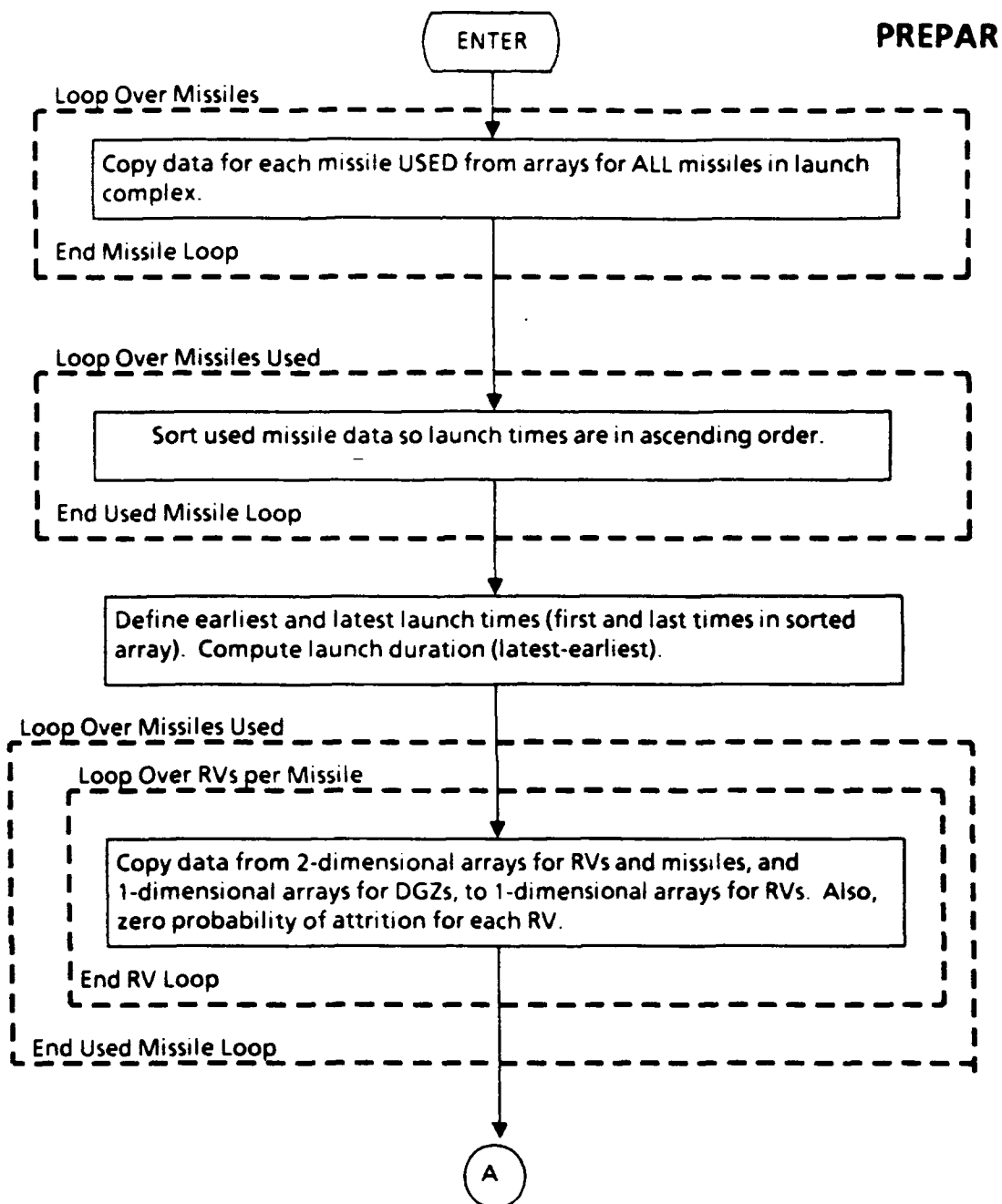
FIGURE 5-4 SUBROUTINE PREPAR PROCESS FLOW
