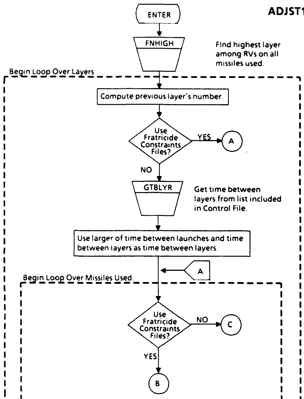
FIGURE 5-7 SUBROUTINE ADJST1 PROCESS FLOW
