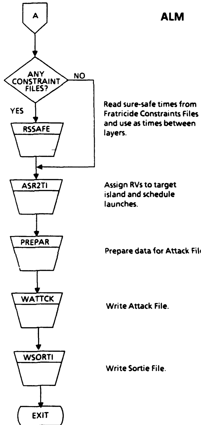
FIGURE 5-1 PROGRAM ALM PROCESS FLOW (Concluded)
