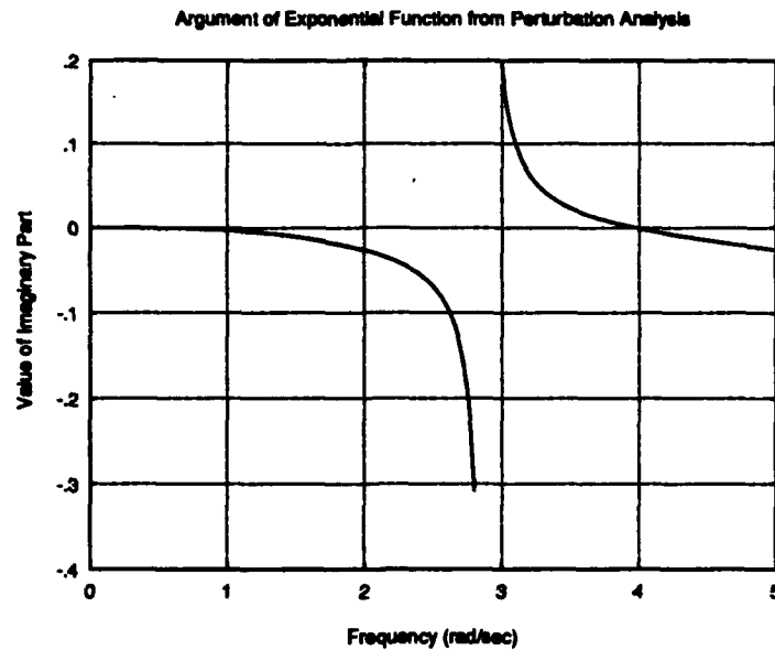
FIGURE 8. IMAGINARY PART OF EXPONENT \alpha FROM PERTURBATION ANALYSIS: IN-PLANE EXCITATION, NORMAL TO CABLE
