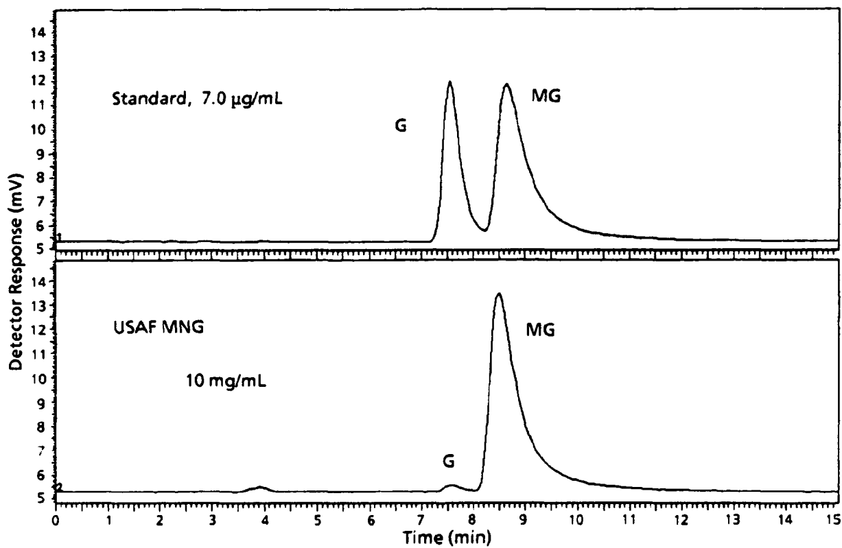
Figure 5. Analysis of Air Force Armament Laboratory MNG by HPLC with Fluorescence Detection. Top panel: Aqueous standards of 7.0 µg/mL G, and MG. Bottom panel: Chromatogram of 10 mg/mL Air Force MNG showing small amounts of G and MG.
