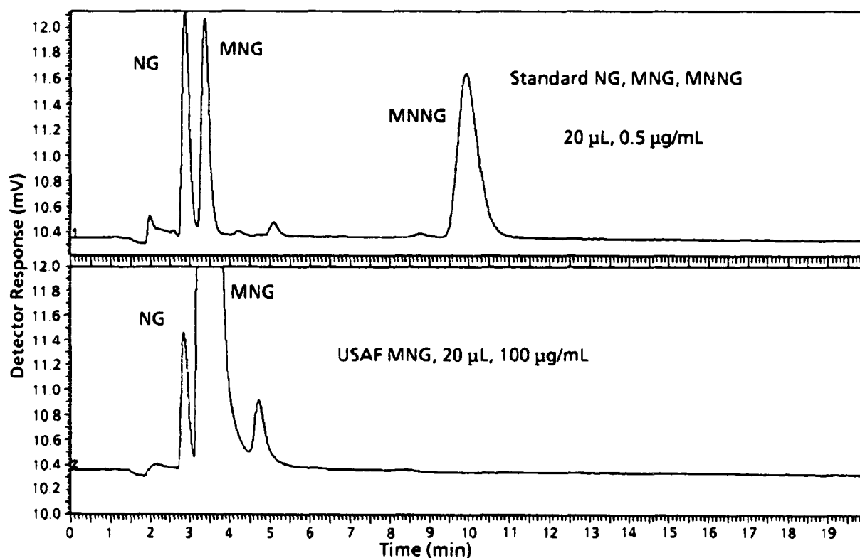
Figure 4. Analysis of Air Force Armament Laboratory MNG by HPLC with UV Detection. Top panel: Aqueous standards of 0.5 μg/mL NG, MNG, and MNNG. Bottom panel: Expanded chromatogram showing small amount of NG in Air Force MNG.
