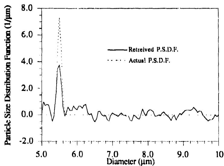
Figure 2. PSDF when the Ref. Index is near the Boundary of the n Space Actual Refractive Index = 1.69 Range of Indices Considered in the Final Inversion 1.68-1.70
