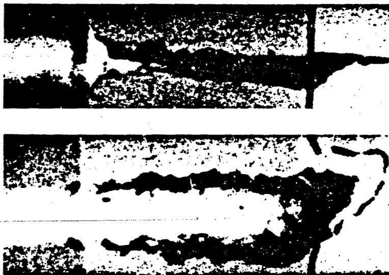
Figure 5. Orthogonal Post-Test Radiographs Showing a Penetration Path Modified by Planar Failure that Resulted From Wave Interactions.
