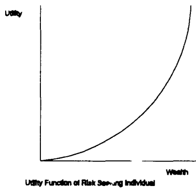
Figure F-3: Risk Attitudes and Utility Functions
