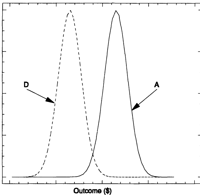
Figure F-7: Stochastic Dominance - PDFs for Alternatives A and D
