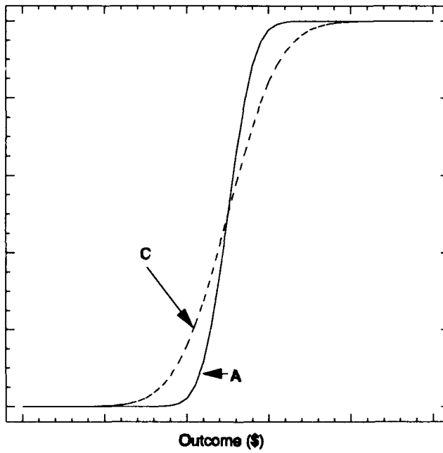
Figure F-10: Stochastic Dominance - CDFs for Alternatives A and C
