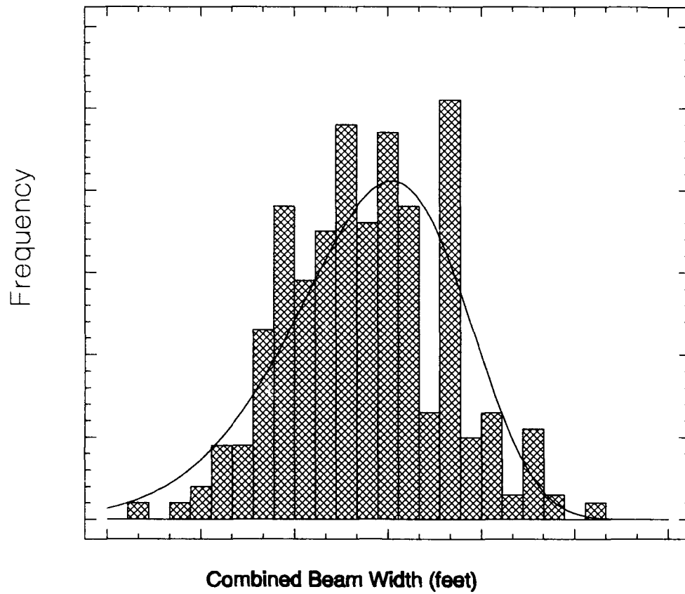
Figure D-9: Weibull Distribution - Superimposed on Data
