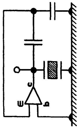
Clapp
