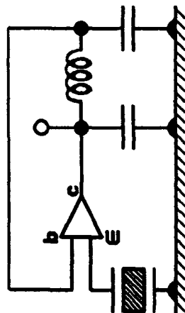
Modified Butler
