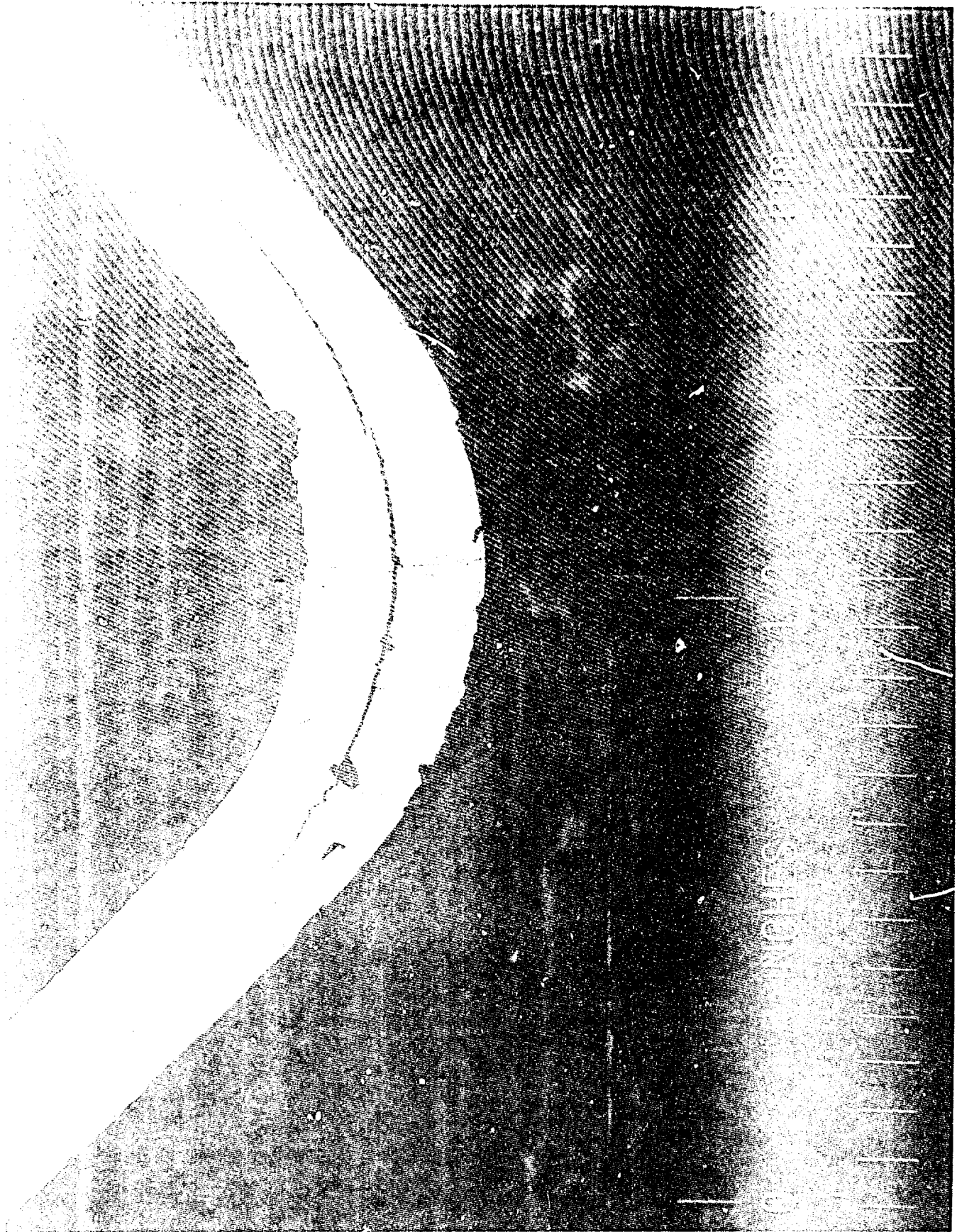
Fig. 8 - Circumferential crack on the edge of a 24-ply specimen with an r_f = 8.5 mm
