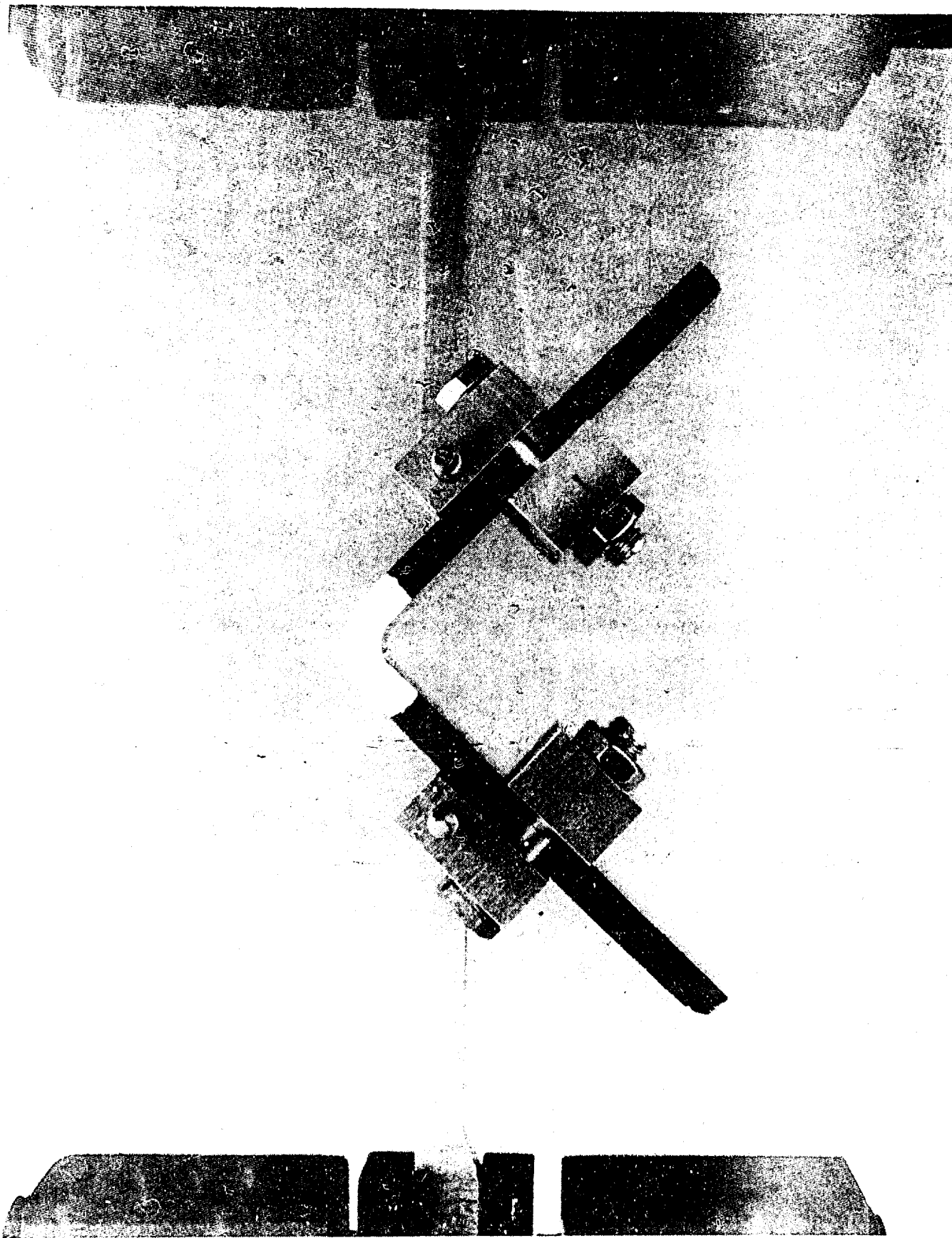
Fig. 2 - Photograph of interlaminae tension strength specimen and test fixture
