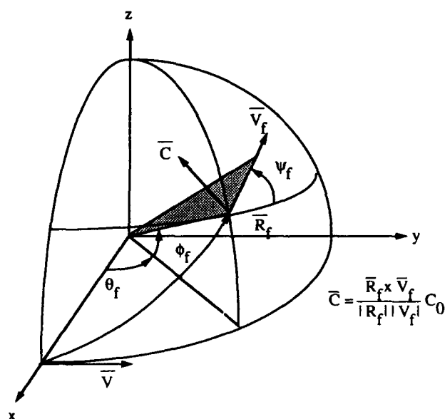
Figure 6. Reformulation of Adjoint Constants
