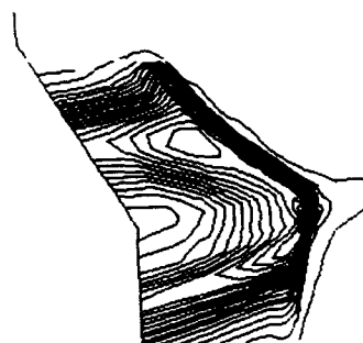
FIGURE 37. - SPANWISE DENSITY CONTOURS, CASE 1.
