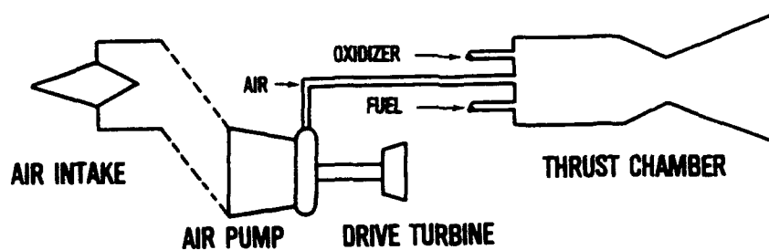
FIGURE 3 CHALLENGE OF PUMPING TO HIGH PRESSURE WITH MINIMUM WEIGHT
