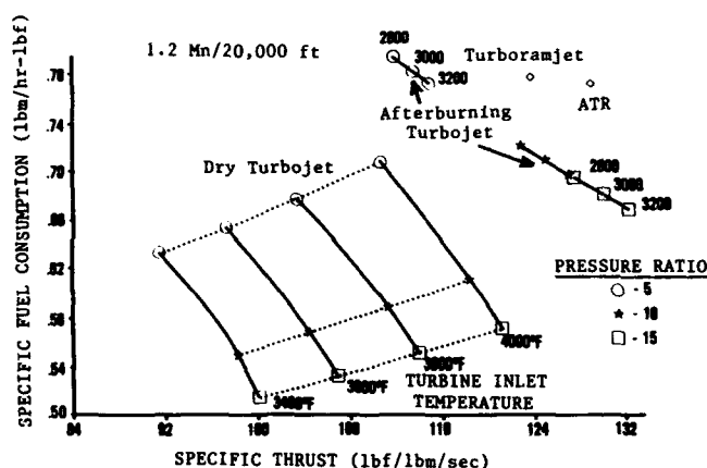
Figure 5 - Transonic Performance Comparison
