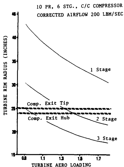
Figure 19 - Turbine Design Tradeoffs
