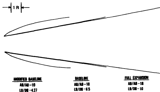
Figure 24 - Nozzle Loss Buildup
