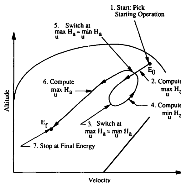
Figure 7. Switching Conditions between Maximum and Minimum Operations
