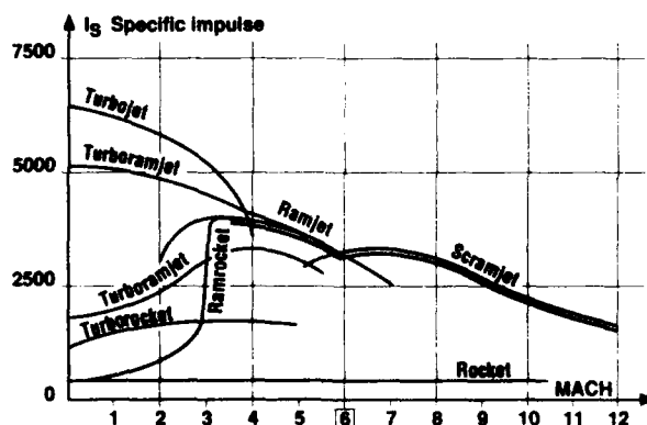
Fig. 17 - Specific impulse with combined engines
