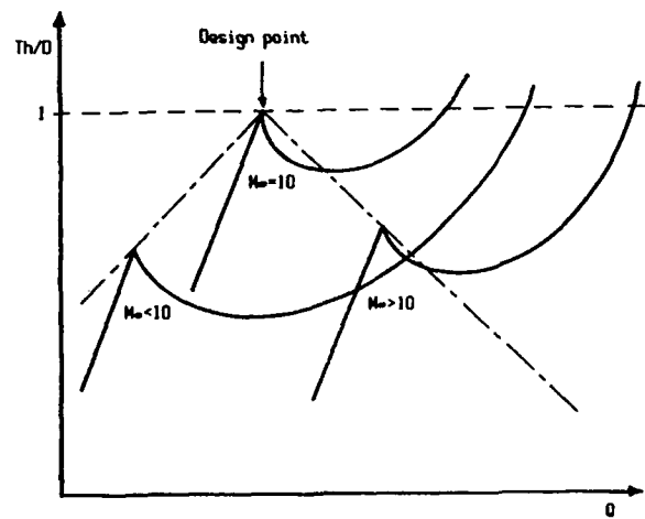
Fig. 20 SKETCH of Th/D vs. Q for Axisymmetric Internal Compression Body
