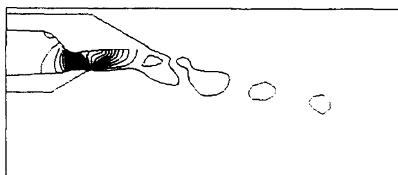
FIGURE 36. - STREAMWISE PRESSURE CONTOURS, CASE 1, i = 1, x = 0.0.
