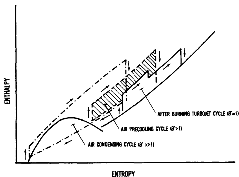
FIGURE 4 THERMODYNAMIC CYCLE SPECTRUM
