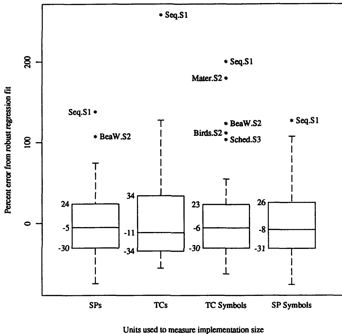
Figure 4-3: Percent error in system size regression, using four measures of system size
