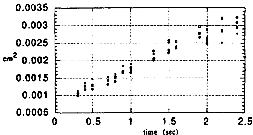
Fig. 5: Spatial extent of the Rb atom cloud as a function of time as it expands into an optical molasses. The different symbols are for different analysis methods.
