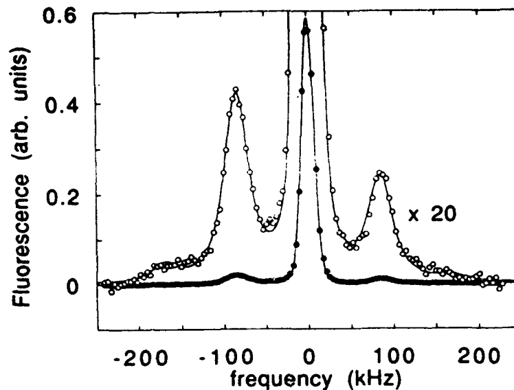
Fig. 8: Spectrum of fluorescence from Rb atoms laser cooled in a 1-D optical molasses with orthogonal linear polarizations in the counterpropagating beams. (From ref. [24].)
