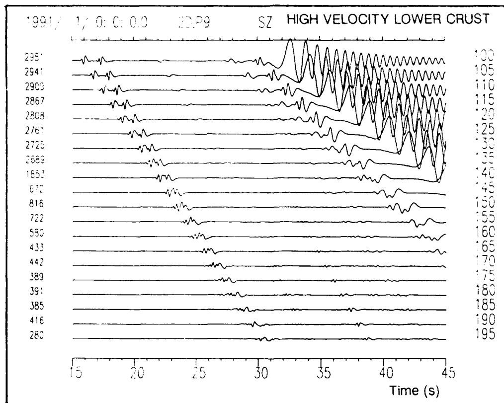
Fig. 3: Comparison between ray tracing and 2D Fd synthetics for a "High Velocity Lower Crust" model taken from Hyndman and Klemperer (1989). For such a simple homogeneous model, the differences between the two sets of synthetic records are small. A peculiar feature in the FD synthetics (Fig. b) is the apparent ringing in the Rayleigh waves apparently caused by the velocity gradients in the upper crust.
