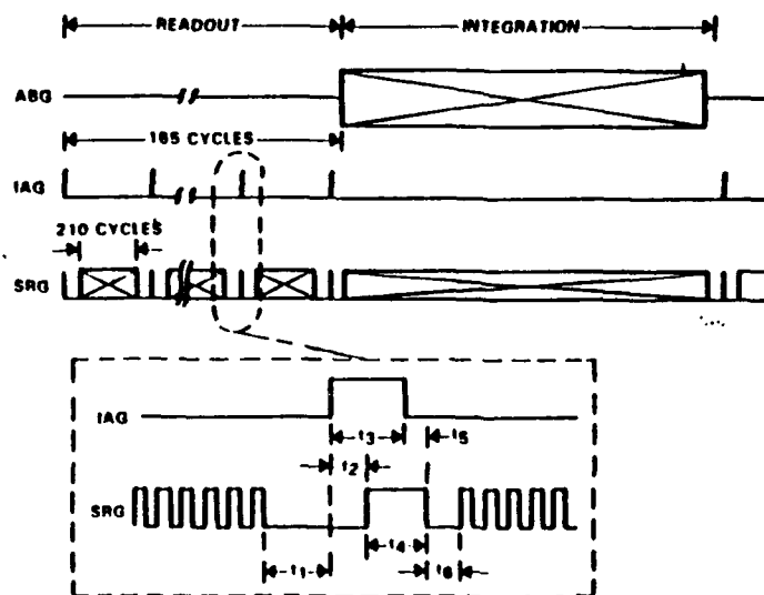
Figure 2. Timing Diagram, NonInterface Mode
