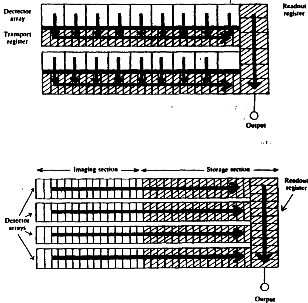
Figure 6. Two schemes for CCD read-out. Top, the interline method; bottom, frame transfer method.
