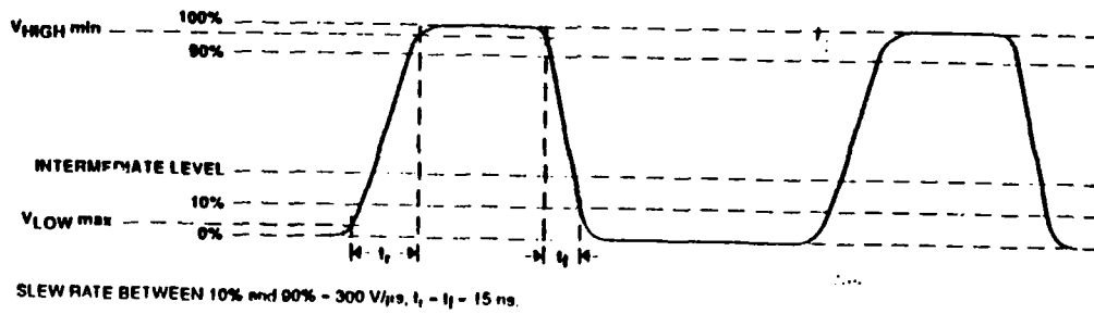
Figure 4. Typical Clock Waveform for SRG
