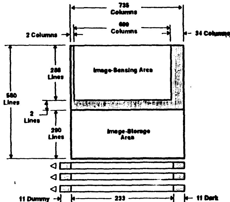
Figure 16. Recommended image sensor CCD, Texas Instruments TC277 block diagram.
