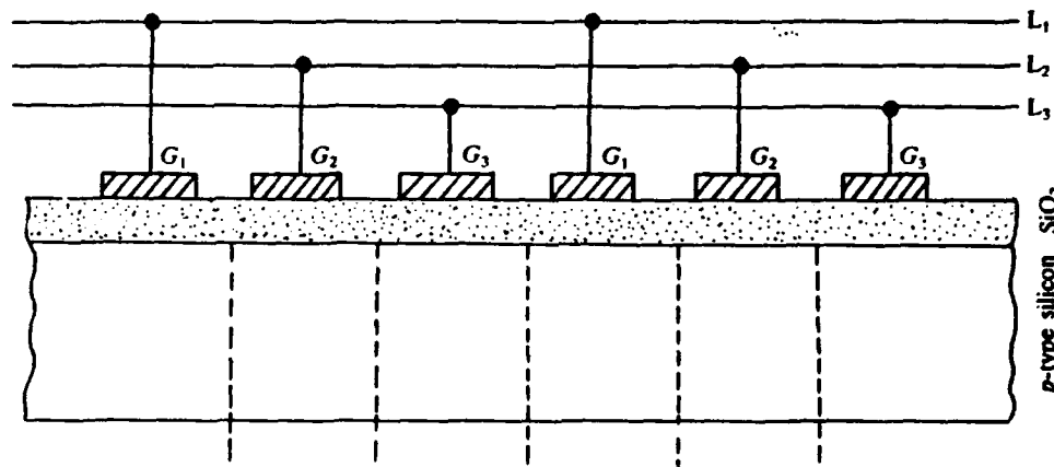
Figure 4. Three pairs of gates (G) are connected with the lines (L) to form three different phases.
