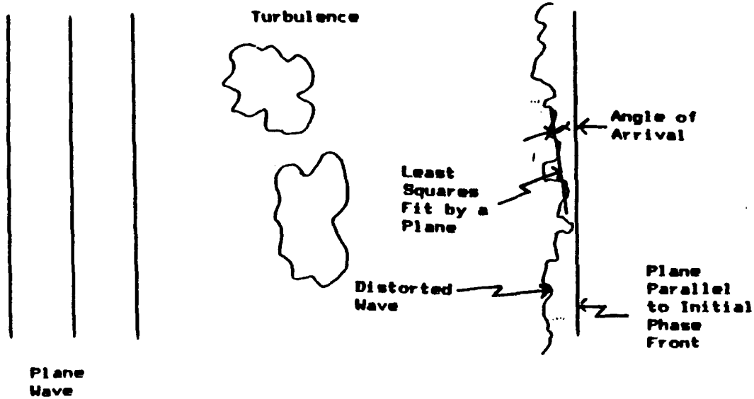
Figure 2. The angle of arrival is the least-squares plane that fits the electric field vector.
