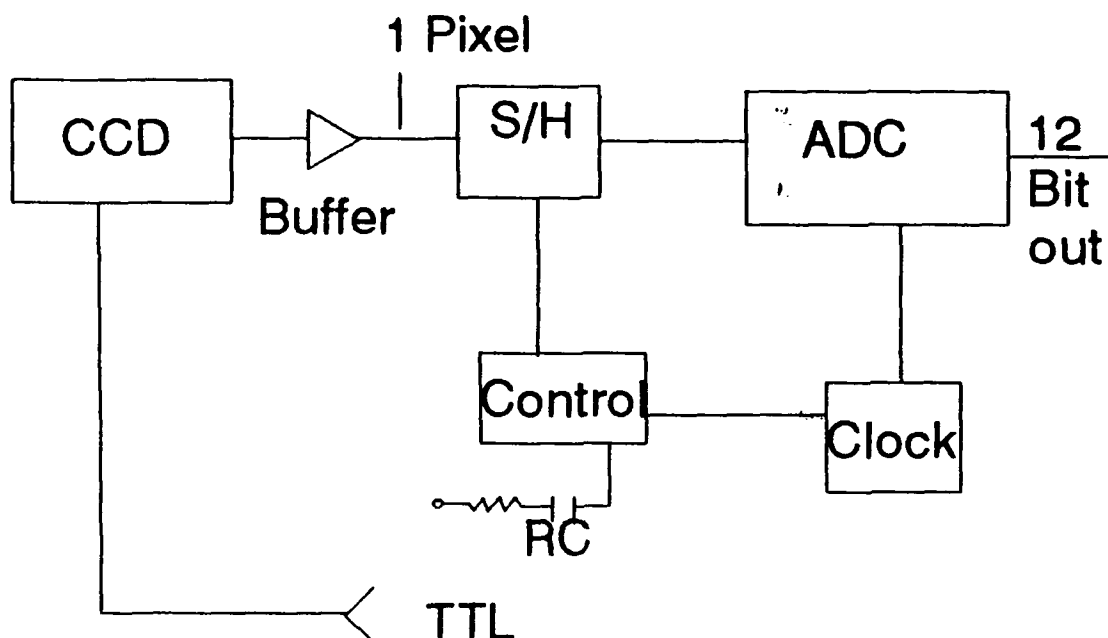
Figure 10. Spectra Sources Lynxx PC+ interface card block diagram.
