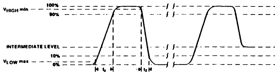
Figure 3. Typical Clock Waveform for IAG and ABG
