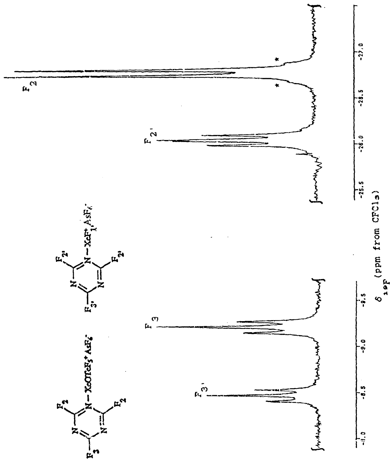
Figure 17. ^{19}\text{F} NMR spectrum (235.361 MHz) of \text{s-C}_6\text{F}_5\text{N}_2\text{N-XeOTeF}_5\text{AsF}_6^- and byproducts of solvolysis in \text{BrF}_5 -55^\circ\text{C} . F-on-C region expansions. Asterisks (*) denote ^{129}\text{Xe} satellites.
