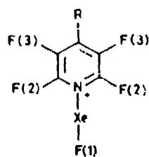
(6): \text{R} = \text{F} (4) or \text{CF}_3
