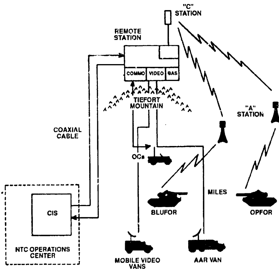
Chart 4 NATIONAL TRAINING CENTER POSITION LOCATION SYSTEM
