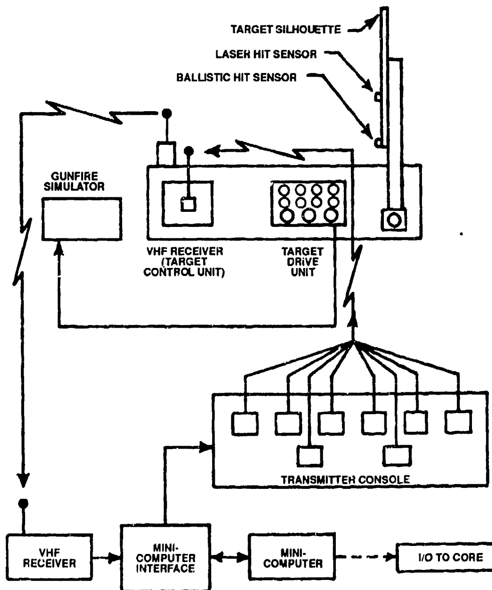
Chart 5 NATIONAL TRAINING CENTER LIVE FIRE SYSTEM RANGE CONTROL UNIT
