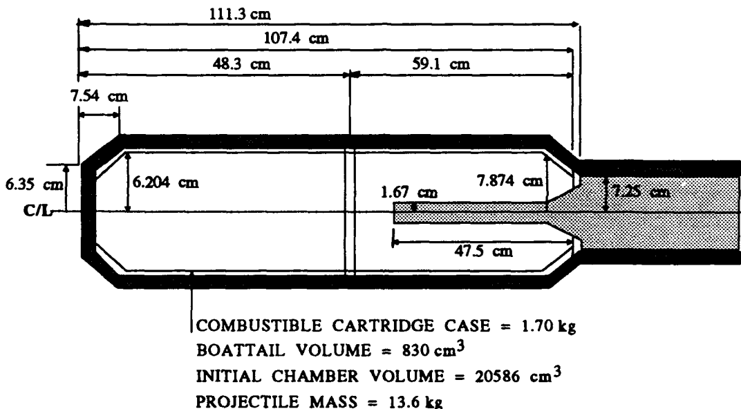
Figure 4. Chamber Dimensions
