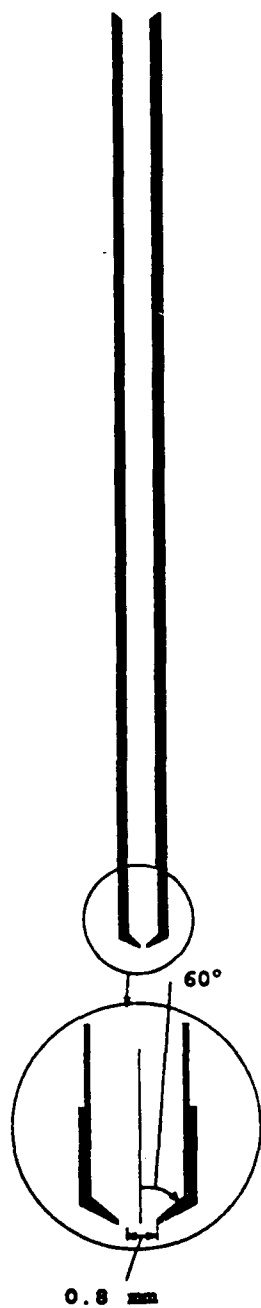
Figure 4.4 Standard 60^\circ Nozzle
