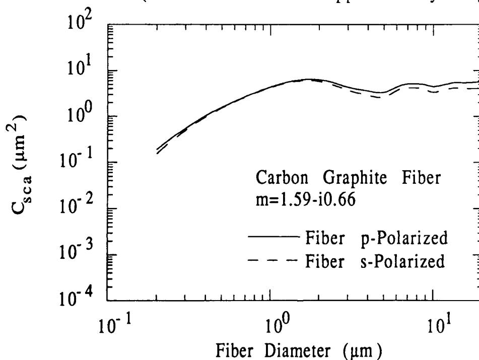
Figure 5.22 Scattering Cross Section ( C_{sca} ) for Carbon Graphite Fibers in a TSI APS (Laser Beam Width is Approximately 30 \mu m )
