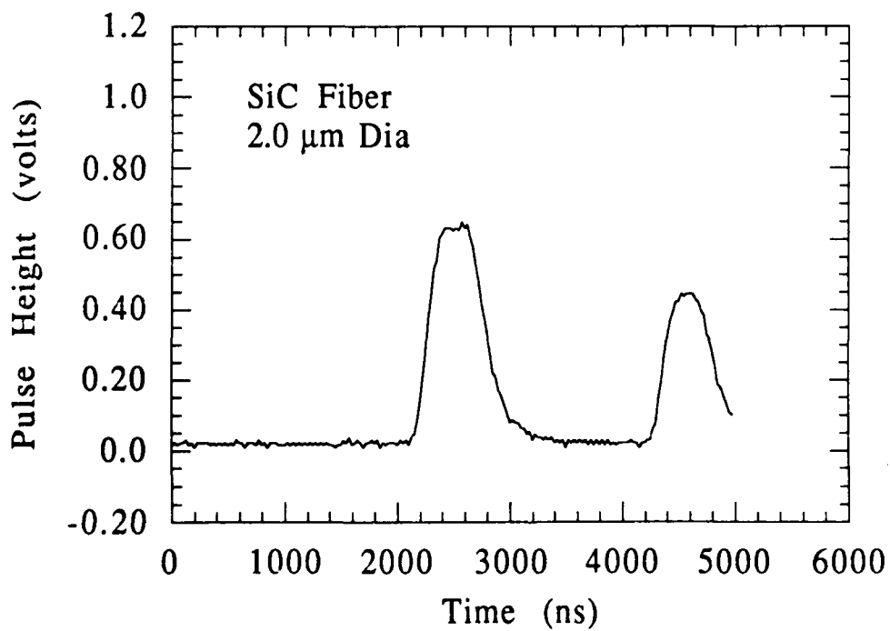
Figure 6.4 APS Pulse from a 2.0 \mu\text{m} SiC Fiber
