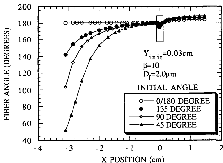
Figure 5.8a Fiber Orientation Through a Modified 2° APS Nozzle for Y_{\text{init}} = 0.03 cm (Nozzle Exit at x = 0 )
