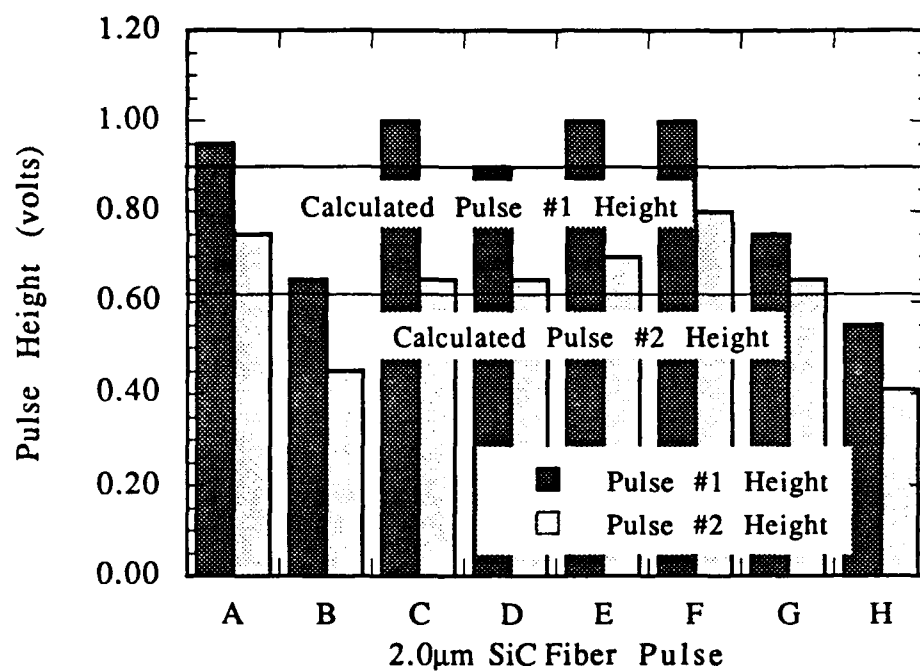
Figure 6.16 Actual Pulse Pair Heights for Several 2.0 \mu m SiC Fiber Pulses
