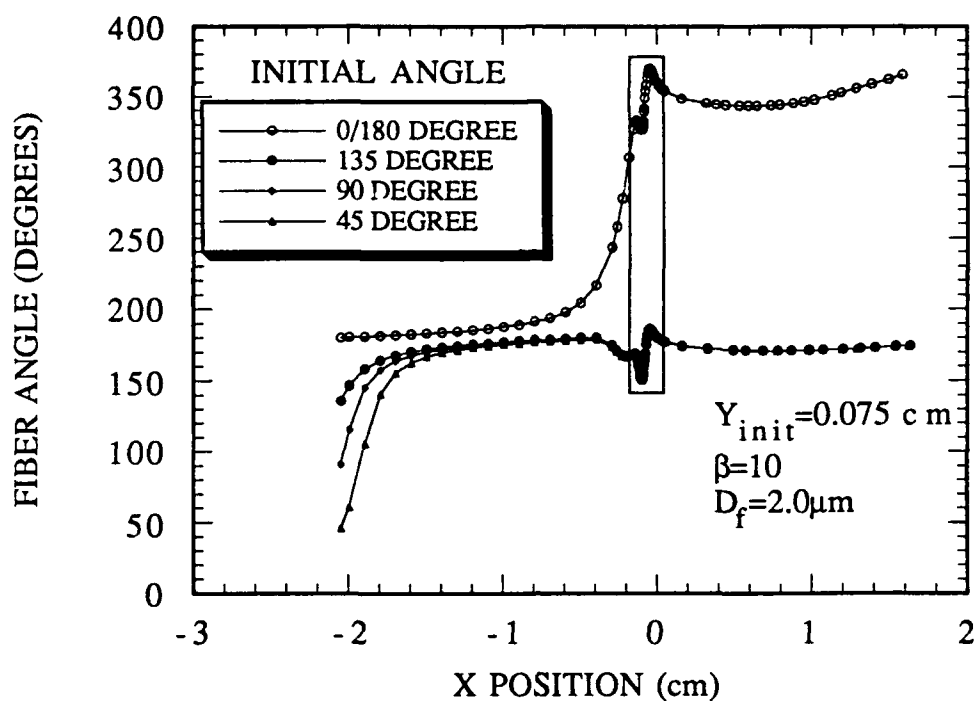
Figure 5.4a Fiber Orientation Through a Standard APS Nozzle for Y_{init}=0.075 cm (Nozzle Exit at x=0 )
