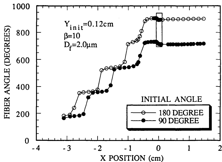
Figure 5.10a Fiber Orientation Through a Modified 2° APS Nozzle for Y_{\text{init}}=0.12\text{ cm} (Nozzle Exit at x=0 )
