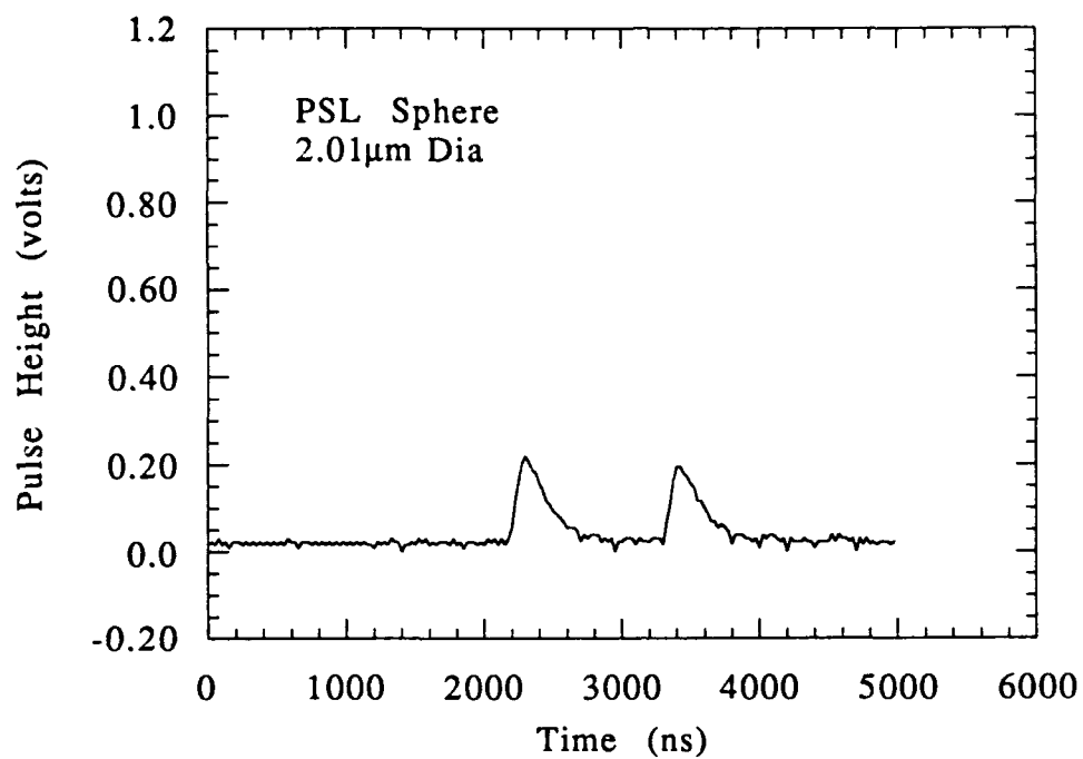
Figure 6.3 APS Pulse from 2.0 \mu\text{m} PSL Sphere
