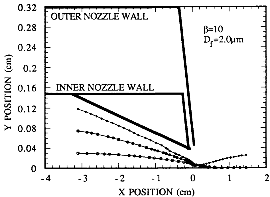
Figure 5.7 Fiber Trajectory in a Modified 2° APS Nozzle (Nozzle Exit at x=0)
