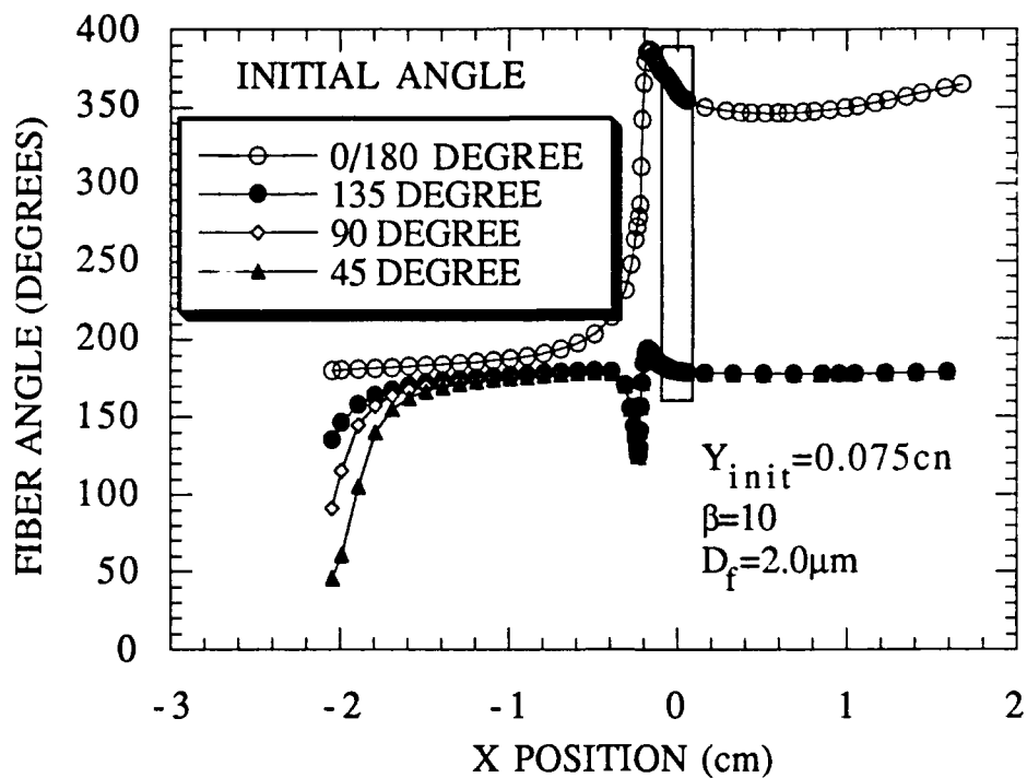
Figure 5.13a Fiber Orientation Through a 90° APS Nozzle for Y_{init}=0.075\text{ cm} (Nozzle Exit at x=0 )
