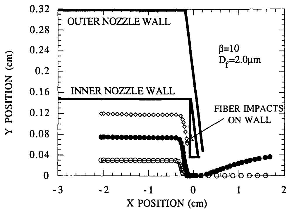
Figure 5.11 Fiber Trajectory in a 90° APS Nozzle (Nozzle Exit at x=0 )
