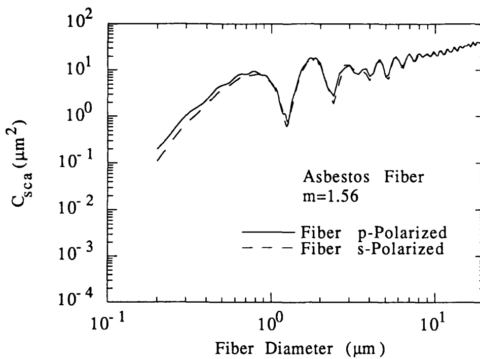
Figure 5.23 Scattering Cross Section ( C_{sca} ) for Asbestos Fibers in a TSI APS (Laser Beam Width Approximately 30 \mu m)
