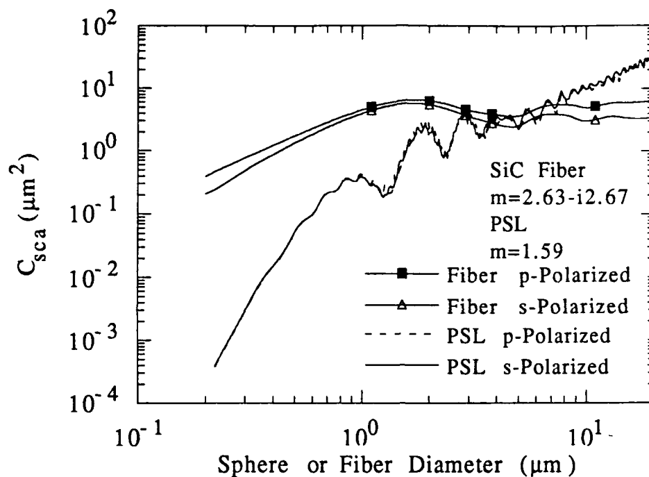
Figure 5.21 Scattering Cross Section ( C_{sca} ) for PSL Spheres and SiC Fibers in a TSI APS (Laser Beam Width is Approximately 30 \mu m )
