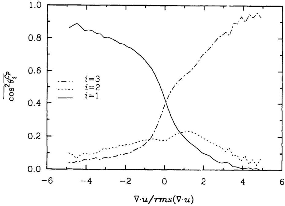
Figure 23: Variation of |\overline{\cos^2 \theta_i^{C\nabla p}}| conditioned on \Theta . M_t = 0.2 , S = 20 , \nu = 1/150 , St = 9 .
