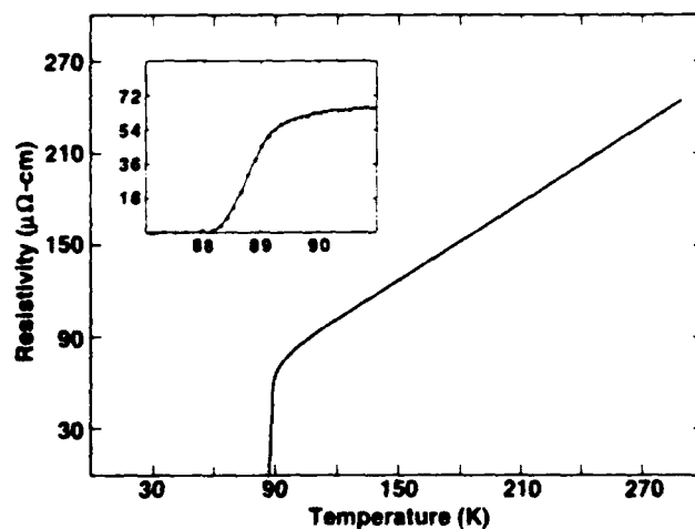
FIG. 1. Resistance vs temperature for a 1300\text{-}\text{\AA} -thick YBCO/YSZ/Si/ \text{Al}_2\text{O}_3 film. The critical current density measured at 77 K is 4.6 \times 10^6 \text{ A/cm}^2 .
