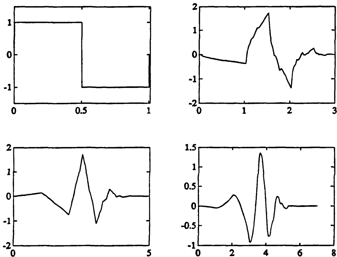
Figure 2.3: Four Examples of Wavelets (clockwise from upper left) "Haar", "Daubechies-2", "Daubechies-4", "Daubechies-3".
