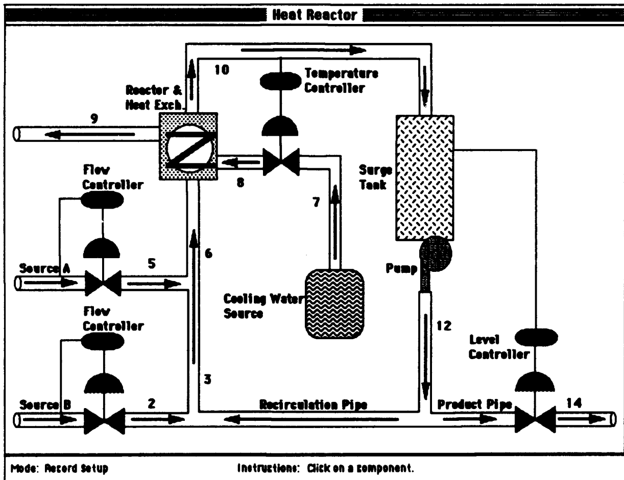
Figure 4. Process Simulation Window
