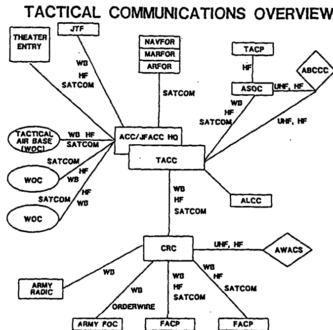
The modes of communication for tactical command and control are provided. SATCOM refers to satellite communications, HF refers to High Frequency comm, and WB refers to tropospheric comm in the UHF/SHF range. Note, in a full blown scenario, two CRCs would normally be deployed under a single TACC.
