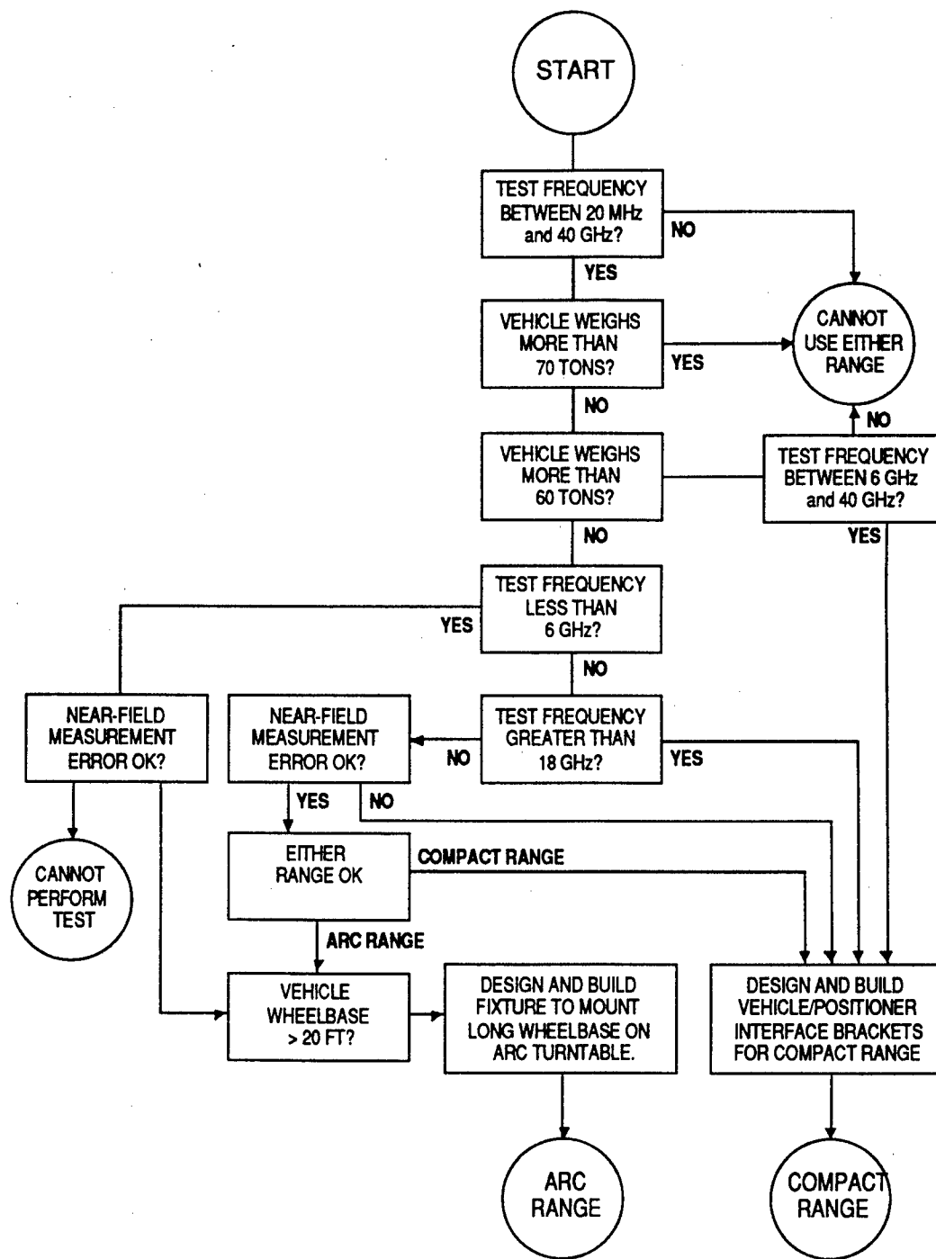
Figure 2. Decision flowchart.
