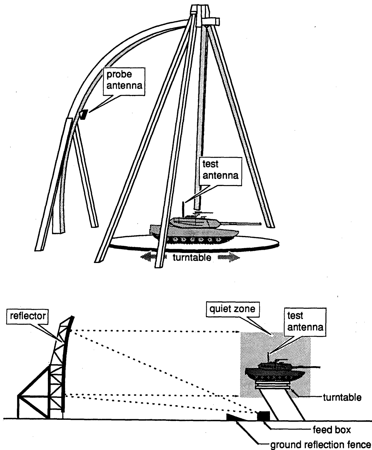
Figure 1. Arc Range (top) and Compact Range (bottom).
