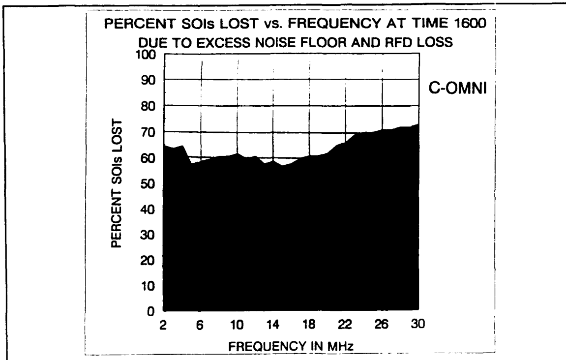
Figure 67. C-OMNI, RFD AND EXCESS NF, 1600.
