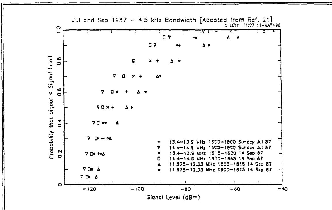
Figure 3.5 - Non-Broadcasting Signal Amplitude Distribution
