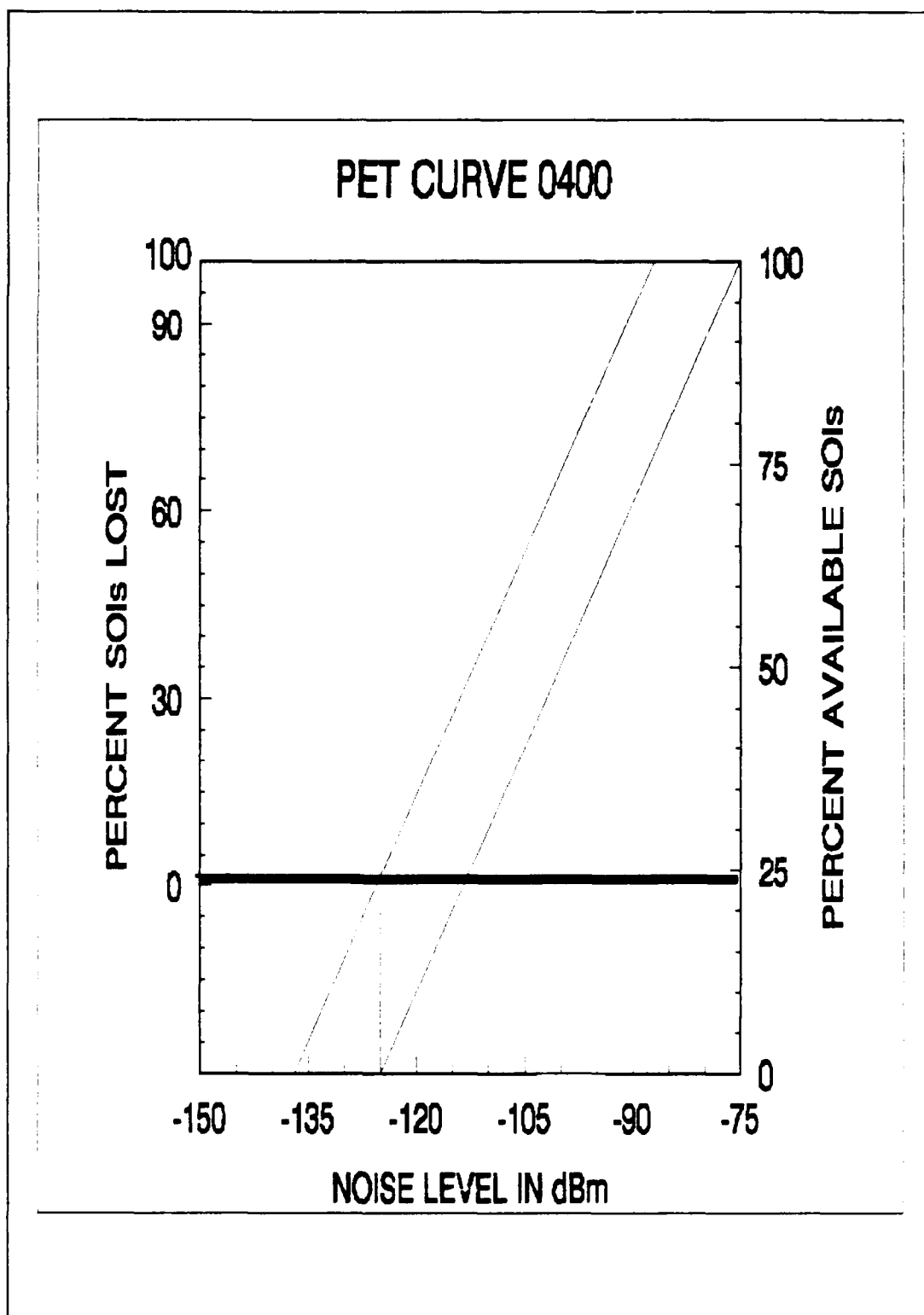
Figure 42. 0400 PET Curve.
