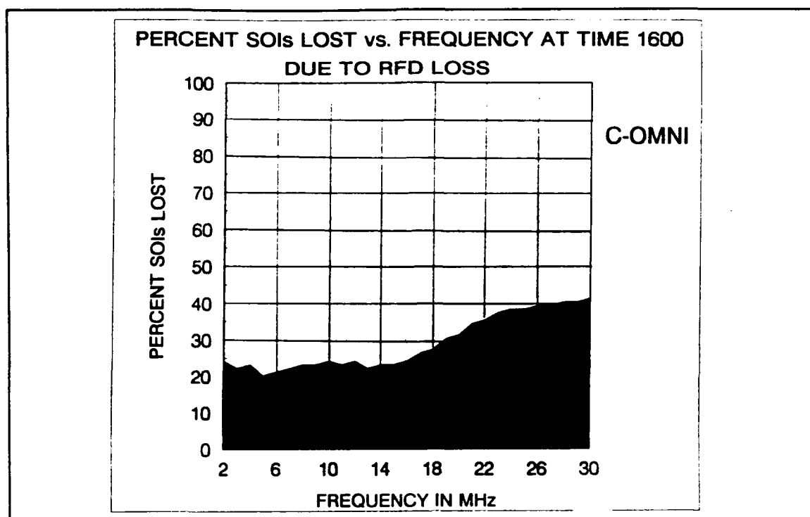
Figure 55. C-OMNI, RFD, 1600.
