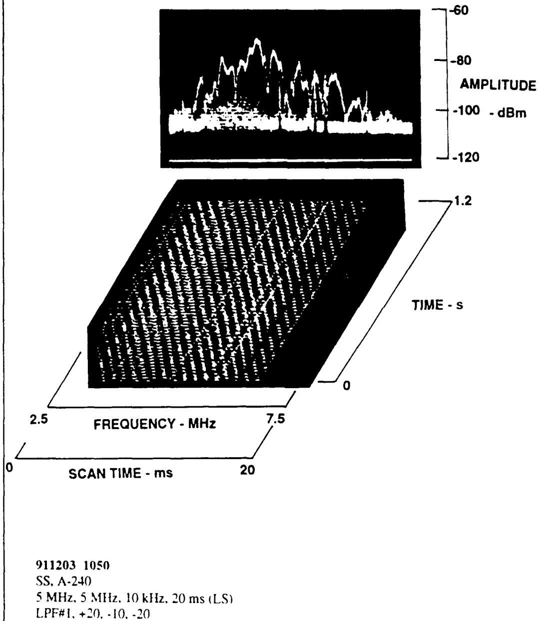
Figure 32. Power-Line Noise.
