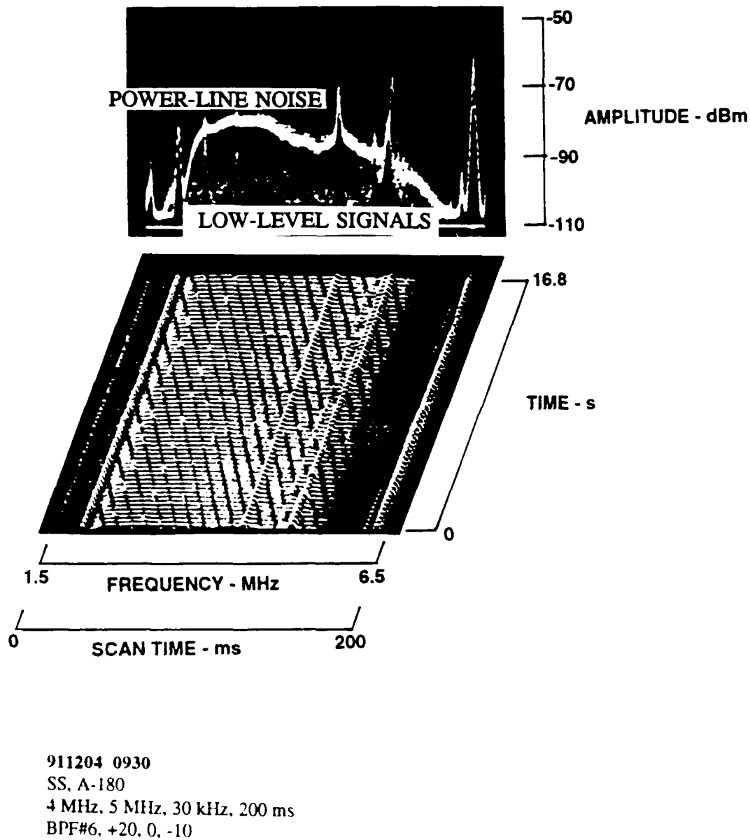
Figure 10. Power Line Noise Hiding Signals.
