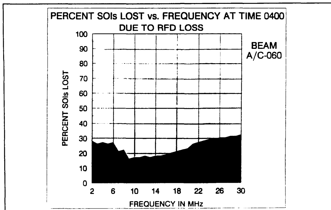
Figure 70. A/C-060, RFD, 0400.
