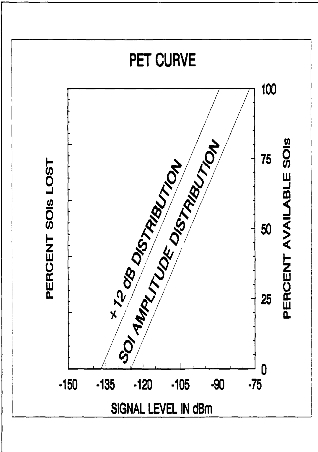
Figure 18. +12 dB Distribution.
