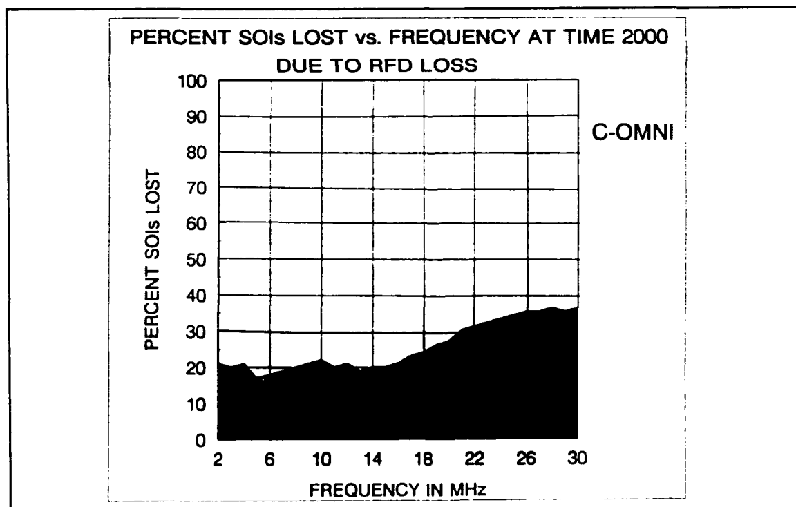
Figure 56. C-OMNI, RFD, 2000.
