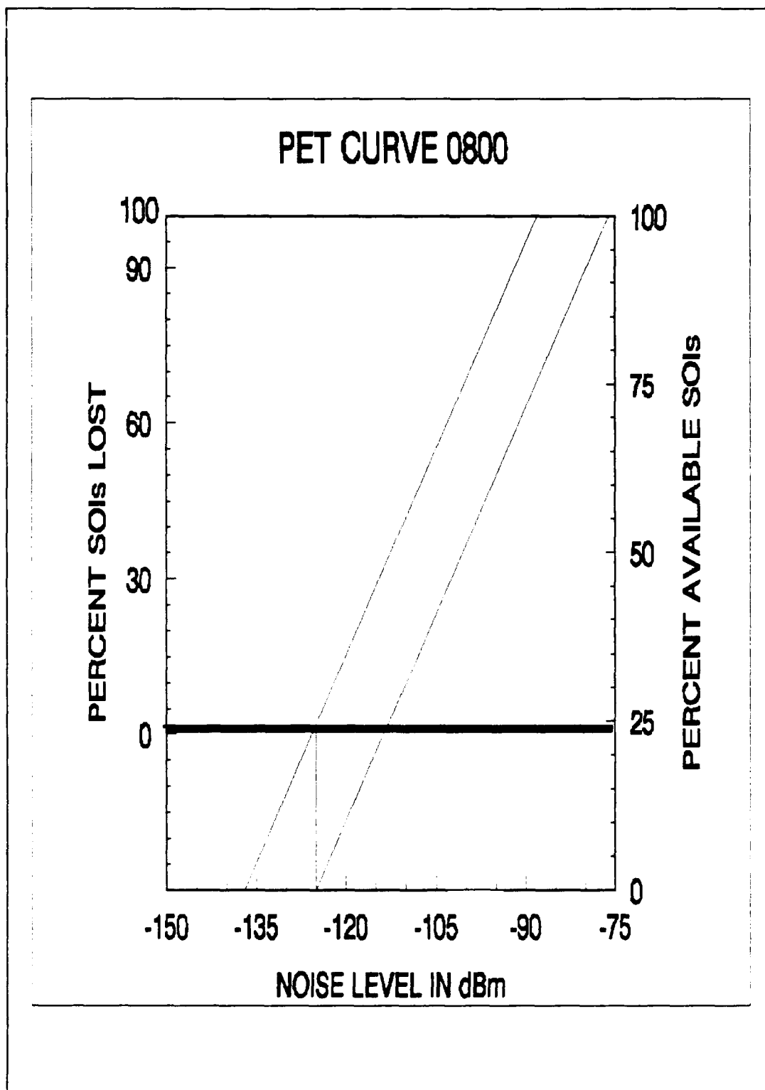
Figure 43. 0800 PET Curve.
