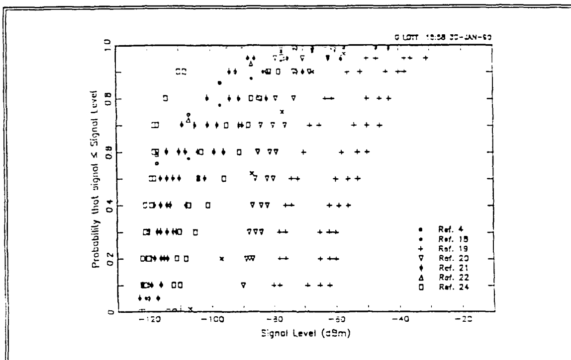
Figure 3.8 - Composite of Non-Broadcasting Signal Amplitude Distributions
