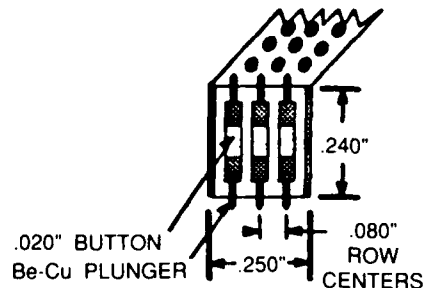
Fig. 17 — Button-based plunger connector. Courtesy of Isi.
