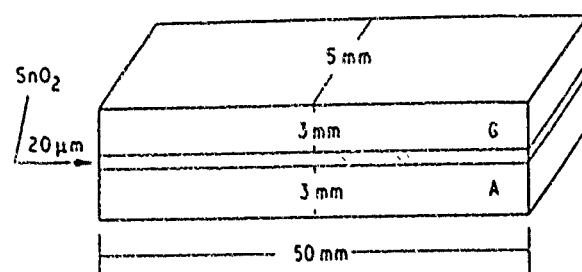
Figure 1 Schematic drawing of a coated composite sample showing the various components. A and G indicate alumina and glass, respectively.
