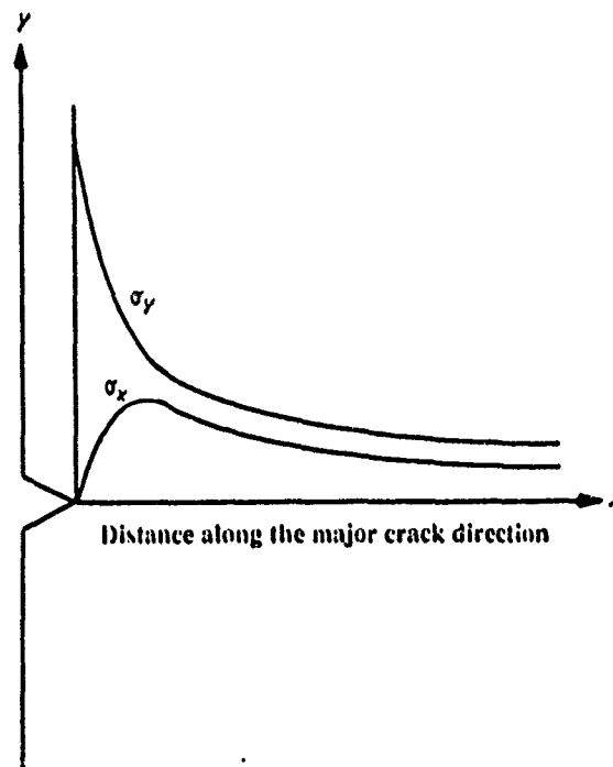
Figure 7 State of stress at a crack tip. Along the x -axis, \sigma_y , although initially high, falls sharply. However, \sigma_x increases from zero at the crack tip and, at a distance roughly equal to one crack tip radius, reaches a maximum value which is about one-fifth of the maximum value of \sigma_y , [15].
