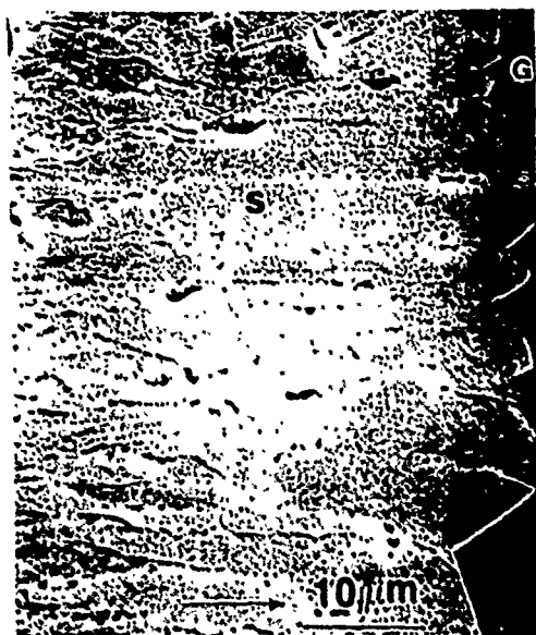
FIG. 9. Etched microstructure of sample 3 (500°C, 150 min). The coating thickness is between 40–45 μm. The columnar \text{SnO}_2 grains are extensively elongated.
