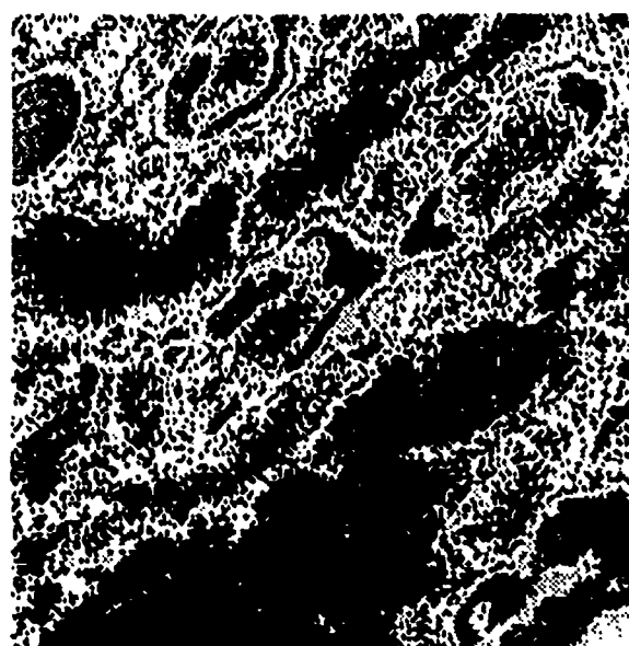
27 Al + Image
