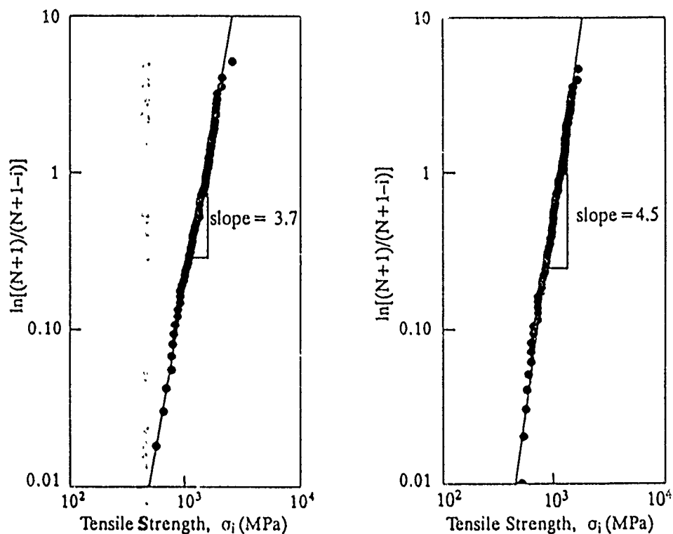
Fig. 1. Weibull plot for a) as-received and b) \text{SnO}_2 coated alumina (PRD-166) fibers.
