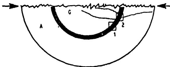
Figure 12 Schematic drawing of a composite disc sample broken under compression. The arrows indicate the compression direction.
