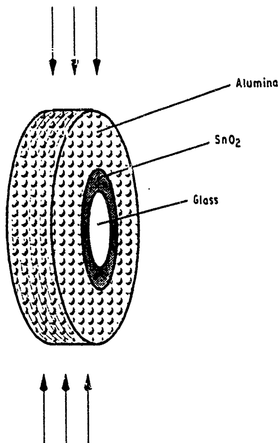
Figure 2 Schematic drawing of a composite disc sample.
