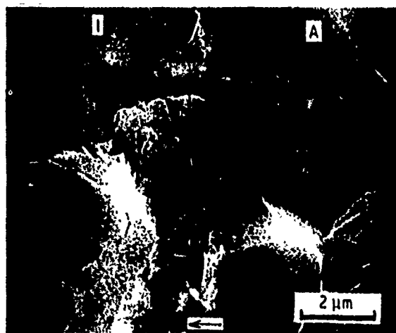
Figure 6 Secondary crack in the \text{SnO}_2 interphase near the \text{SnO}_2/\text{Al}_2\text{O}_3 interface. The fracture surface features are continuous across the crack.
