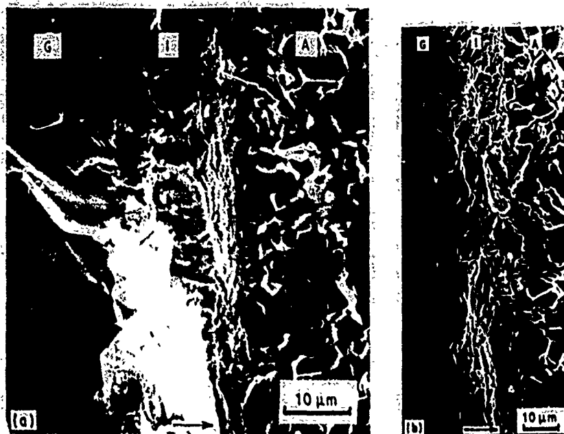
Figure 5 (a) Secondary crack at the \text{SnO}_2/\text{Al}_2\text{O}_3 interface. (b) Secondary crack in the \text{SnO}_2 interphase. The fracture surface features are not continuous across the crack.
