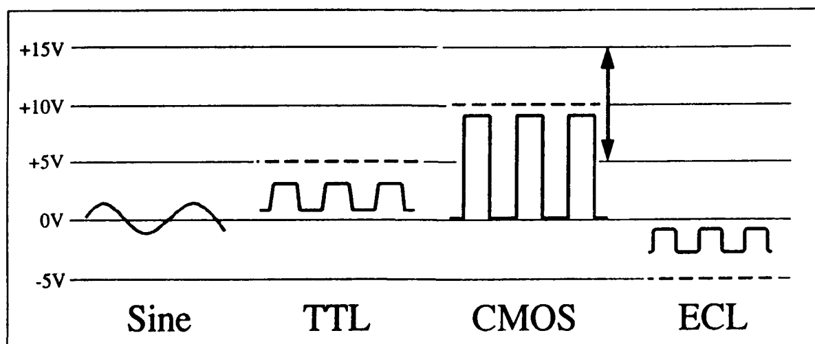
Figure 14. Oscillator outputs.
